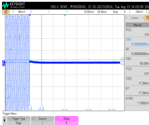
Plot 7.6.1 Transient frequency during power ON test results at low carrier frequency
