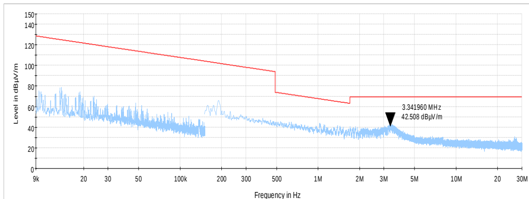
Plot 7.5.2 Radiated emission measurements in 9 kHz - 30 MHz range
