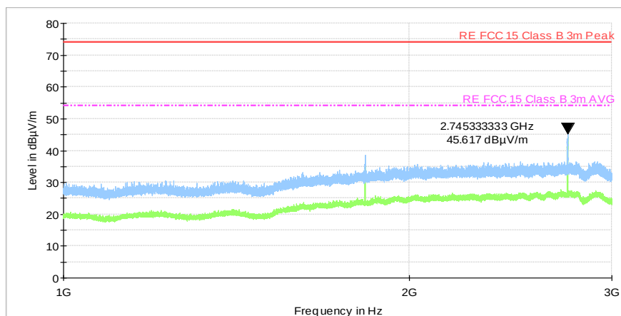
Plot 7.3.18 Radiated emission measurements from 1000 to 3000 MHz at the high carrier frequency
