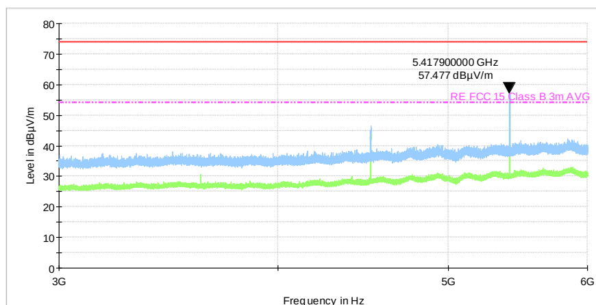
Plot 7.3.20 Radiated emission measurements from 3000 to 6000 MHz at the mid carrier frequency
