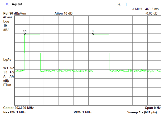
Plot 7.7.20 Transmission pulse period
