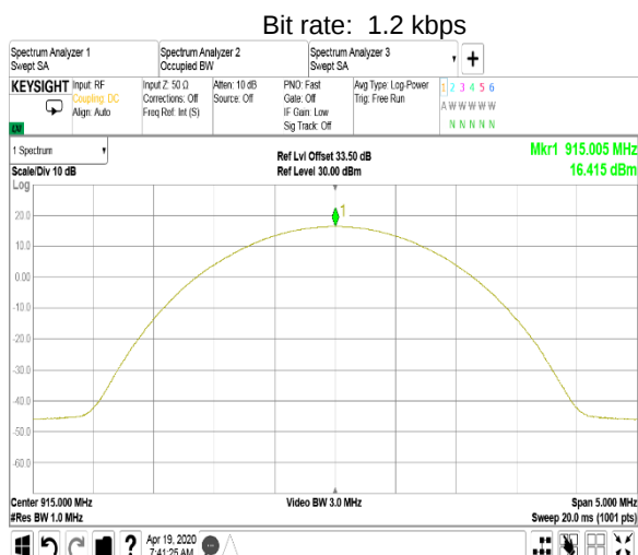
Plot 7.5.2 Peak output power at mid frequency
