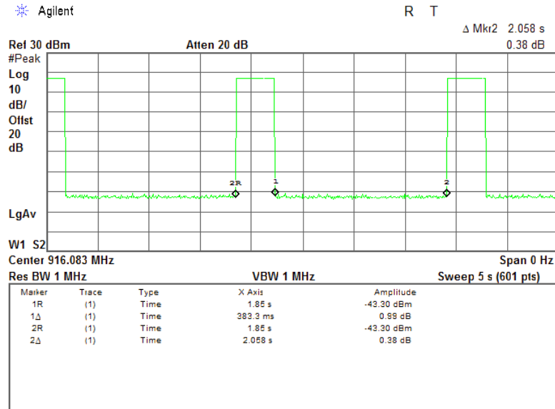
Plot 7.5.10 Transmission pulse duration and pulse period
