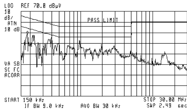
Plot 7.9.2 Conducted emission measurements
