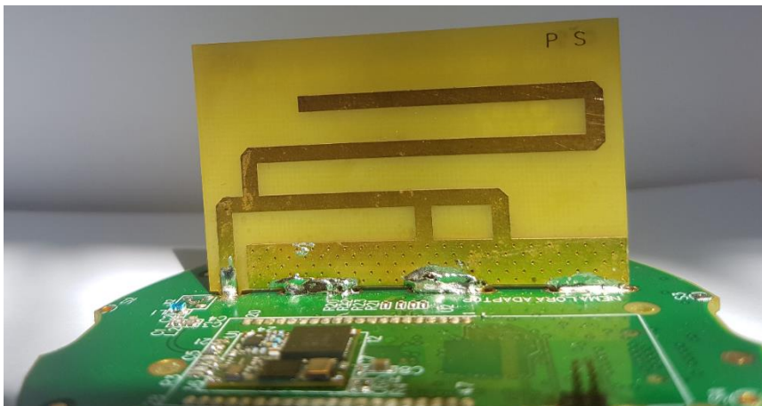
Photograph 7.10.1 Antenna assembly
