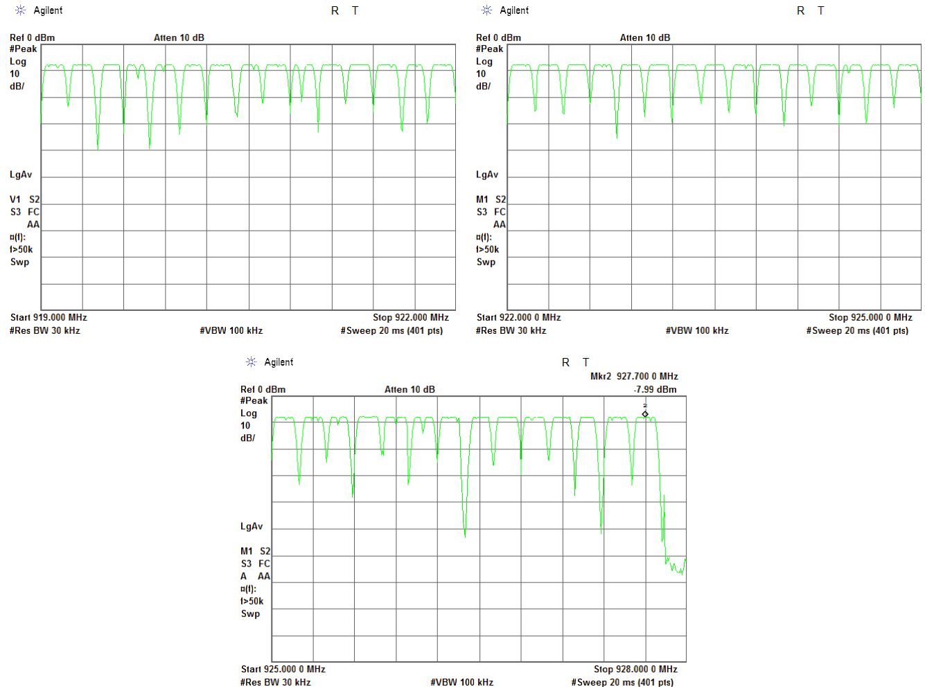
Plot 7.3.2 Number of hopping frequencies
