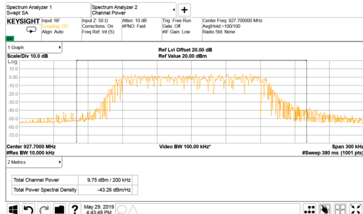
Plot 7.5.6 Peak output power at high frequency and 115%Unom
