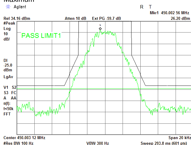
Plot 7.3.2 Emission mask test results at mid carrier frequency
