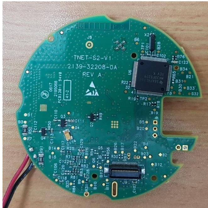
TNET S2 V1 (RF card) - bottom view
