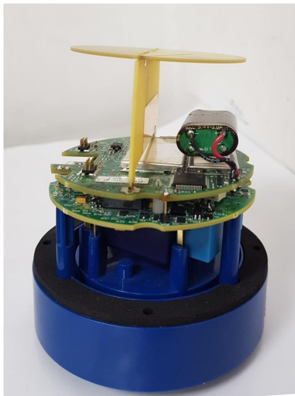
Full integration with antenna
