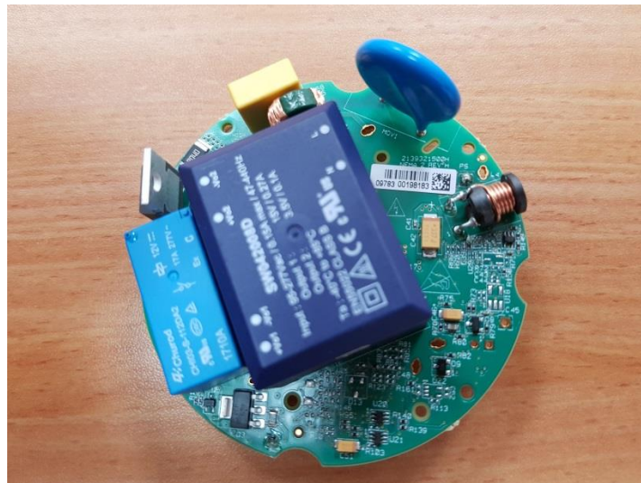
NEMA2 card-Bottom view
