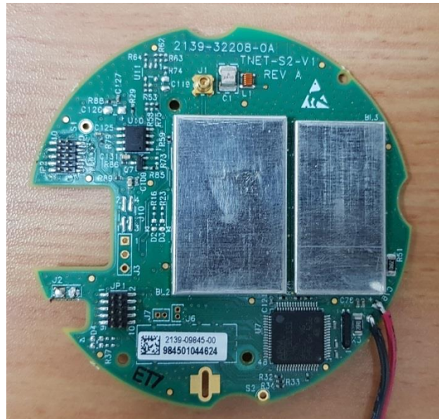
TNET S2 V1 (RF card) with shields- top view
