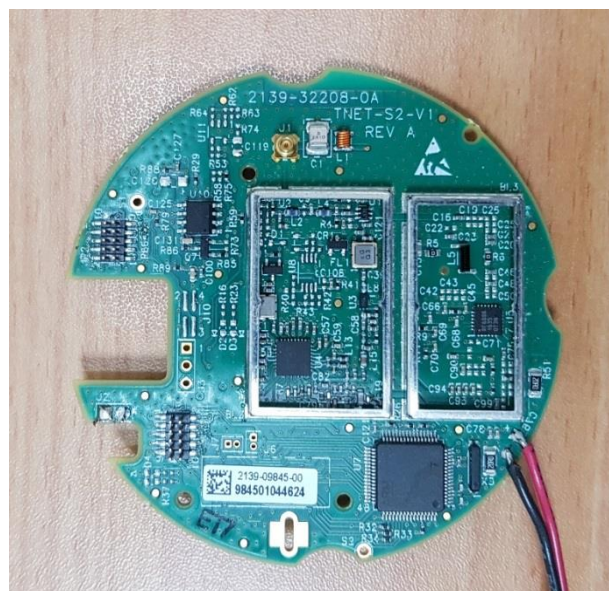
TNET S2 V1 (RF card) shields removed- top view
