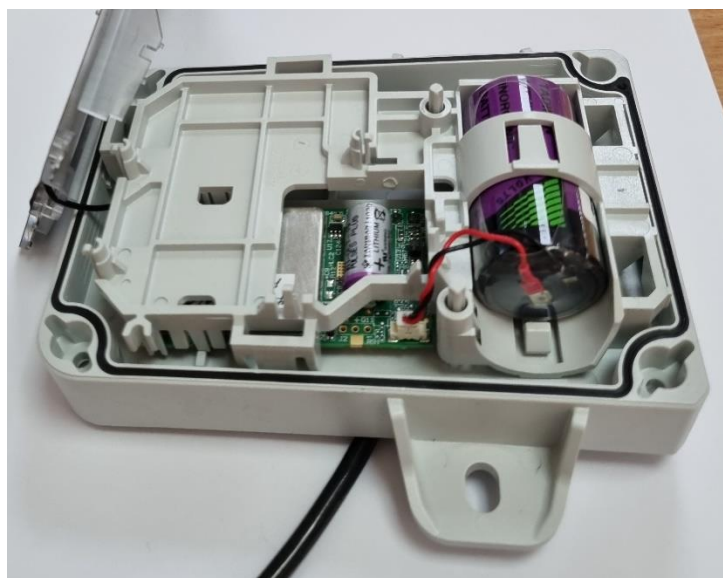
Assembly – RF card and Battery
