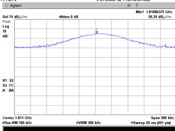
Plot 7.3.27 Radiated emission measurements at the second harmonic of mid carrier frequency
