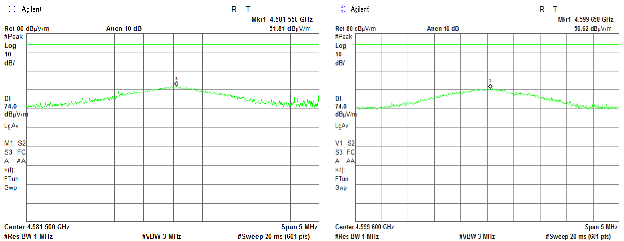
Plot 7.3.37 Radiated emission measurements at the fifth harmonic of high carrier frequency
