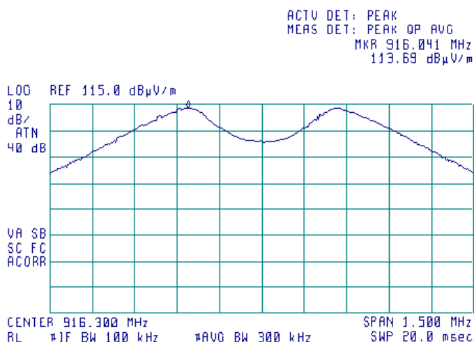
Plot 7.5.4 Peak spectral power density, FSK modulation
