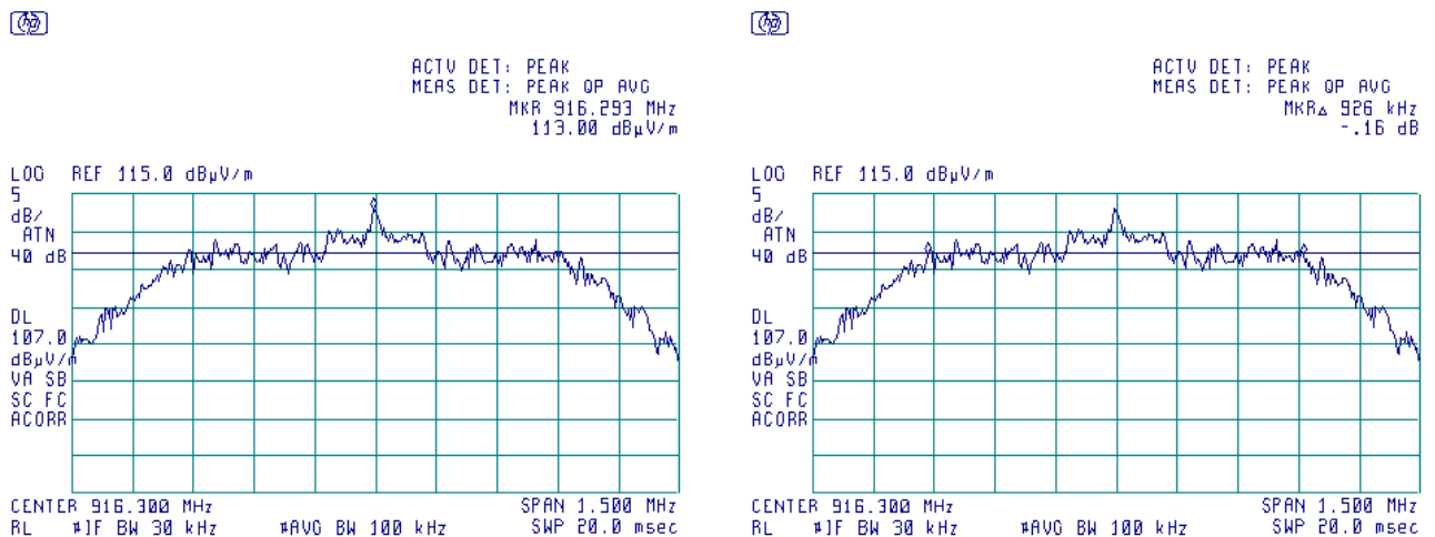
Plot 7.1.2 The 6 dB bandwidth test result at mid frequency, BPSK modulation
