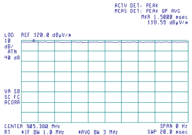
Plot 7.2.2 Field strength of carrier at mid frequency, BPSK modulation
