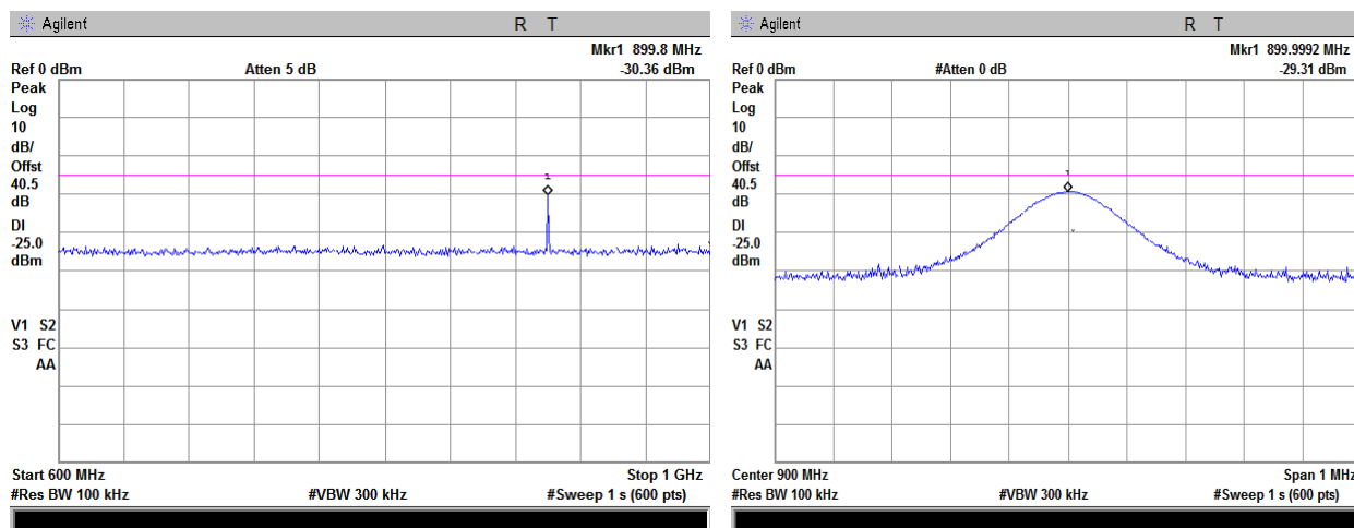
Plot 7.5.5 Spurious emission measurements in 600 - 1000 MHz range at low carrier frequency
