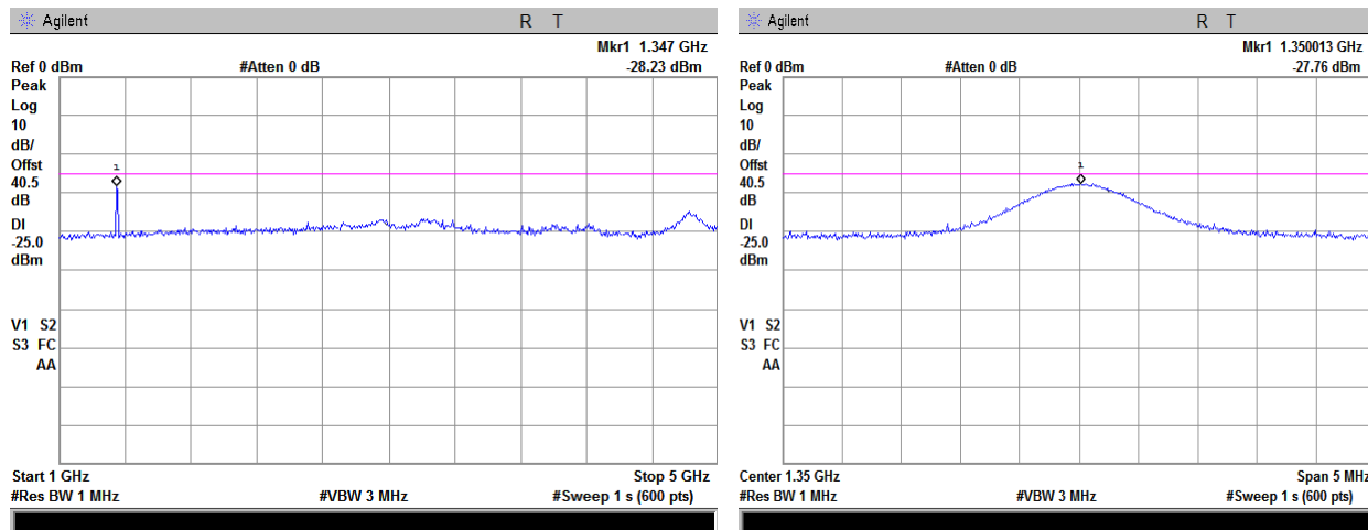
Plot 7.5.6 Spurious emission measurements in 1000 – 5000 MHz at low carrier frequency
