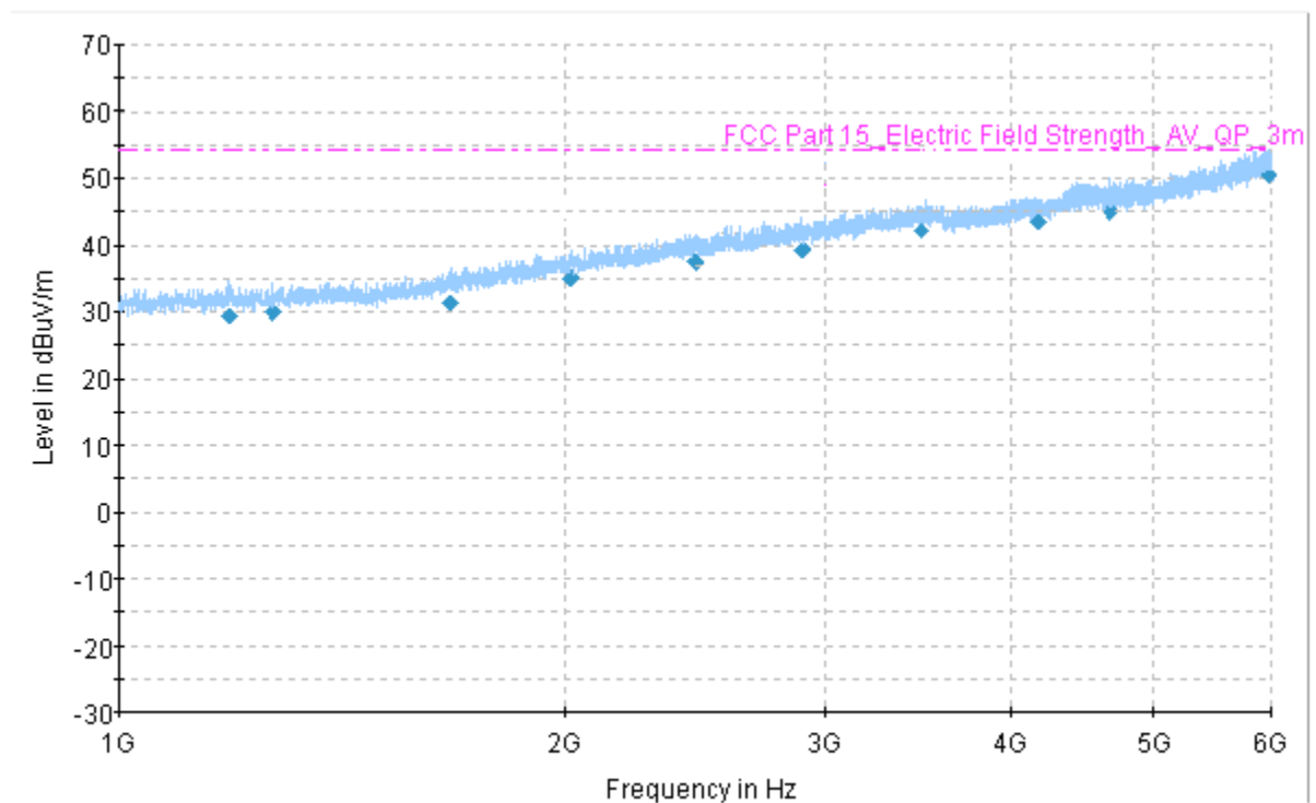
Plot 3.8.2 Radiated emission measurements in (1000 – 6000) MHz range, vertical and horizontal polarization (450 MHz)
