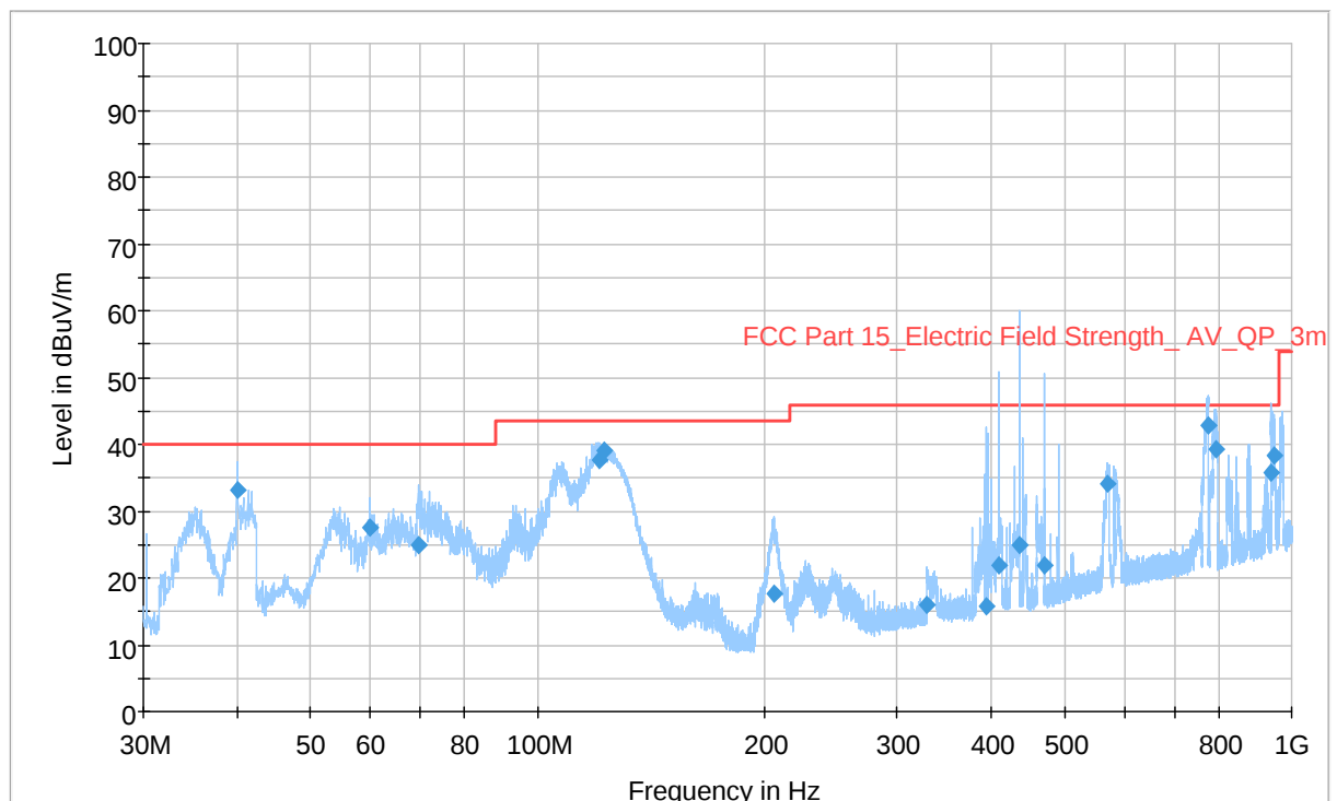
Plot 3.8.1 Radiated emission measurements in (30 – 1000) MHz range, vertical and horizontal polarization (450 MHz)
