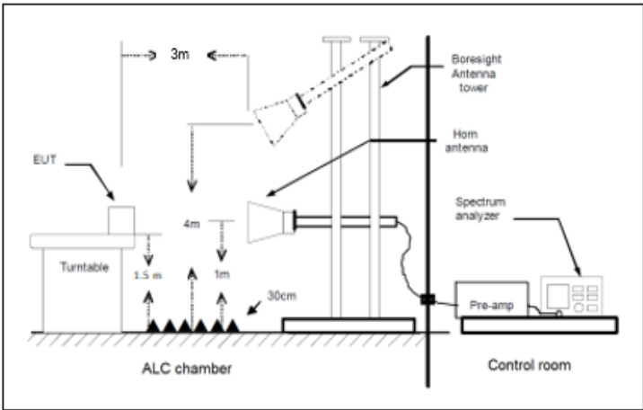
Radiated measurements setup f > 18\text{ GHz}
