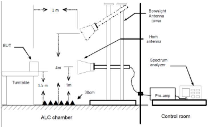
Radiated measurements setup f > 18\text{ GHz}
