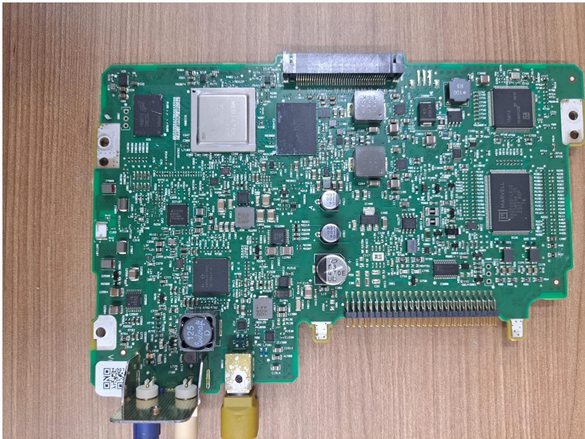
Main board
