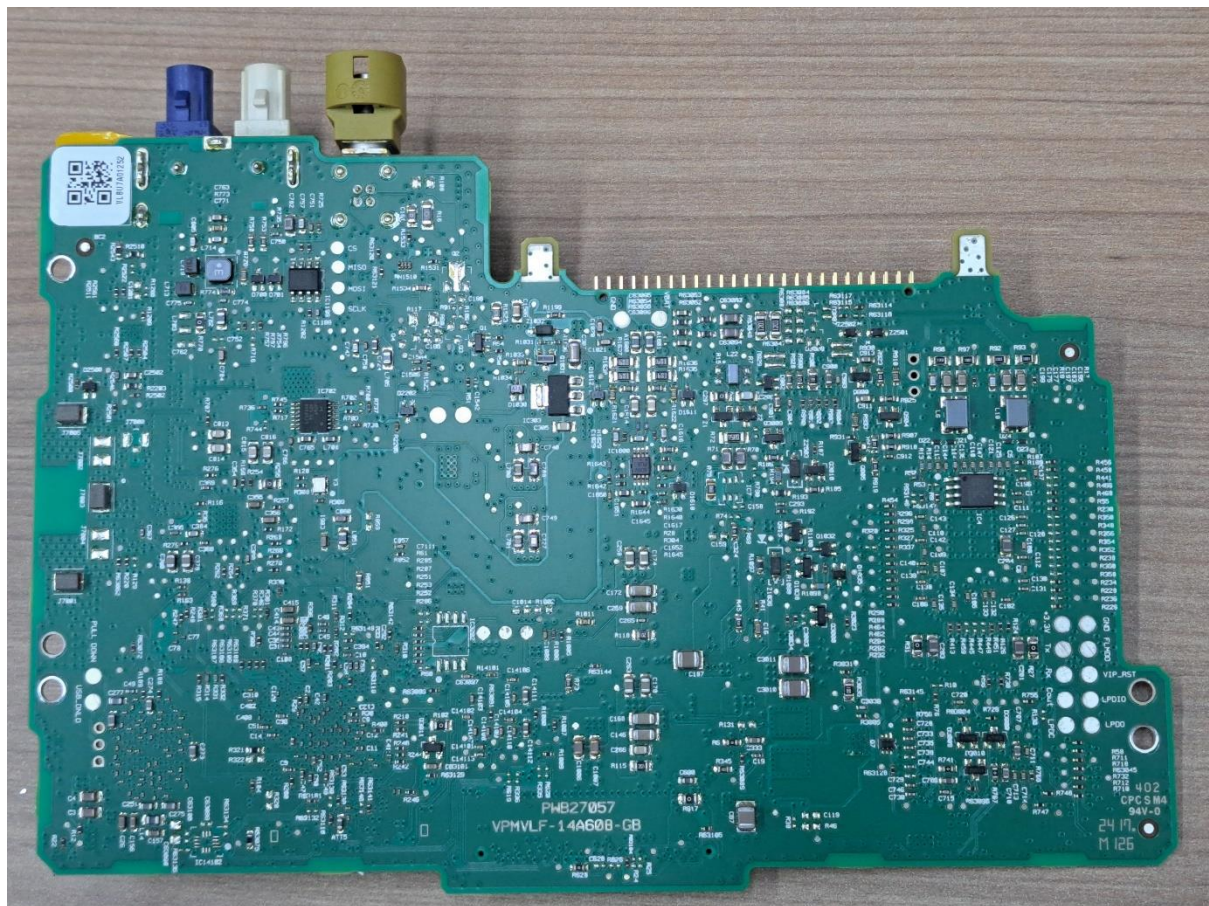
Front Board
