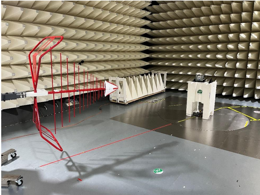
4. Radiated Emission test setup 1
