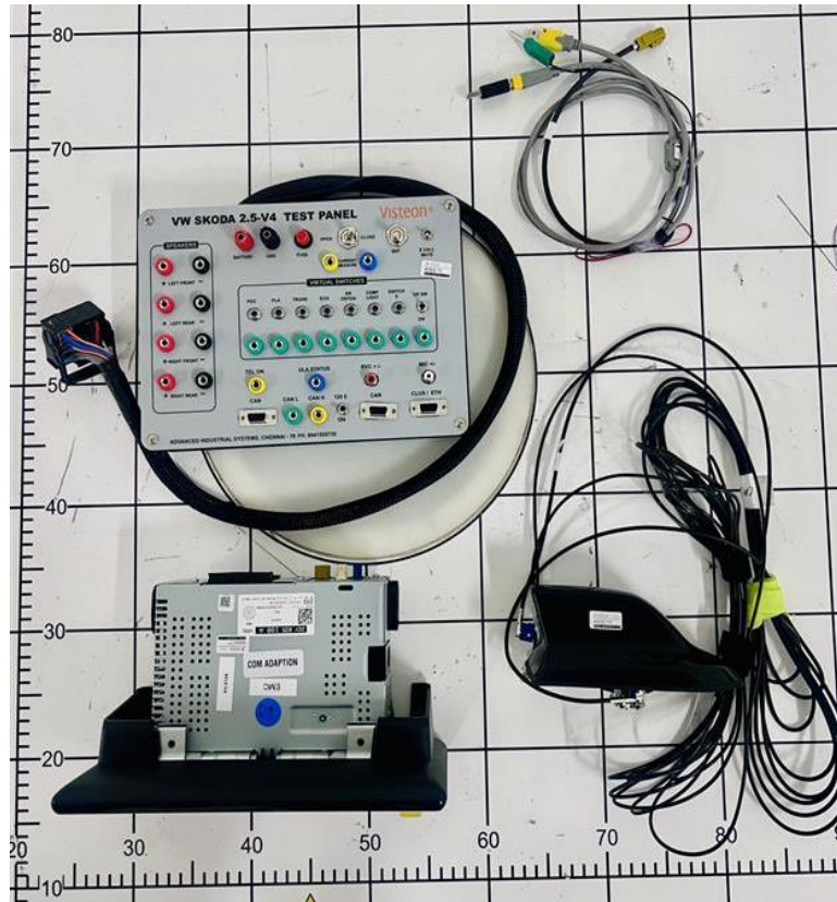
3. Top View of the DUT and accessories
