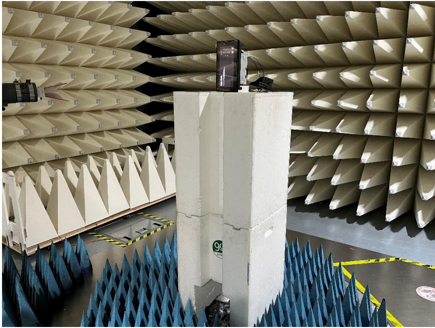
6. Radiated Emission test setup 3
