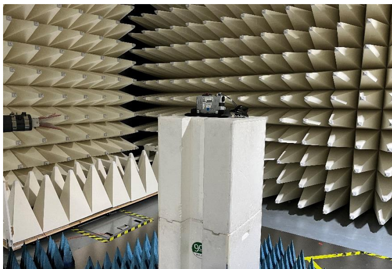
Figure C7. High Range Radiated Emission test setup 18-26GHz
