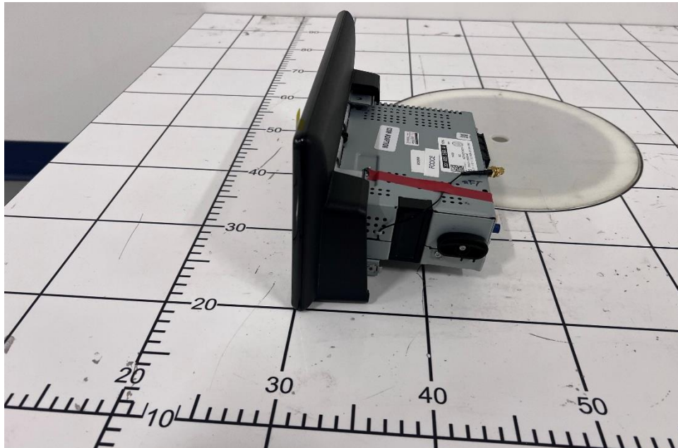
Figure C3. Side View of DUT
