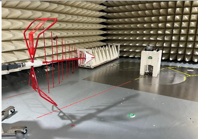
Figure C5. Low Range Radiated Emission test setup
