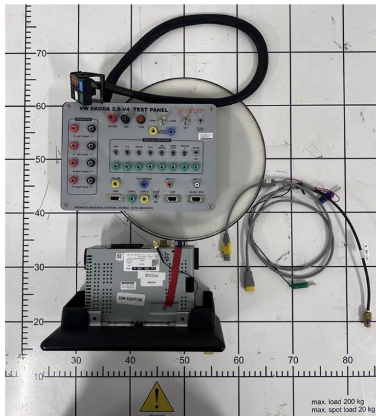
Figure C4. Front View of Conducted and Radiated samples with Accessories
