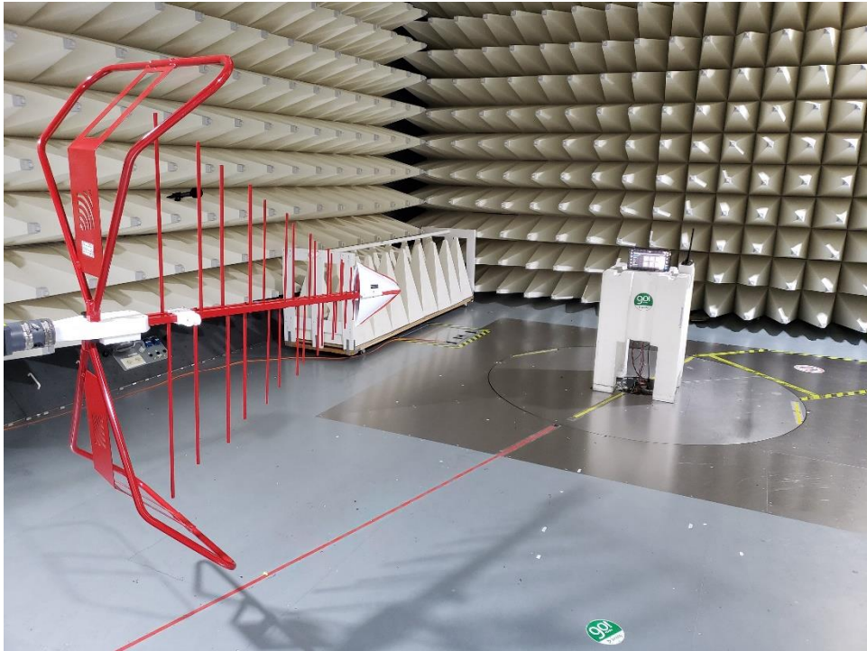
4. Radiated Emission test setup 1
