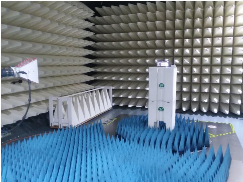
5. Radiated Emission test setup 2
