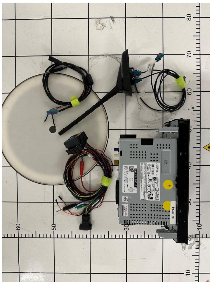
3. Top View of the DUT and accessories
