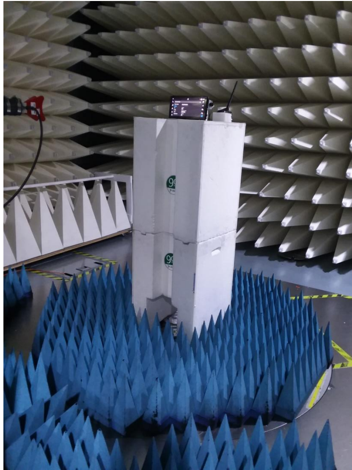
6. Radiated Emission test setup 3
