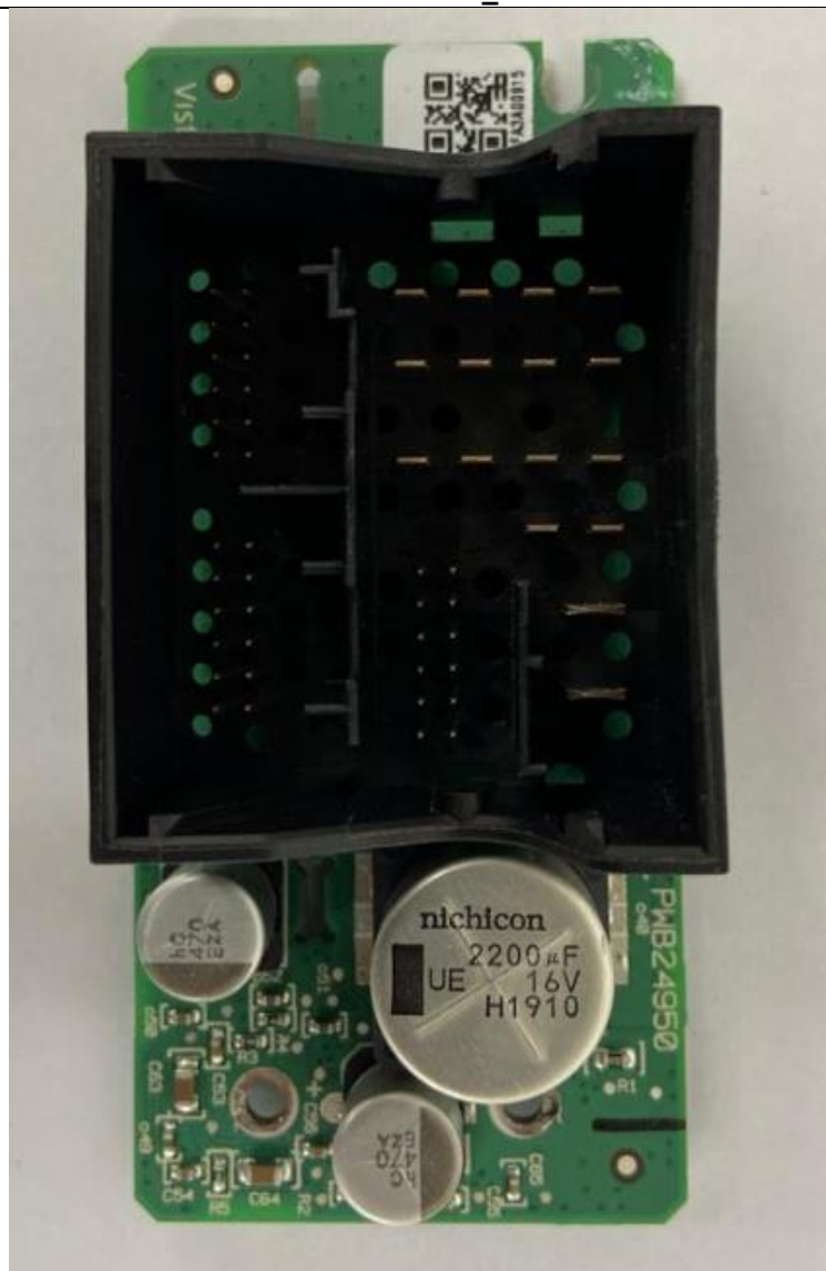
Rear Board_2
