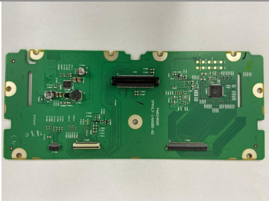
Front Board_1
