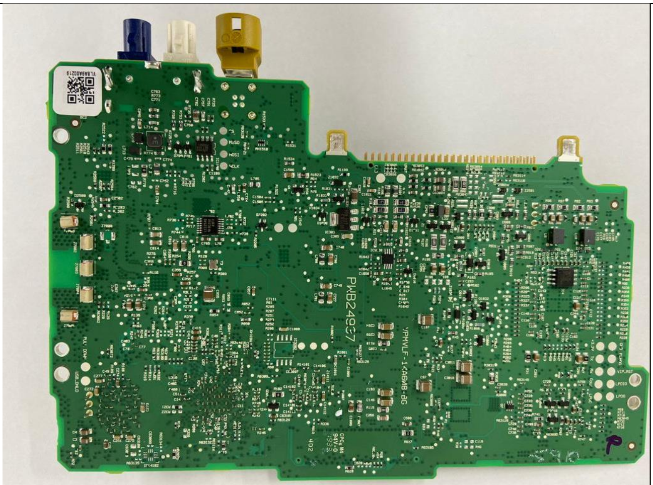
Main Board_1
