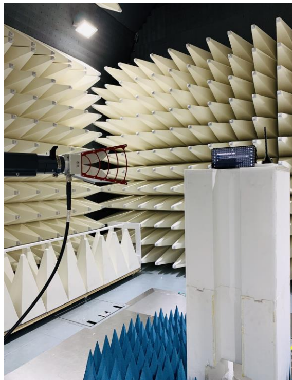
FigureC2. Radiated Setup – High Range
