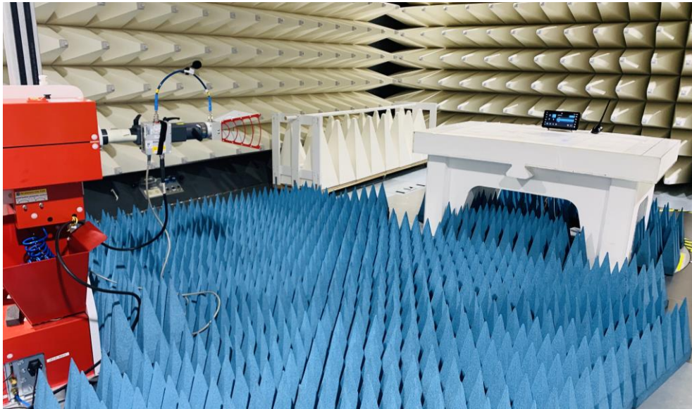
Figure B5: : Radiated Emission testing High range Setup
