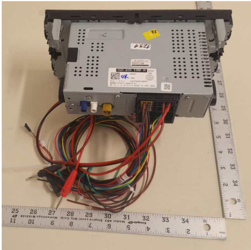
Figure B3: EUT with Harness attached
