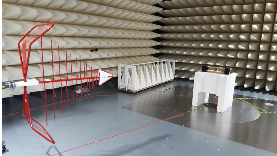
Figure B5. Radiated emission Setup – Low Range 30 to 1000 MHz
