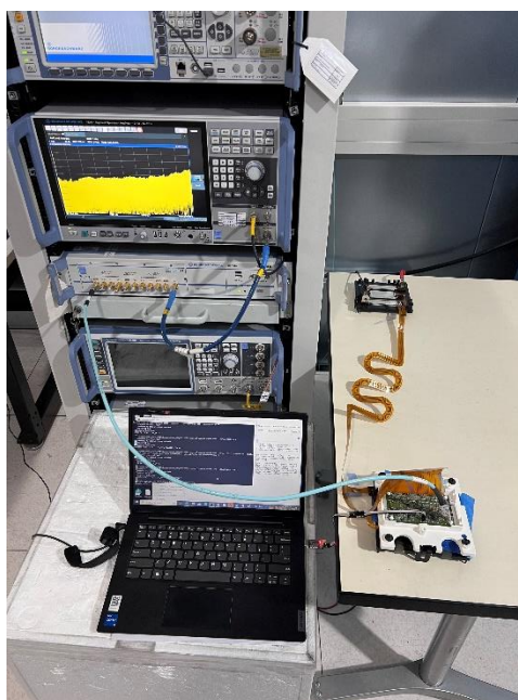
Figure B4. Conducted setup
