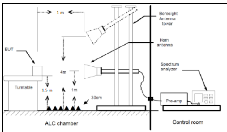
Radiated measurements setup f > 18 \text{ GHz}
