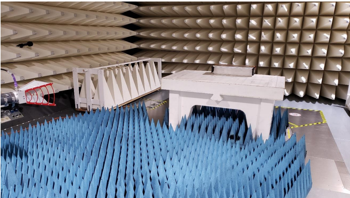
4. Radiated Emission test setup High Range
