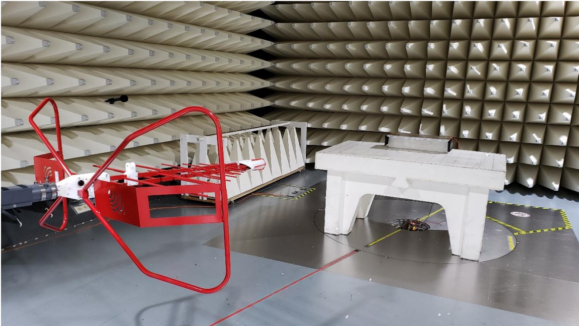
3. Radiated Emission test setup Low Range
