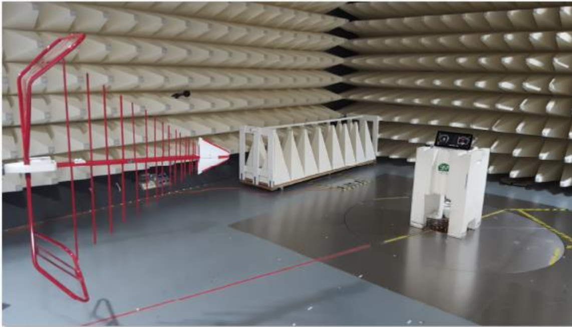
4. Radiated Emission test setup 1
