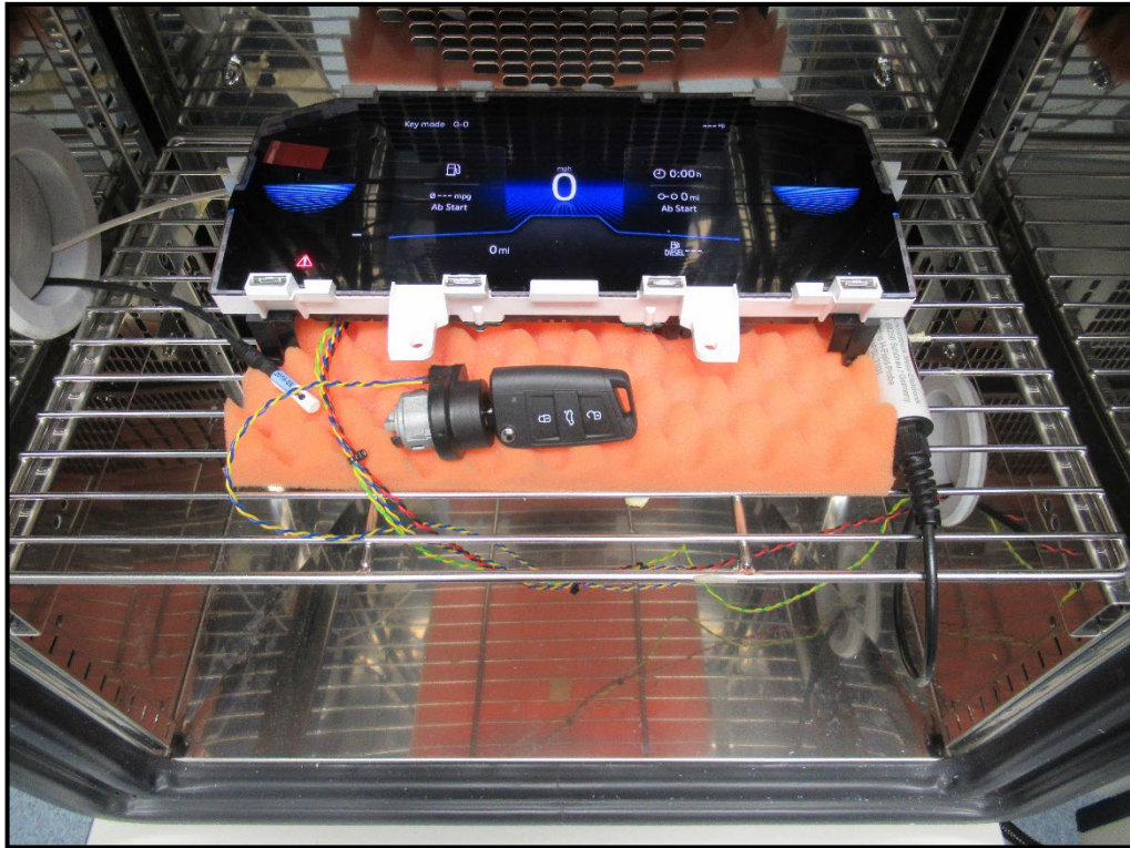
Photo 5: (99% / 20 dB) Bandwidth Test Setup
