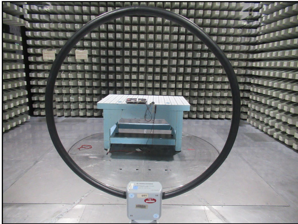
Photo 1: Radiated Test Setup from 9 kHz to 30 MHz
