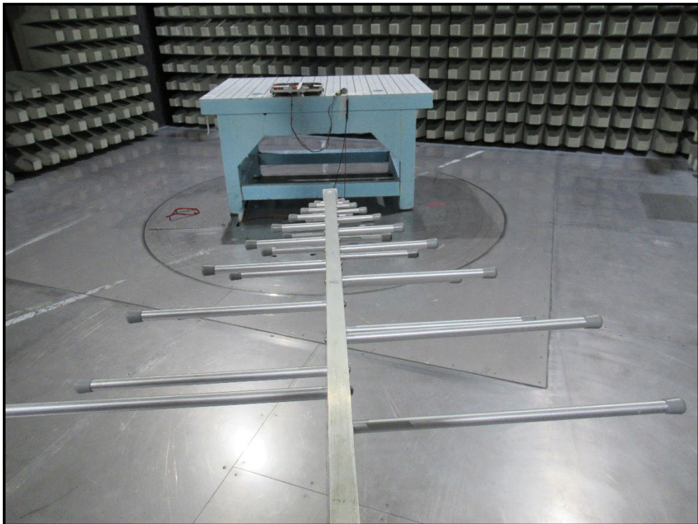
Photo 1: Radiated Test Setup from 30 MHz to 1 GHz
