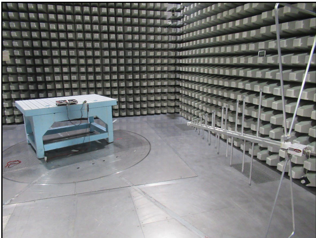
Photo 2: Radiated Test Setup from 30 MHz to 1 GHz
