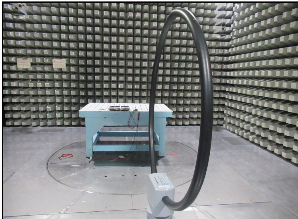
Photo 2: Radiated Test Setup from 9 kHz to 30 MHz
