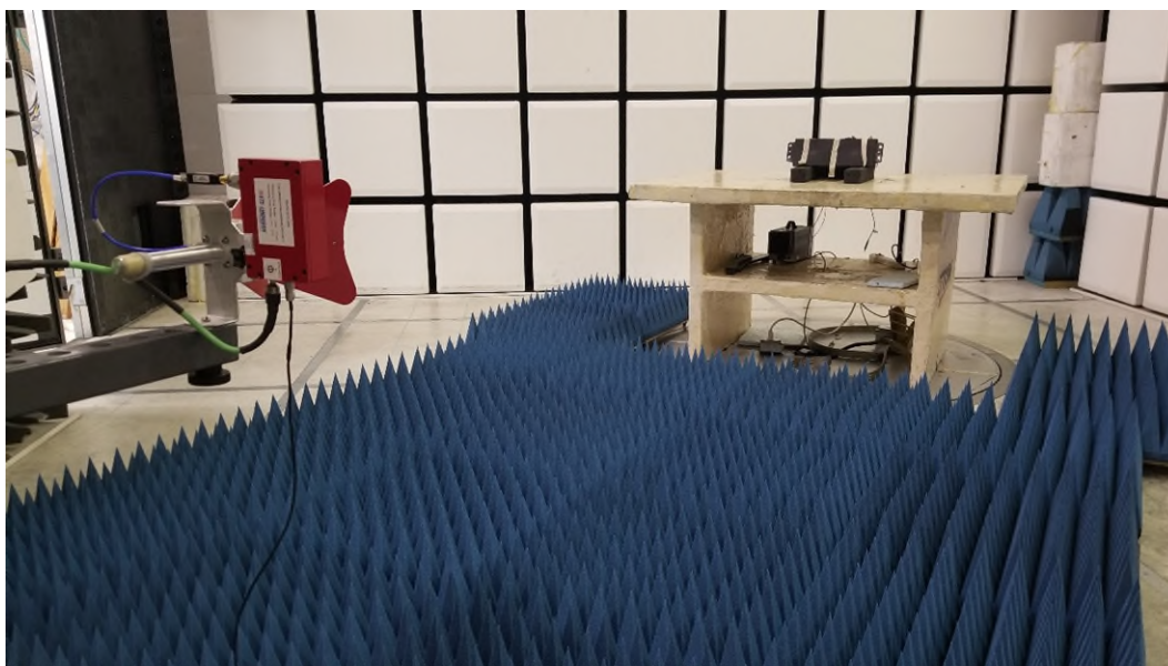
Photo 3: Emissions in frequency range 3-18 GHz
