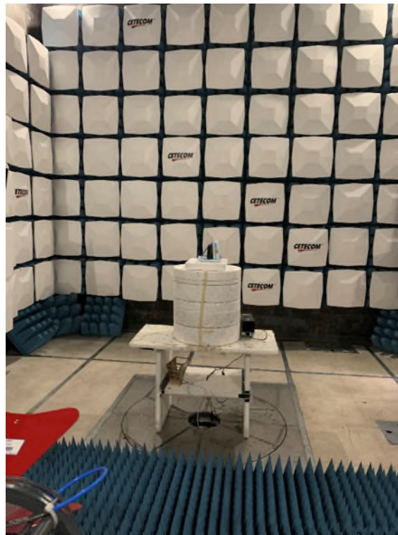
Photo 4: Emissions in frequency range 3-18 GHz
