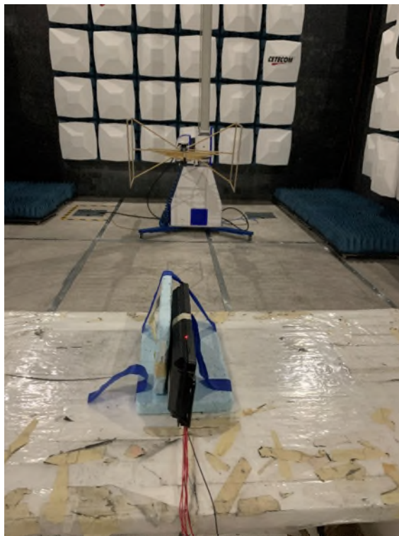
Photo 2: Emissions in frequency range 30 MHz to 1 GHz
