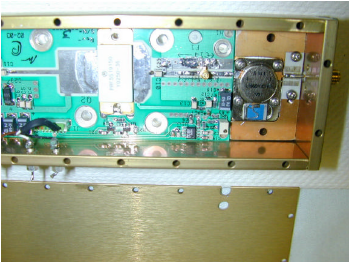
Amplifier PCB Top (Right Side)
