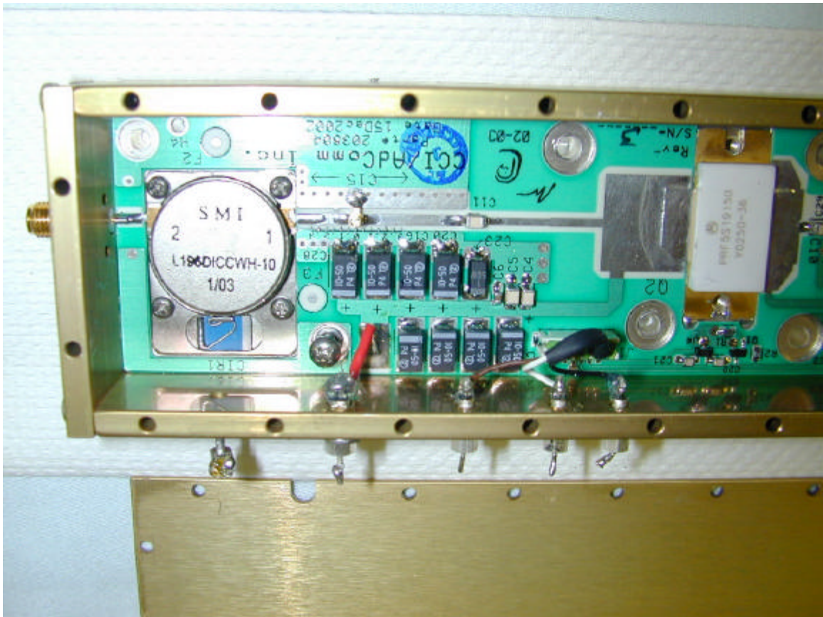
Amplifier PCB Top (Left Side)
