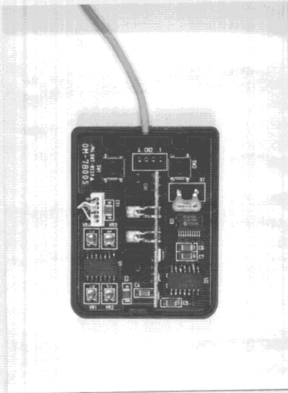
Top View of printed circuit board on mouse base
