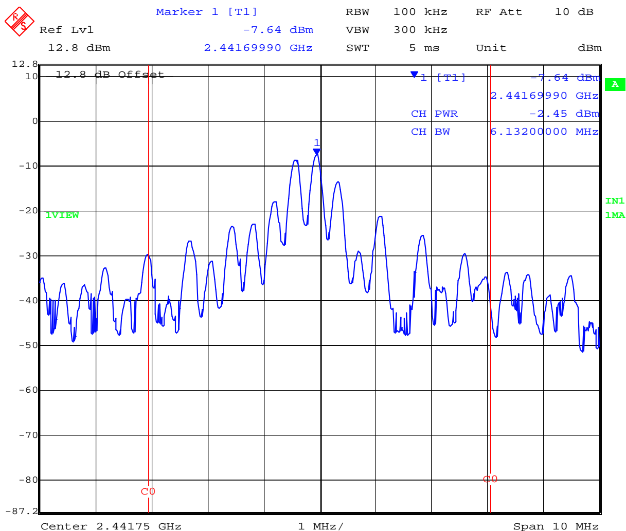
Plot 04 2441.75 MHz Peak Power (dBm)
