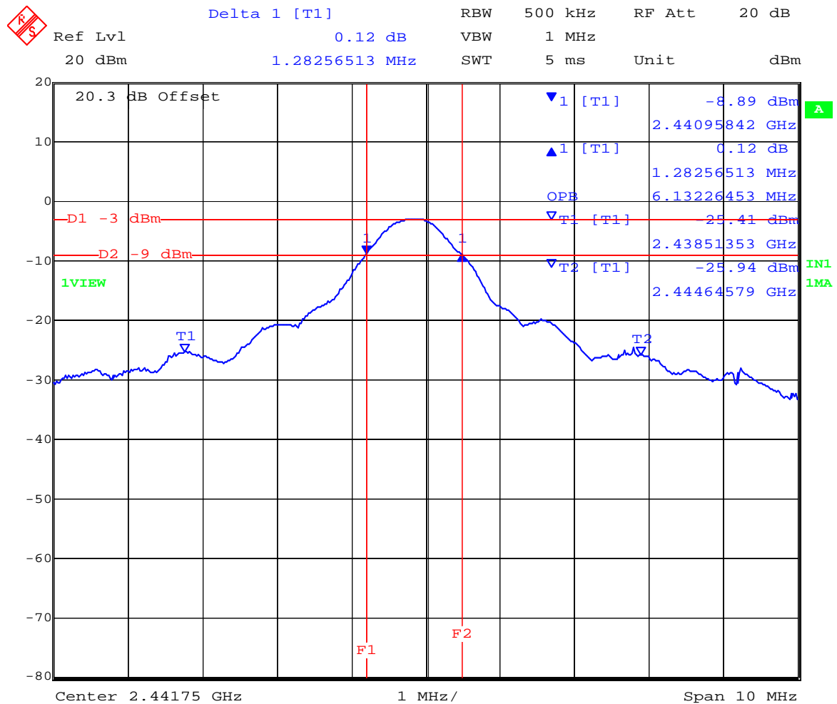
Plot 02 6 dB and 99% Bandwidth
