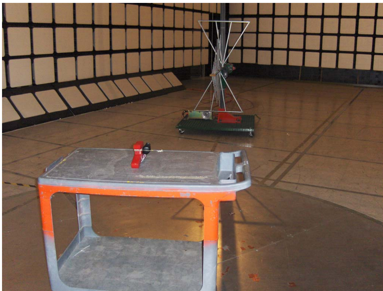
Radiated Emission at 3 m Distance (Orthogonal Position 3)
