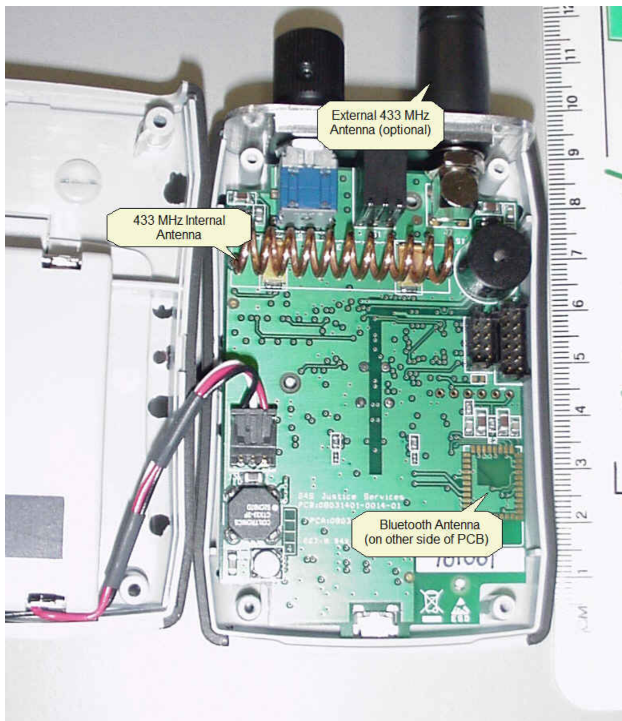
Figure 3: Bottom view of main PCB showing location of various antenna's (scale in centimeters is included for measurement reference purposes)
