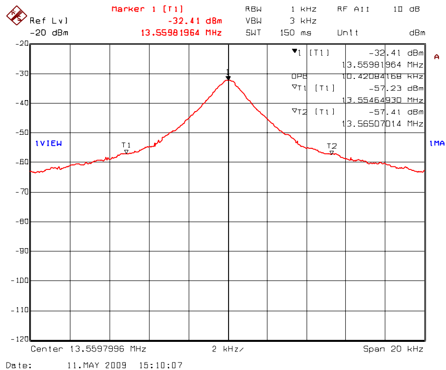
Plot 5.7.4.2. 99% Occupied Bandwidth Test Frequency: 13.56 MHz
