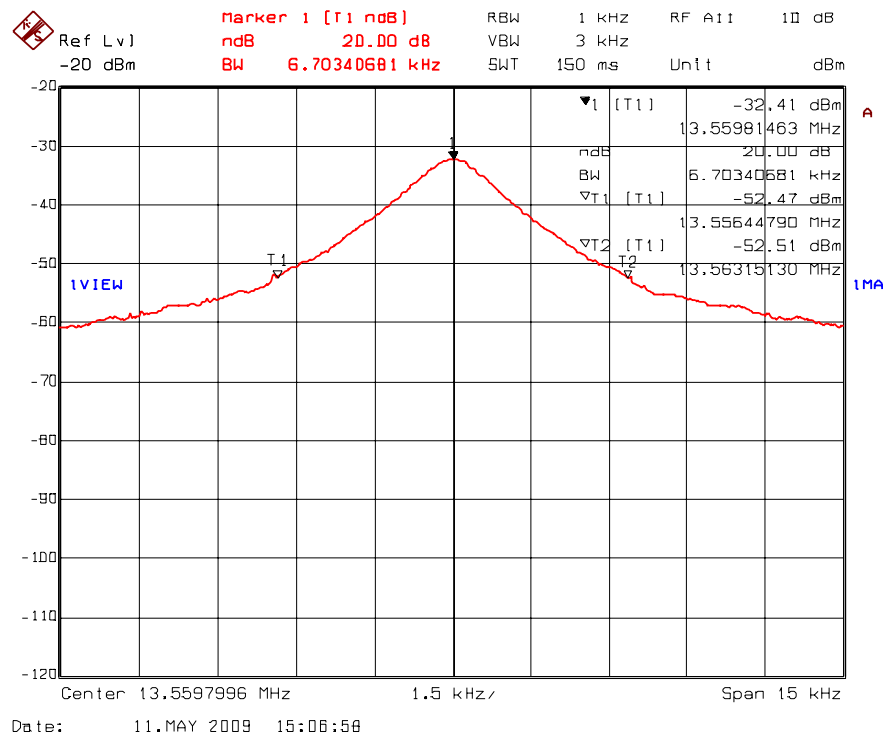
Plot 5.7.4.1. 20 dB Bandwidth Test Frequency: 13.56 MHz
