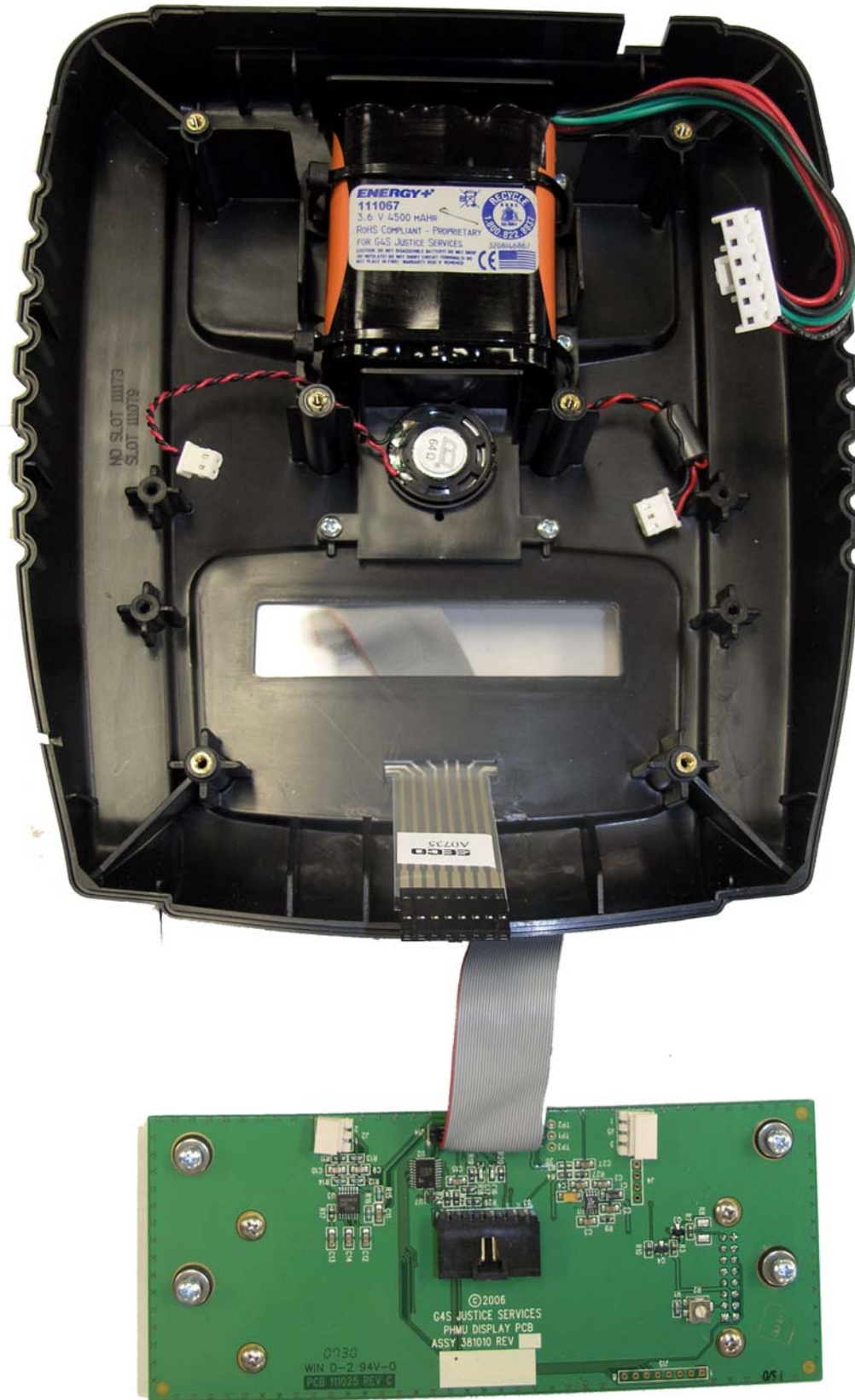
G4S Justice Services Canada, Inc. Product: PHMUC, Model: PHMUC08 FCC ID: NSNPHMUC08, IC: 7995A-PHMUC08
