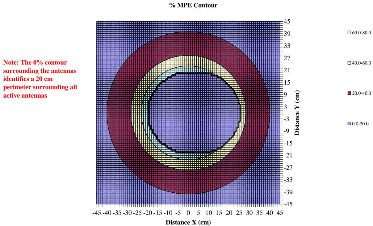
Plot 5. Simultaneous transmission of Xemics Transceiver A & GSM in GSM850 mode { 433.92, 0.00002, 0.0, 5.5, 0 } & { 835, 1.778, 1.0, 0, 0 }
