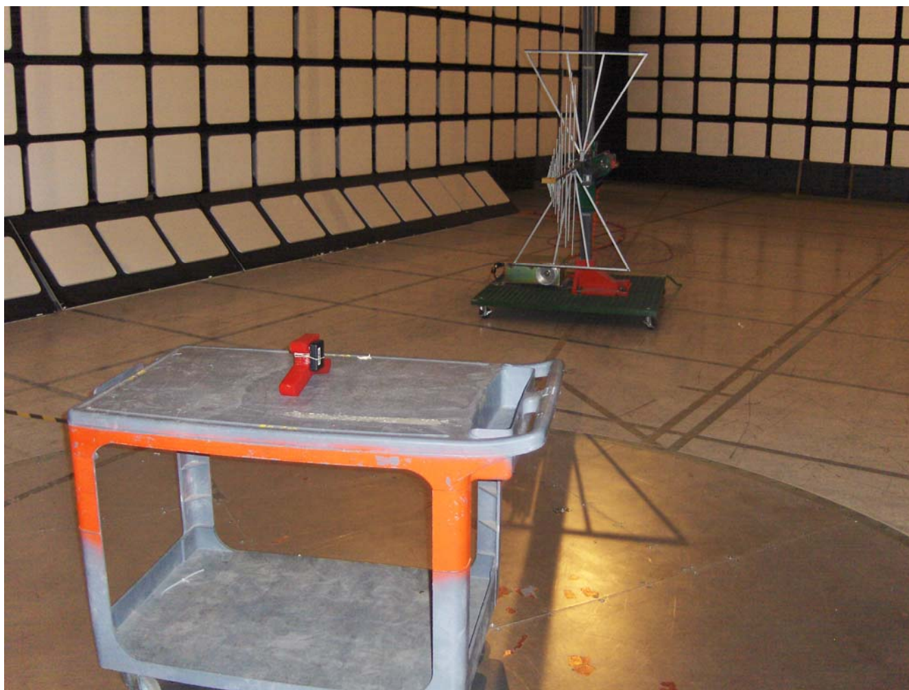
Radiated Emission at 3 m Distance (Orthogonal Position 2)
