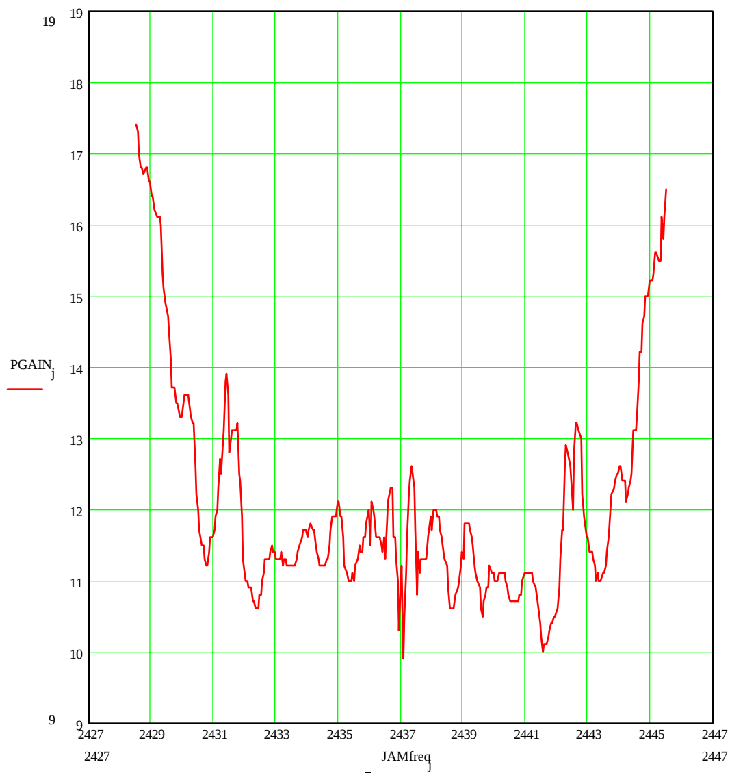
GRAPH OF HWN SLICE PROCESSING GAIN VERSUS JAMMER FREQUENCY IEEE 802.11 CHANNEL 6
