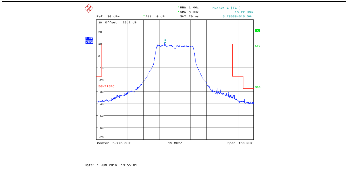
Plot 5.3.4.1.21. Band-Edge Conducted Emissions, 802.11an HT40, 135 Mbps, Ch 159, 5795 MHz, PCDAC Power 40, ANT 1 Offset = 29.16dB = 27.16dB Insertion Loss + 2dBi EUT antenna gain
