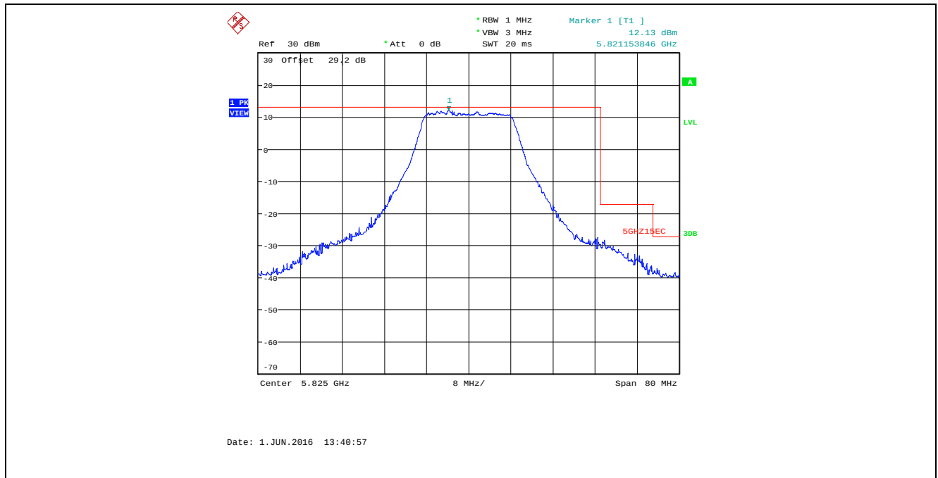
Plot 5.3.4.1.16. Band-Edge Conducted Emissions, 802.11an HT20, 65 Mbps, Ch 165, 5825 MHz, PCDAC Power 40, ANT 1 Offset = 29.16dB = 27.16dB Insertion Loss + 2dBi EUT antenna gain
