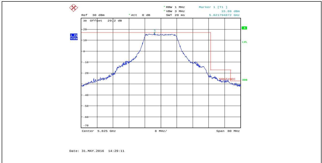
Plot 5.3.4.1.11. Band-Edge Conducted Emissions, 802.11a, 54 Mbps, Ch 165, 5825 MHz, PCDAC Power 83, ANT 2 Offset = 29.16dB = 27.16dB Insertion Loss + 2dBi EUT antenna gain
