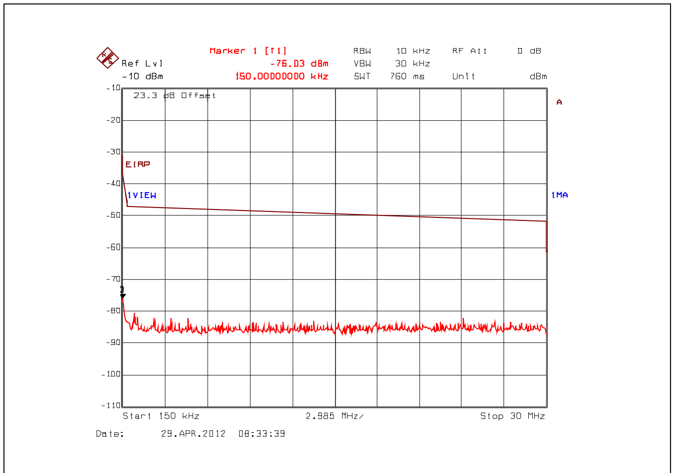
Plot 5.4.4.4.15. Conducted Spurious Emissions – Restricted Bands 802.11b, 2462 MHz, CCK 11 Mbps, 150 kHz - 30 MHz, Peak Detector
