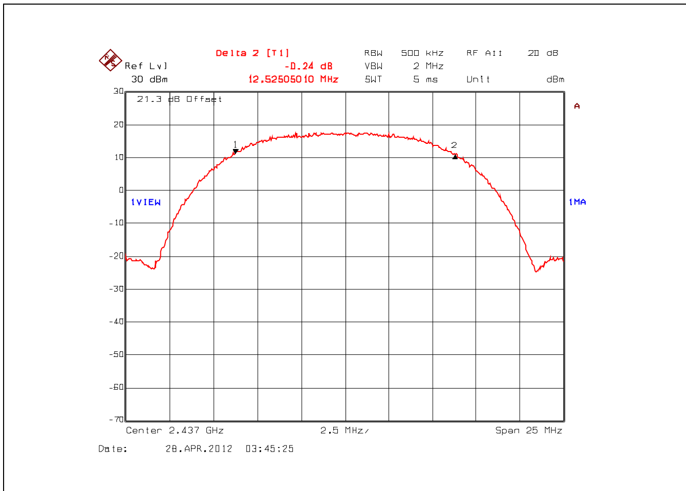
Plot 5.2.4.8. 6 dB Bandwidth, 2437 MHz, 802.11b, CCK 11 Mbps
