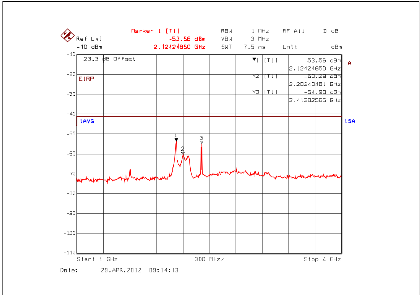
Plot 5.4.4.4.4. Conducted Spurious Emissions – Restricted Bands 802.11b, 2412 MHz, CCK 11 Mbps, 1 GHz - 4 GHz, Trace Average with Band (Notch) Reject Filter
