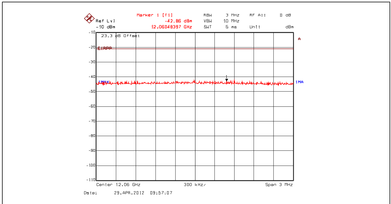
Plot 5.4.4.4.6. Conducted Spurious Emissions – Restricted Bands 802.11b, 2412 MHz, CCK 11 Mbps, 4 GHz - 25 GHz, Peak Power at 12.06 GHz with High Pass Filter
