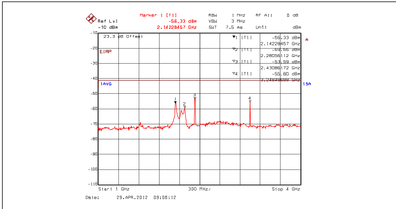
Plot 5.4.4.4.29. Conducted Spurious Emissions – Restricted Bands 802.11g, 2437 MHz, 64-QAM 54 Mbps, 1 GHz - 4 GHz, Trace Averaging with Band (Notch) Reject Filter
