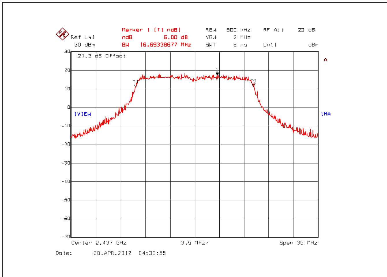
Plot 5.2.4.17. 6 dB Bandwidth, 2437 MHz, 802.11g, 16-QAM, 36 Mbps
