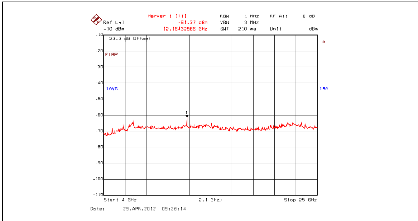
Plot 5.4.4.4.31. Conducted Spurious Emissions – Restricted Bands 802.11g, 2437 MHz, 64-QAM 54 Mbps, 4 GHz - 25 GHz, Trace Averaging with High Pass Filter
