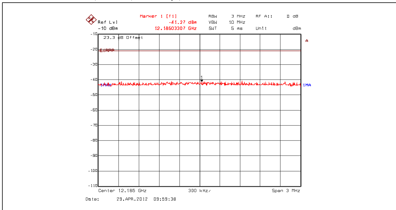
Plot 5.4.4.4.13. Conducted Spurious Emissions – Restricted Bands 802.11b, 2437 MHz, CCK 11 Mbps, Peak Power at 12.19 GHz with Band Pass Filter
