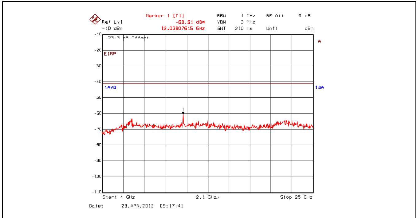
Plot 5.4.4.4.5. Conducted Spurious Emissions – Restricted Bands 802.11b, 2412 MHz, CCK 11 Mbps, 4 GHz - 25 GHz, Trace Average with High Pass Filter
