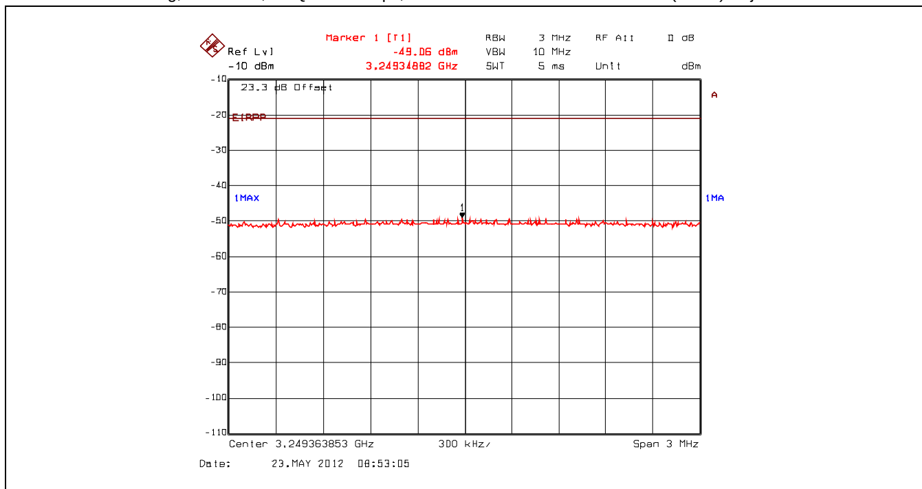
Plot 5.4.4.4.30. Conducted Spurious Emissions – Restricted Bands 802.11g, 2437 MHz, 64-QAM 54 Mbps, Peak Power at 3.25 GHz with Band (Notch) Reject Filter
