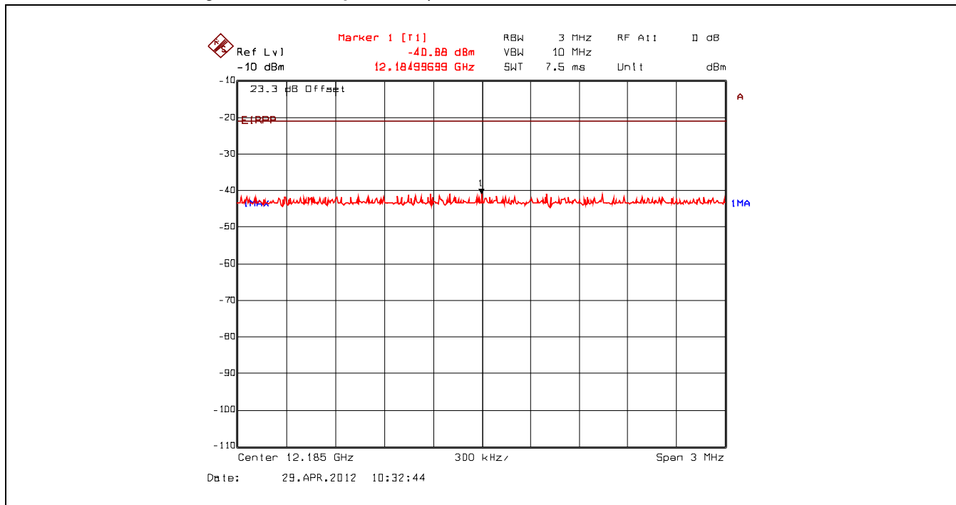
Plot 5.4.4.4.32. Conducted Spurious Emissions – Restricted Bands 802.11g, 2437 MHz, 64-QAM 54 Mbps, Peak Power at 12.18 GHz with Band Pass Filter
