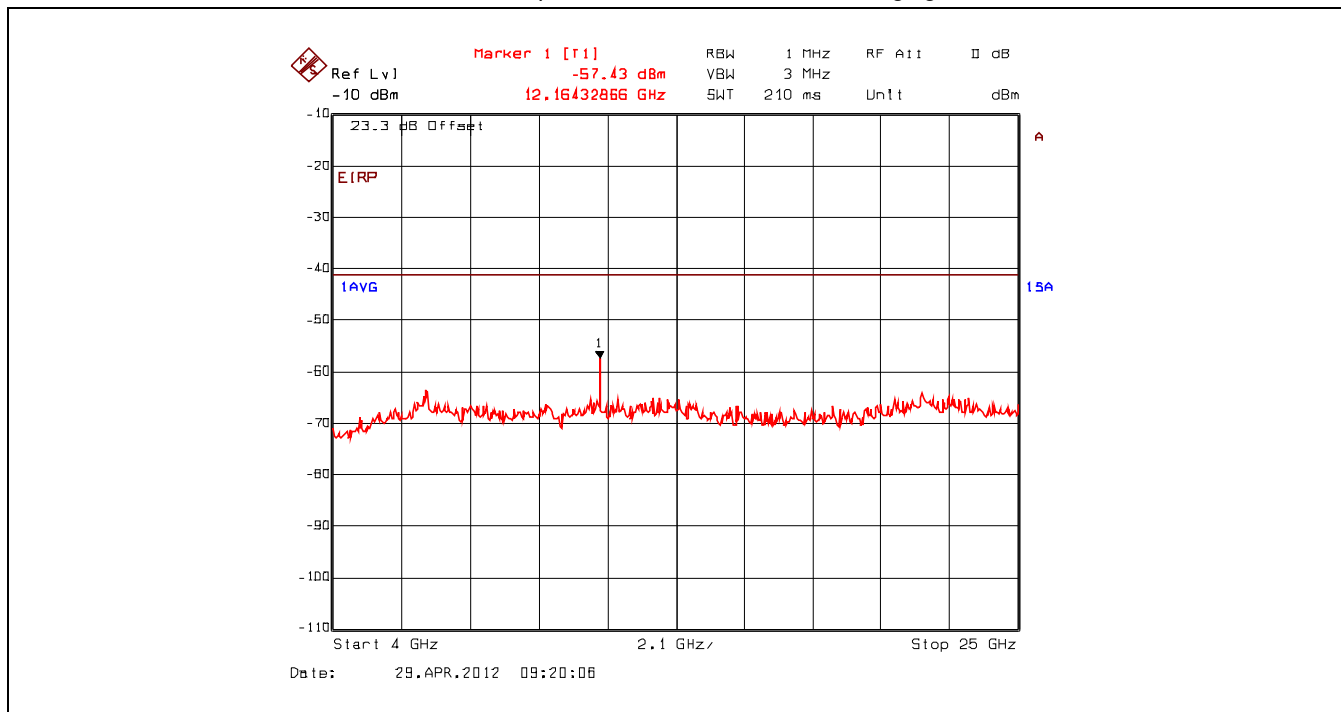
Plot 5.4.4.4.12. Conducted Spurious Emissions – Restricted Bands 802.11b, 2437 MHz, CCK 11 Mbps, 4 GHz - 25GHz, Trace Averaging with Band Pass Filter
