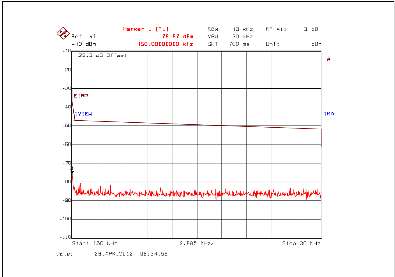
Plot 5.4.4.8. Conducted Spurious Emissions – Restricted Bands 802.11b, 2437 MHz, CCK 11 Mbps, 150 kHz - 30 MHz, Peak Detector
