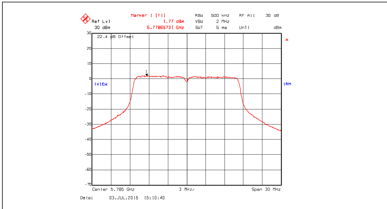
Plot 5.4.4.9. Power Spectral Density, Data Rate 2, Chain # 1, Ch 157, 5785 MHz, Software Output Power Setting 19
