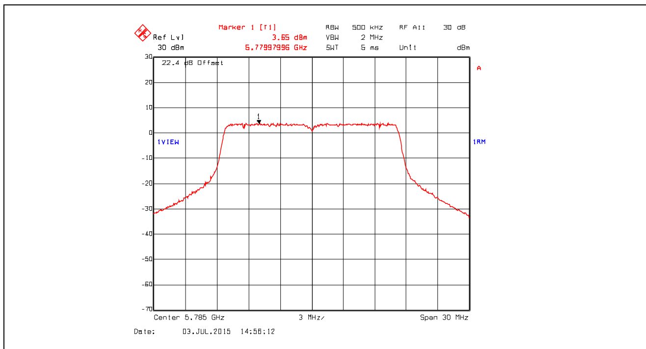
Plot 5.4.4.10. Power Spectral Density, Data Rate 2, Chain # 2, Ch 157, 5785 MHz, Software Output Power Setting 19
