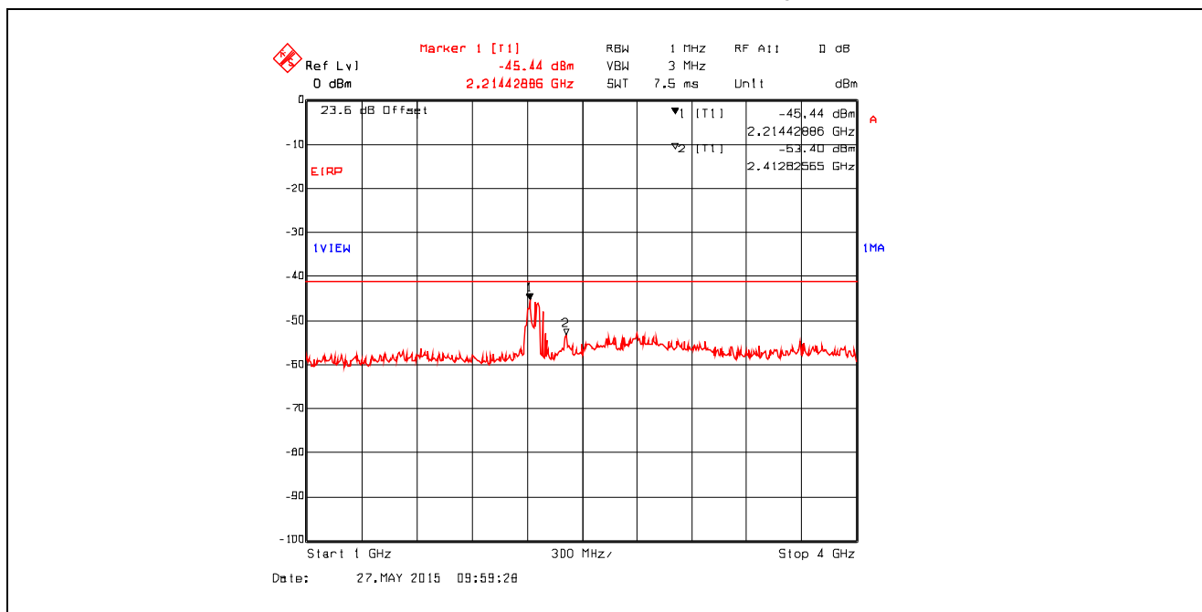
Plot 5.4.4.3.38. Conducted Spurious Emissions in Restricted Frequency Bands Chain #2 , Data Rate 7, Ch 1, 2412 MHz, Software Output Power Setting 18, 1 GHz - 4 GHz, Peak Detector
