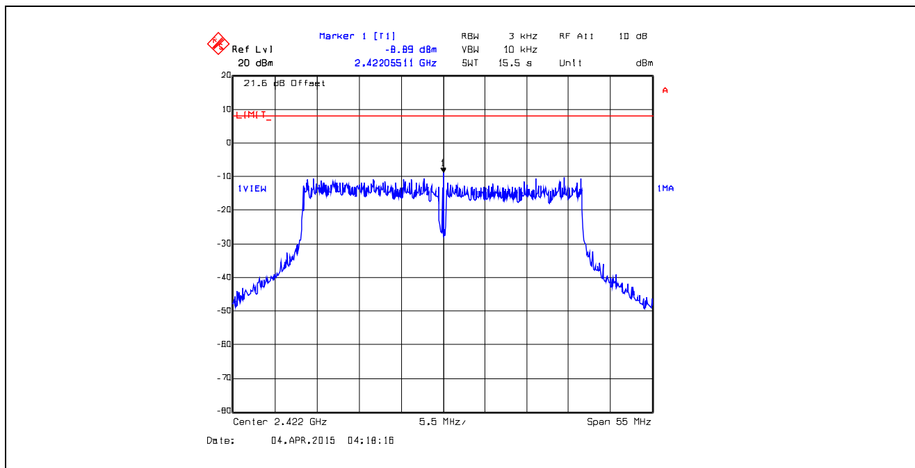
Plot 5.6.4.68. Power Spectral Density Data Rate 12, Chain # 2, Ch 3, 2422 MHz, Software Output Power Setting 17
