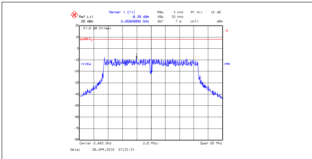
Plot 5.6.4.36. Power Spectral Density Data Rate 6, Chain # 2, Ch 11, 2462 MHz, Software Output Power Setting 18
