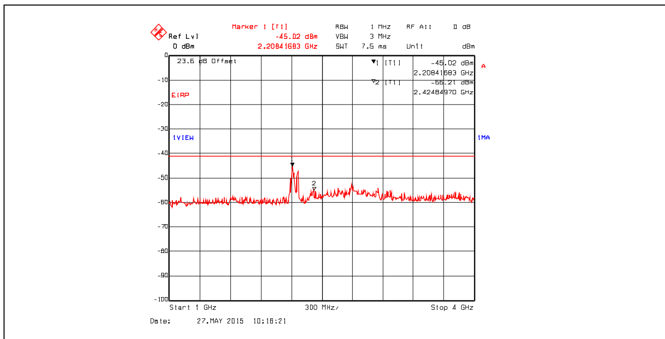
Plot 5.4.4.3.68. Conducted Spurious Emissions in Restricted Frequency Bands Chain #2 , Data Rate 11, Ch 1, 2412 MHz, Software Output Power Setting 19, 1 GHz - 4 GHz, Peak Detector
