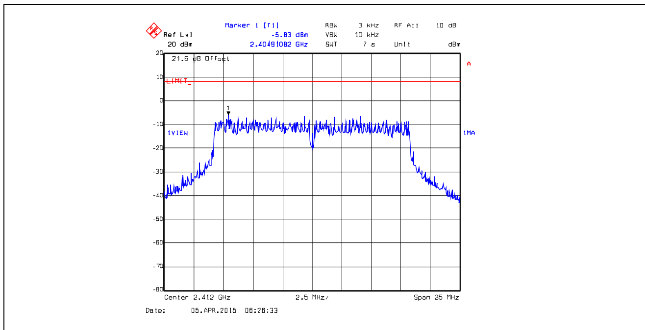
Plot 5.6.4.26. Power Spectral Density Data Rate 5, Chain # 2, Ch 1, 2412 MHz, Software Output Power Setting 18
