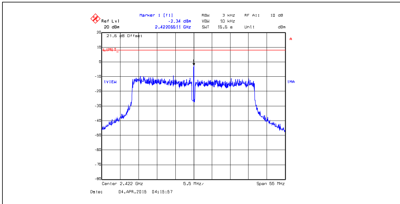
Plot 5.6.4.67. Power Spectral Density Data Rate 12, Chain # 1, Ch 3, 2422 MHz, Software Output Power Setting 17
