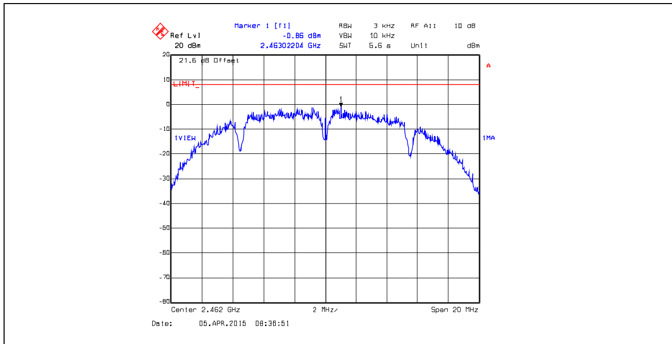
Plot 5.6.4.11. Power Spectral Density Data Rate 2, Chain # 1, Ch 11, 2462 MHz, Software Output Power Setting 26
