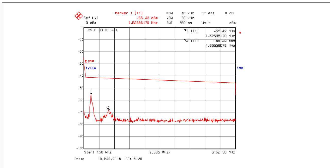
Plot 5.4.4.3.63. Conducted Spurious Emissions in Restricted Frequency Bands Chain #1 , Data Rate 11, Ch 1, 2412 MHz, Software Output Power Setting 19, 150 kHz - 30 MHz, Peak Detector
