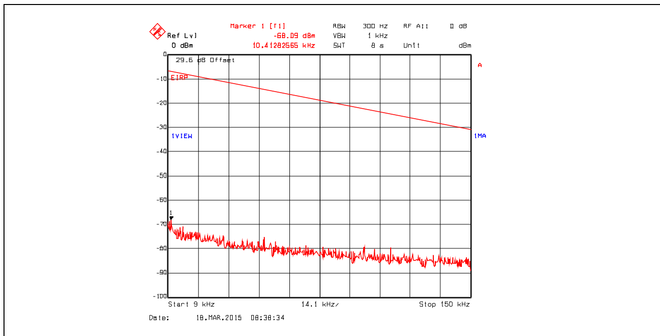
Plot 5.4.4.3.61. Conducted Spurious Emissions in Restricted Frequency Bands Chain #1 , Data Rate 11, Ch 1, 2412 MHz, Software Output Power Setting 19, 9 kHz - 150 kHz, Peak Detector
