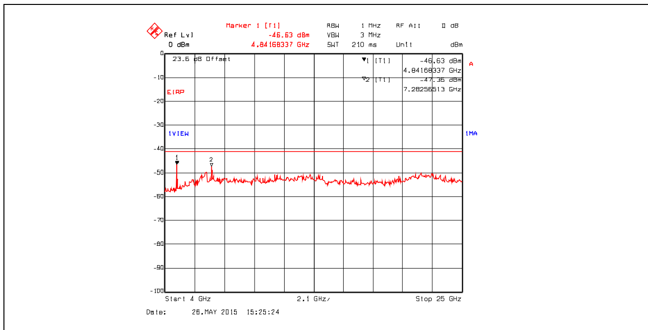
Plot 5.4.4.3.19. Conducted Spurious Emissions in Restricted Frequency Bands Chain #1 , Data Rate 3, Ch 6, 2437 MHz, Software Output Power Setting 26, 4 GHz - 25 GHz, Peak Detector
