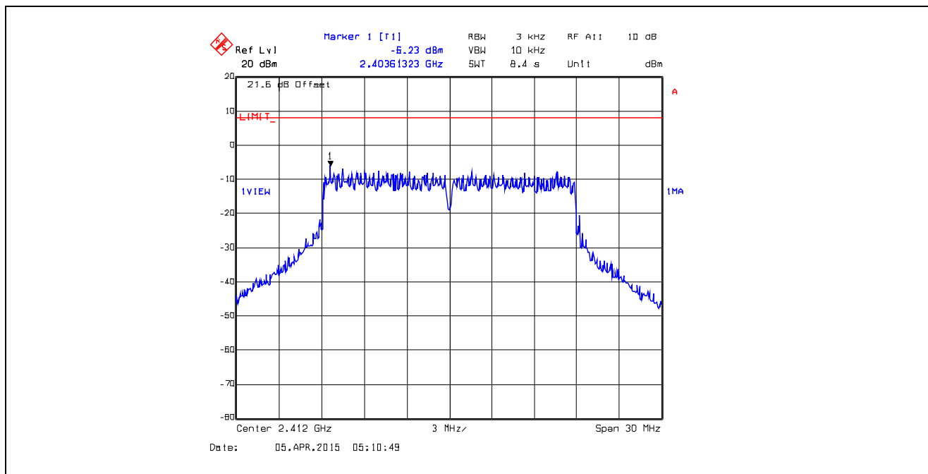
Plot 5.6.4.56. Power Spectral Density Data Rate 10, Chain # 2, Ch 1, 2412 MHz, Software Output Power Setting 19
