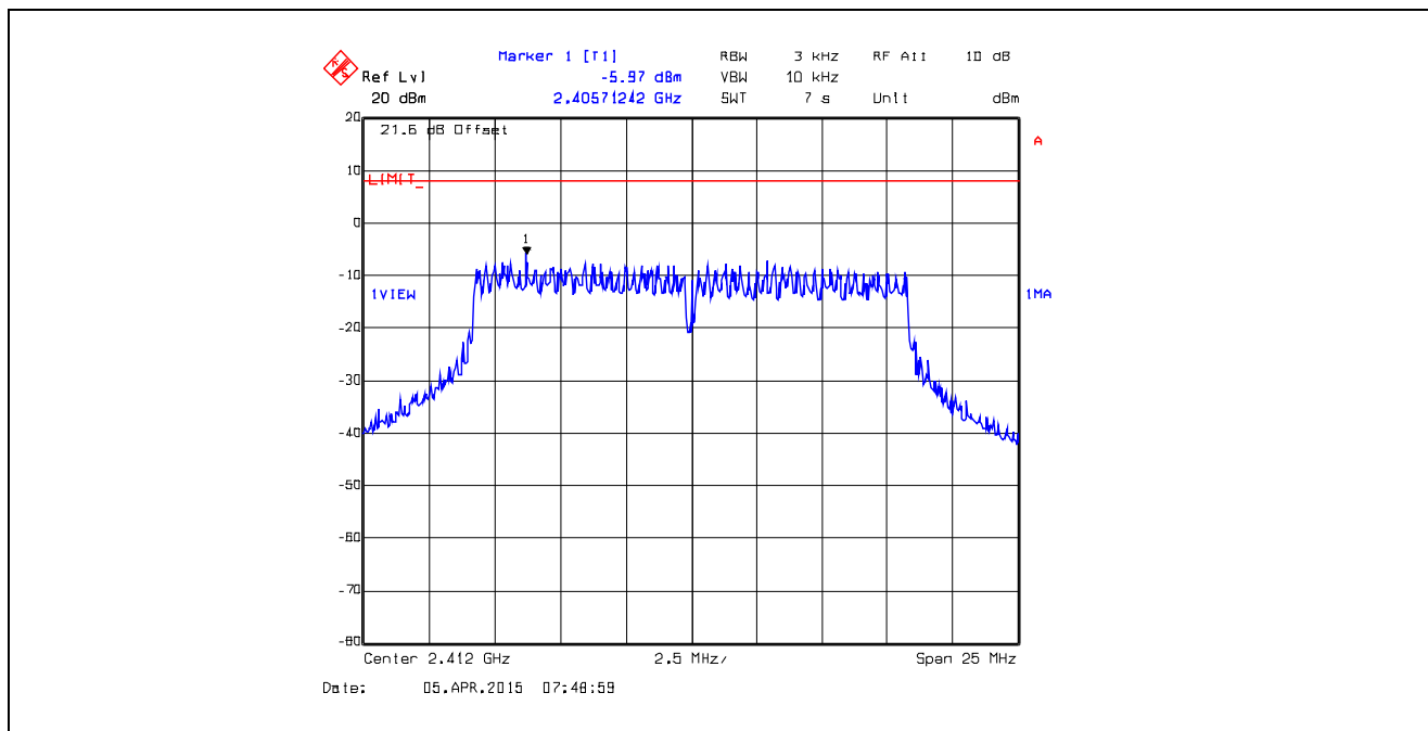
Plot 5.6.4.38. Power Spectral Density Data Rate 7, Chain # 2, Ch 1, 2412 MHz, Software Output Power Setting 18
