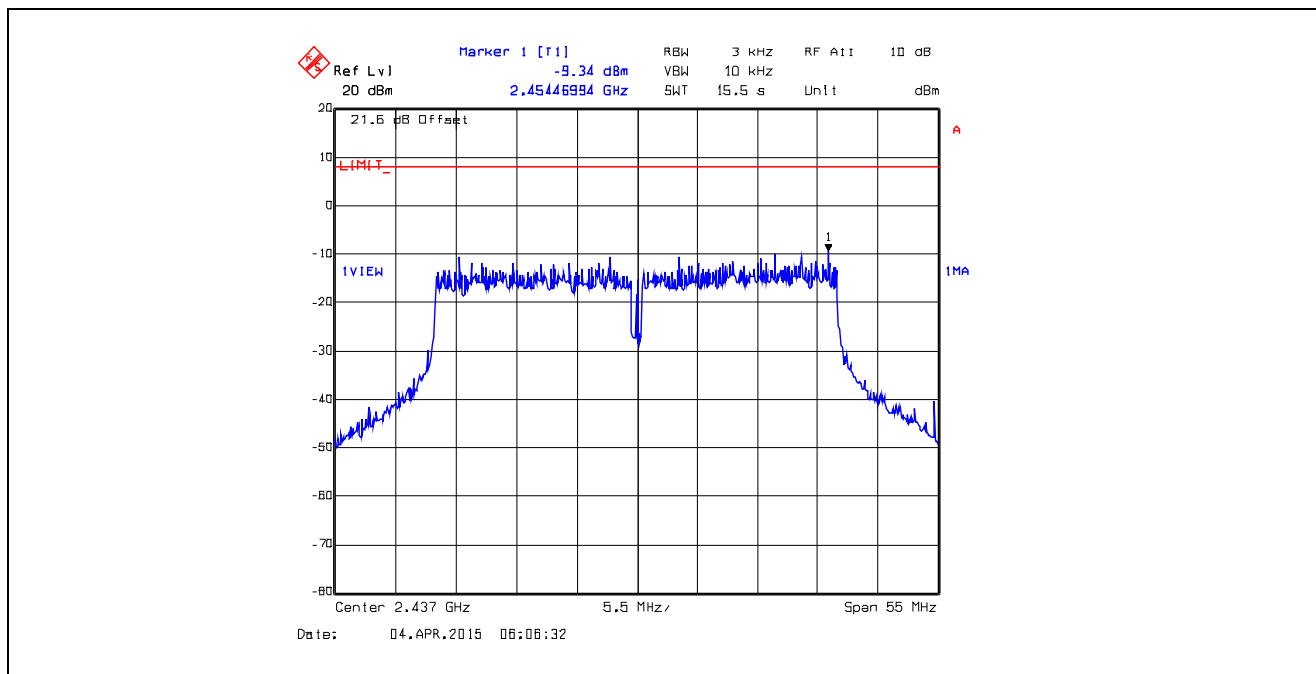
Plot 5.6.4.88. Power Spectral Density Data Rate 15, Chain # 2, Ch 6, 2437 MHz, Software Output Power Setting 17
