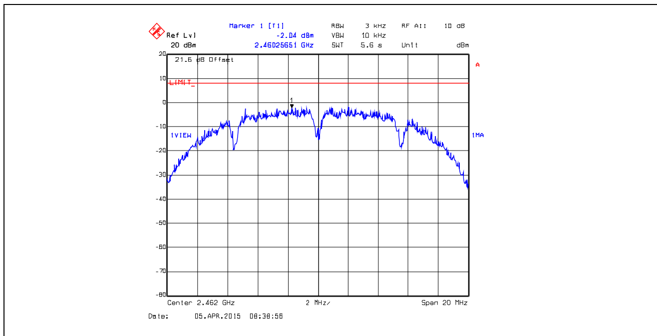
Plot 5.6.4.12. Power Spectral Density Data Rate 2, Chain # 2, Ch 11, 2462 MHz, Software Output Power Setting 26
