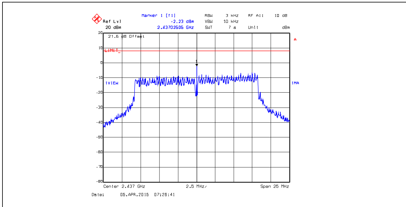
Plot 5.6.4.33. Power Spectral Density Data Rate 6, Chain # 1, Ch 6, 2437 MHz, Software Output Power Setting 18
