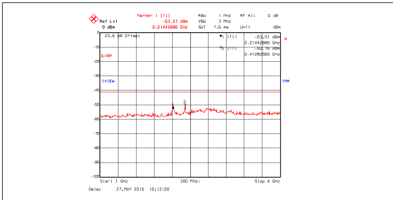
Plot 5.4.4.3.67. Conducted Spurious Emissions in Restricted Frequency Bands Chain #1 , Data Rate 11, Ch 1, 2412 MHz, Software Output Power Setting 19, 1 GHz - 4 GHz, Peak Detector
