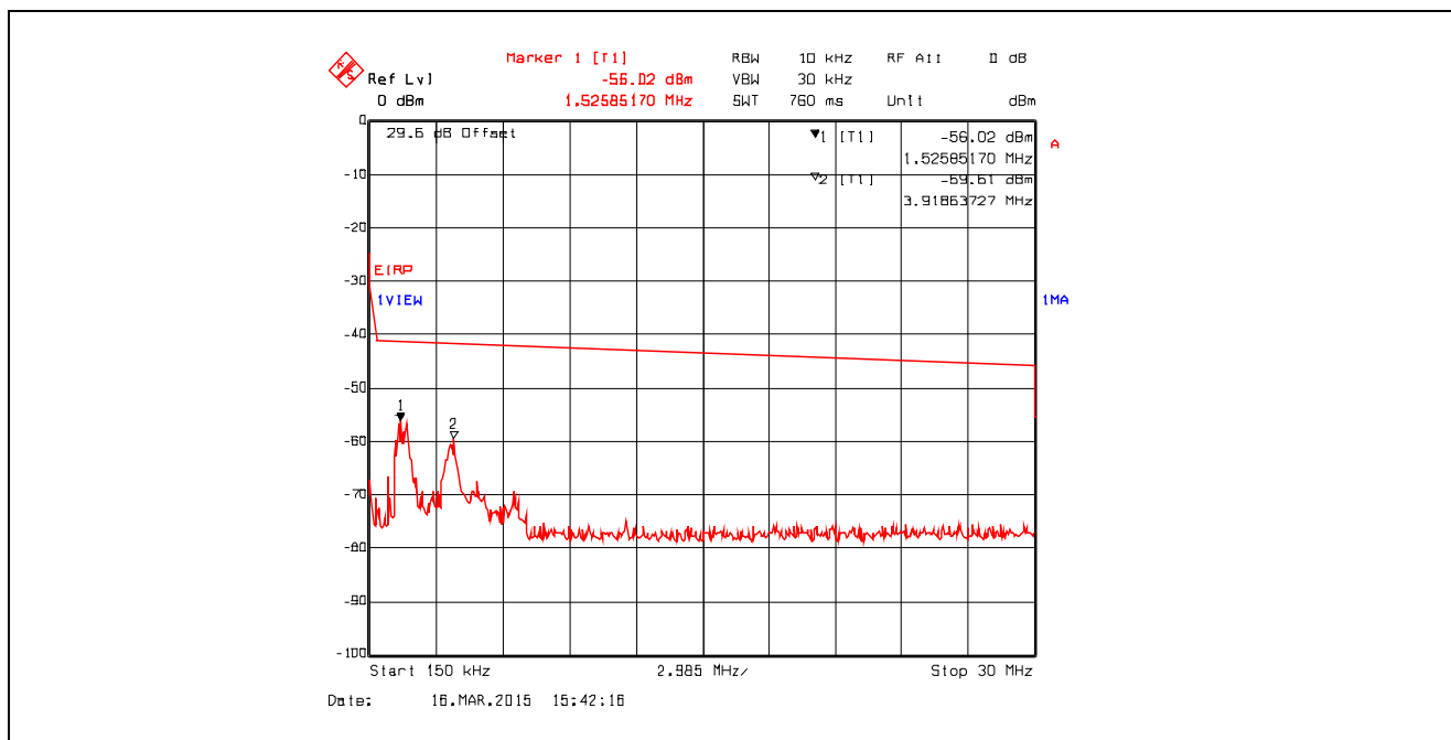
Plot 5.4.4.3.4. Conducted Spurious Emissions in Restricted Frequency Bands Chain #2 , Data Rate 3, Ch 1, 2412 MHz, Software Output Power Setting 26, 150 kHz - 30 MHz, Peak Detector
