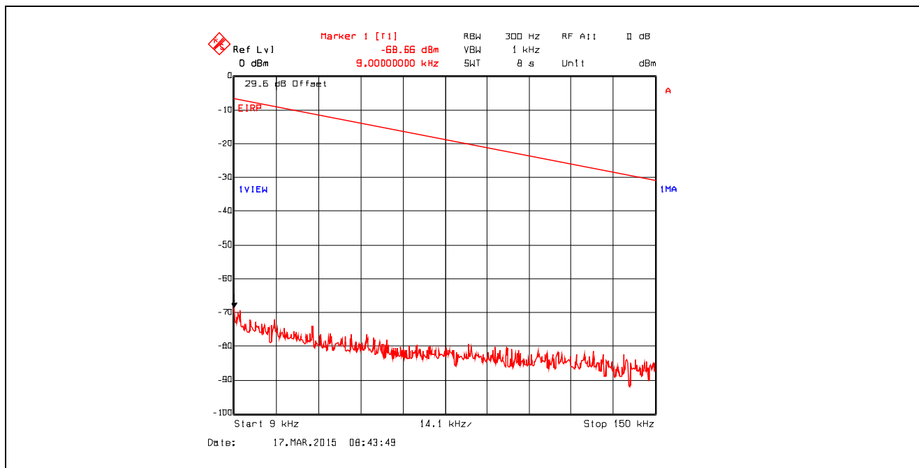
Plot 5.4.4.3.21. Conducted Spurious Emissions in Restricted Frequency Bands Chain #1 , Data Rate 3, Ch 11, 2462 MHz, Software Output Power Setting 26, 9 kHz - 150 kHz, Peak Detector
