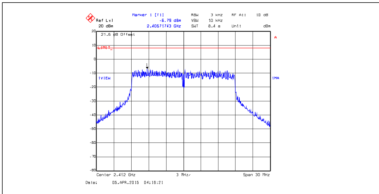
Plot 5.6.4.44. Power Spectral Density Data Rate 8, Chain # 2, Ch 1, 2412 MHz, Software Output Power Setting 19
