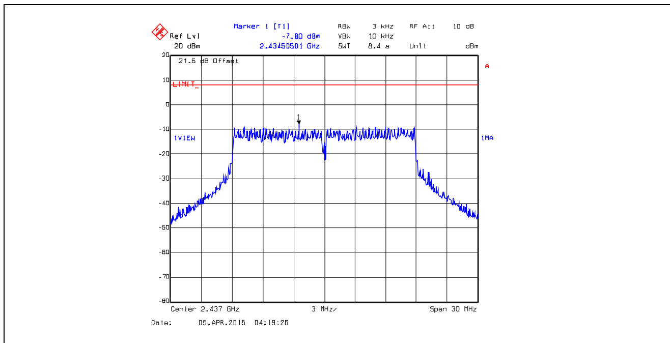
Plot 5.6.4.46. Power Spectral Density Data Rate 8, Chain # 2, Ch 6, 2437 MHz, Software Output Power Setting 19
