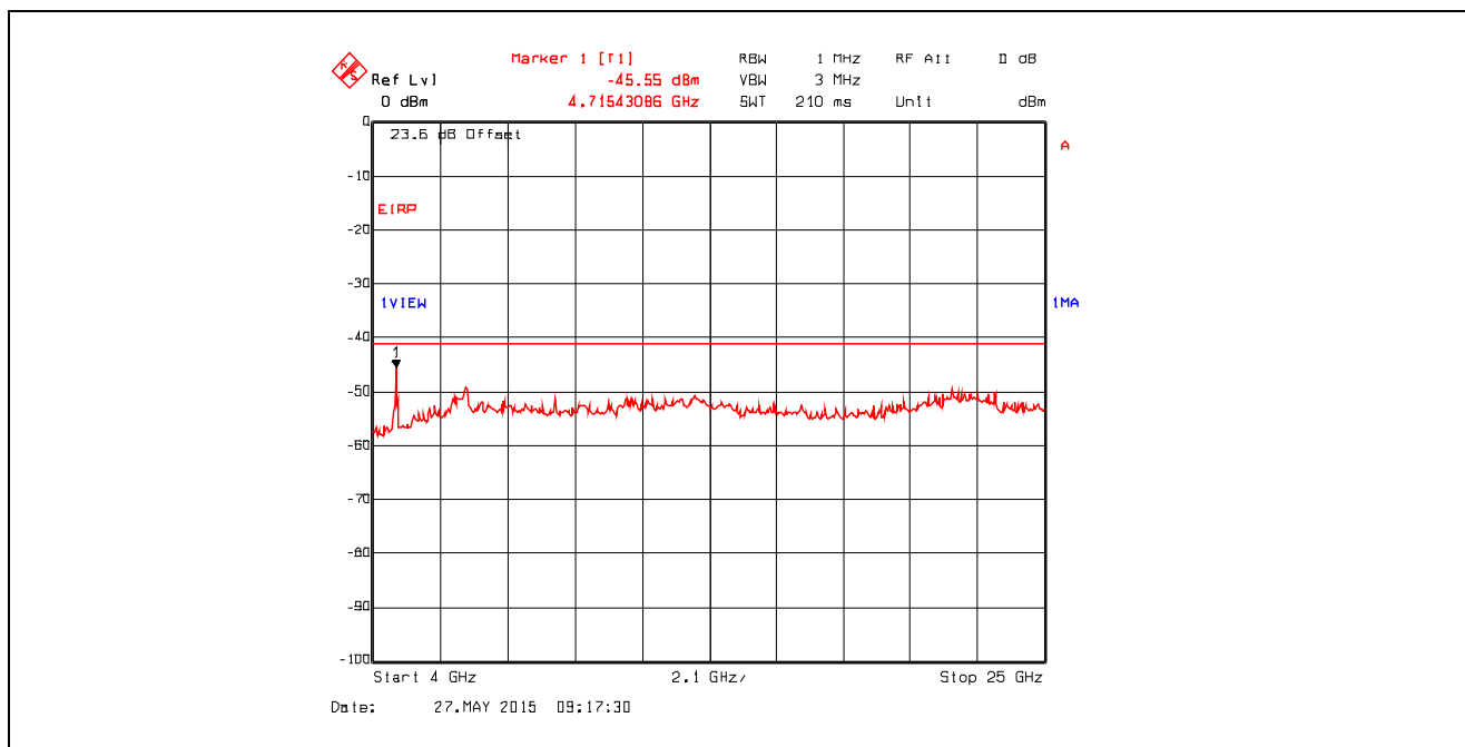
Plot 5.4.4.3.60. Conducted Spurious Emissions in Restricted Frequency Bands Chain #2 , Data Rate 7, Ch 11, 2462 MHz, Software Output Power Setting 18, 4 GHz - 25 GHz, Peak Detector
