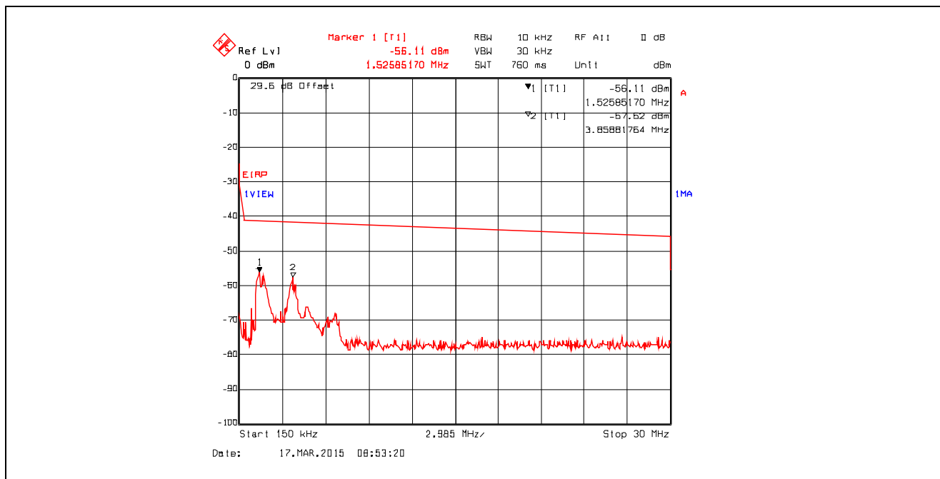
Plot 5.4.4.3.13. Conducted Spurious Emissions in Restricted Frequency Bands Chain #1 , Data Rate 3, Ch 6, 2437 MHz, Software Output Power Setting 26, 150 kHz - 30 MHz, Peak Detector
