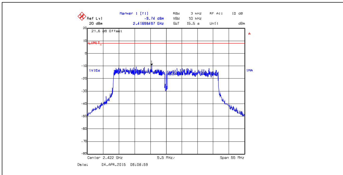
Plot 5.6.4.86. Power Spectral Density Data Rate 15, Chain # 2, Ch 3, 2422 MHz, Software Output Power Setting 17
