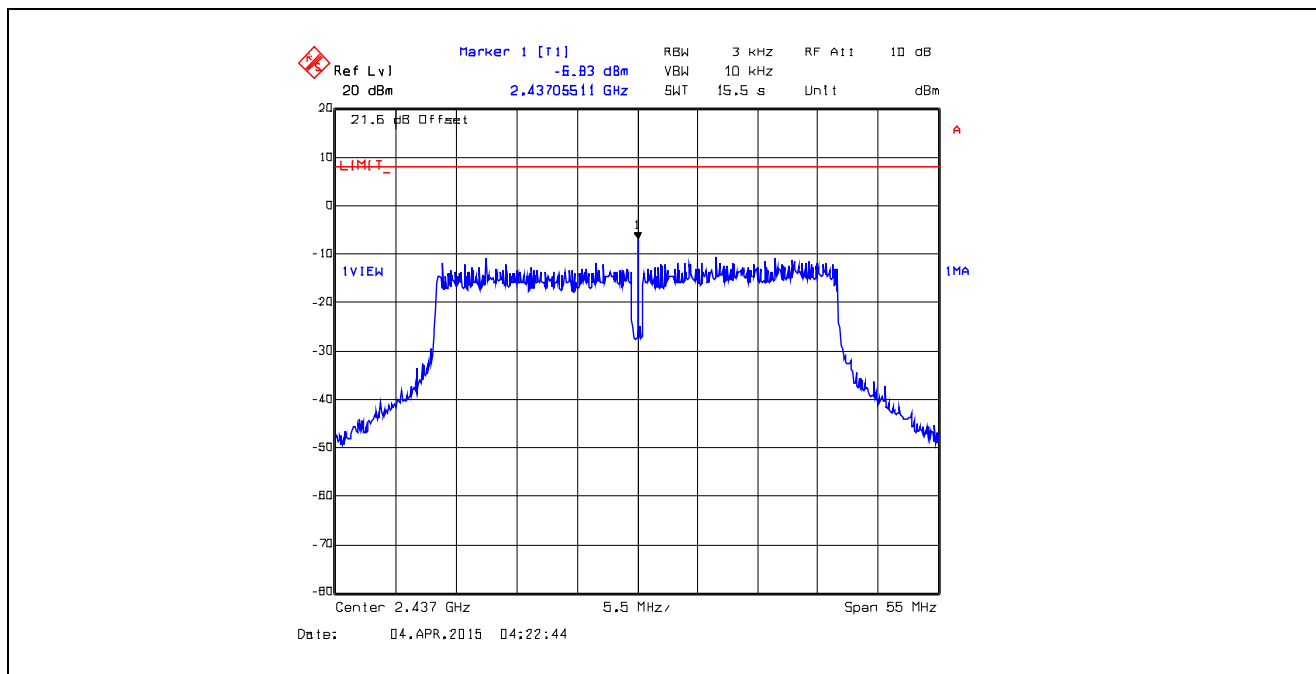
Plot 5.6.4.70. Power Spectral Density Data Rate 12, Chain # 2, Ch 6, 2437 MHz, Software Output Power Setting 17
