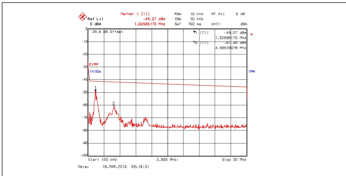
Plot 5.4.4.3.64. Conducted Spurious Emissions in Restricted Frequency Bands Chain #2 , Data Rate 11, Ch 1, 2412 MHz, Software Output Power Setting 19, 150 kHz - 30 MHz, Peak Detector
