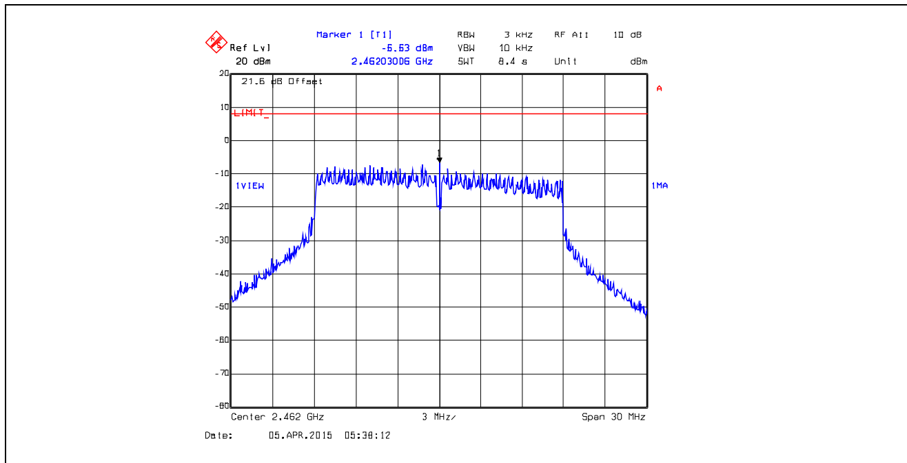
Plot 5.6.4.65. Power Spectral Density Data Rate 11, Chain # 1, Ch 11, 2462 MHz, Software Output Power Setting 19
