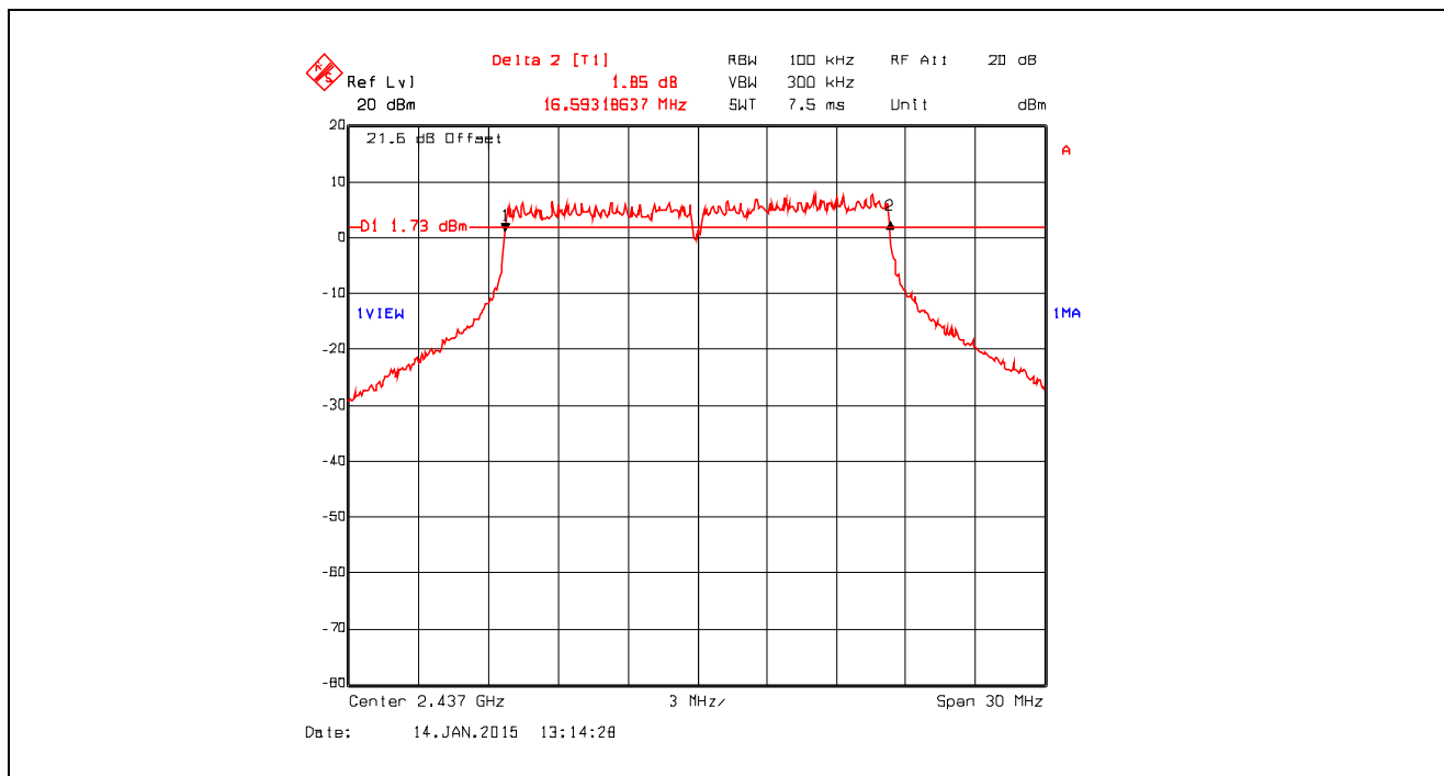
Plot 5.2.4.40. 6 dB Bandwidth, Data Rate 7, Chain # 2, Ch 6, 2437 MHz, Software Output Power Setting 18
