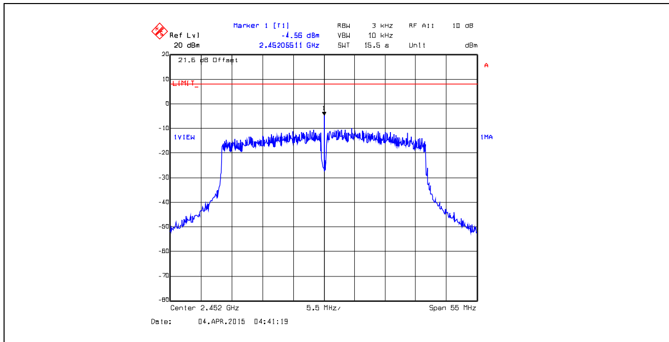
Plot 5.6.4.77. Power Spectral Density Data Rate 13, Chain # 1, Ch 9, 2452 MHz, Software Output Power Setting 17
