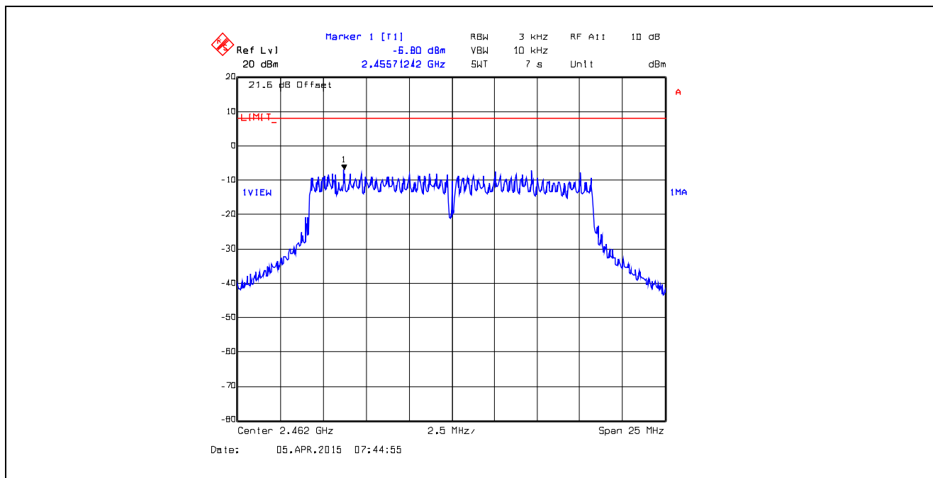
Plot 5.6.4.42. Power Spectral Density Data Rate 7, Chain # 2, Ch 11, 2462 MHz, Software Output Power Setting 18
