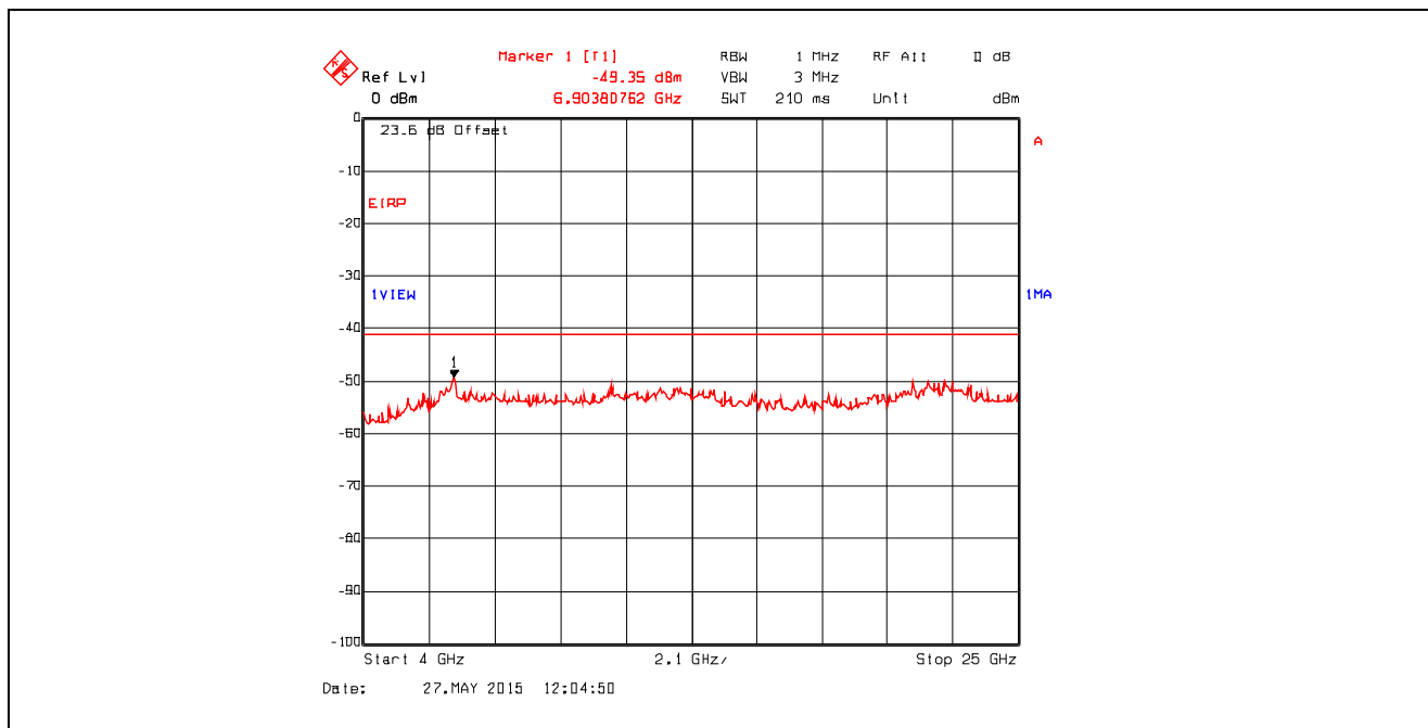
Plot 5.4.4.3.69. Conducted Spurious Emissions in Restricted Frequency Bands Chain #1 , Data Rate 11, Ch 1, 2412 MHz, Software Output Power Setting 19, 4 GHz - 25 GHz, Peak Detector
