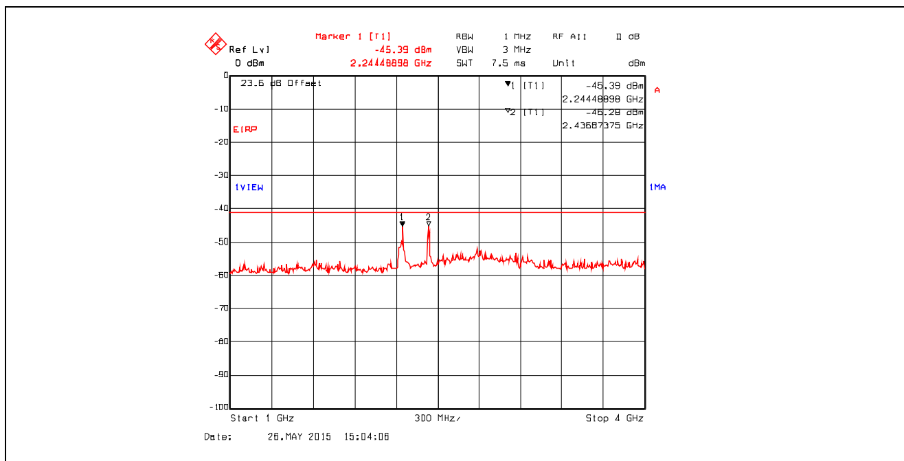
Plot 5.4.4.3.18. Conducted Spurious Emissions in Restricted Frequency Bands Chain #2 , Data Rate 3, Ch 6, 2437 MHz, Software Output Power Setting 26, 1 GHz - 4 GHz, Peak Detector
