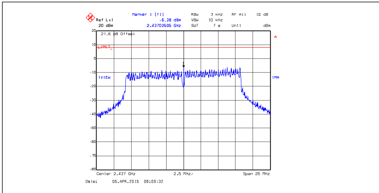
Plot 5.6.4.21. Power Spectral Density Data Rate 4, Chain # 1, Ch 6, 2437 MHz, Software Output Power Setting 18
