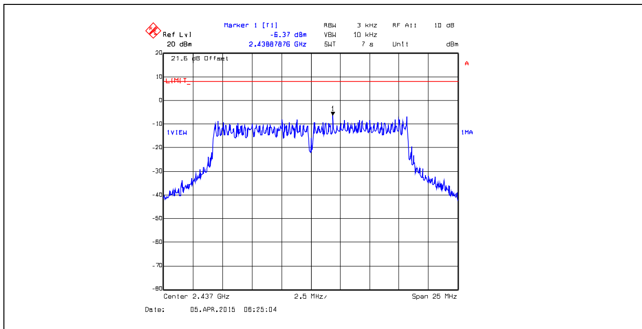
Plot 5.6.4.28. Power Spectral Density Data Rate 5, Chain # 2, Ch 6, 2437 MHz, Software Output Power Setting 18
