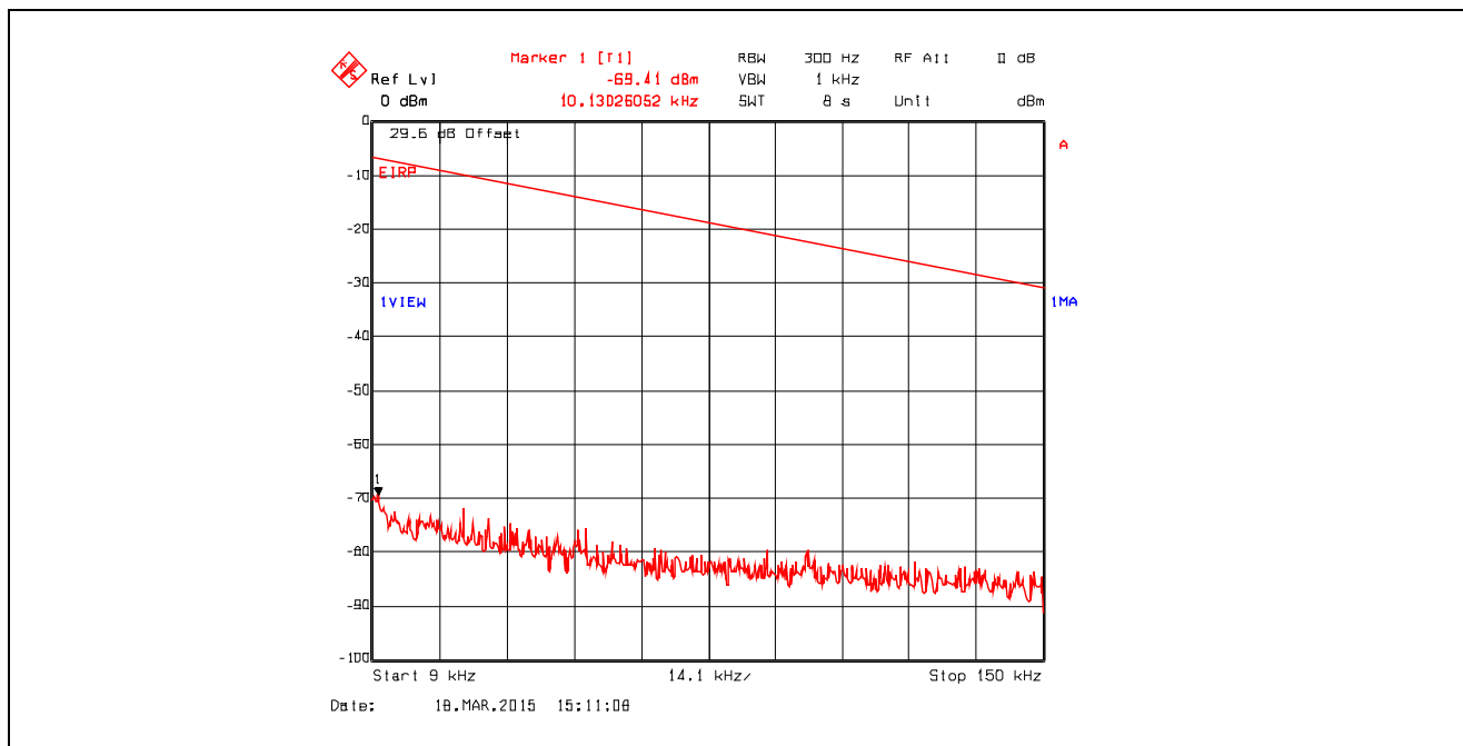
Plot 5.4.4.3.92. Conducted Spurious Emissions in Restricted Frequency Bands Chain #2 , Data Rate 15, Ch 3, 2422 MHz, Software Output Power Setting 17, 9 kHz - 150 kHz, Peak Detector
