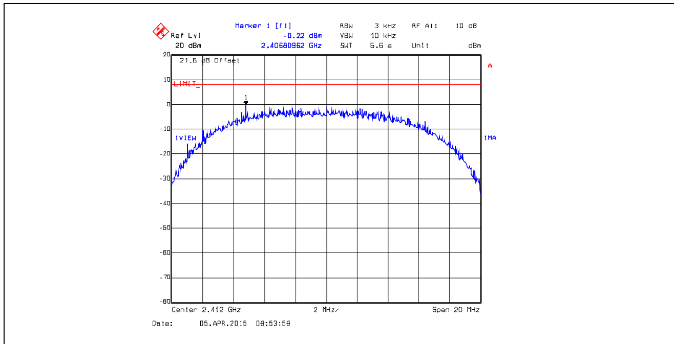
Plot 5.6.4.13. Power Spectral Density Data Rate 3, Chain # 1, Ch 1, 2412 MHz, Software Output Power Setting 26
