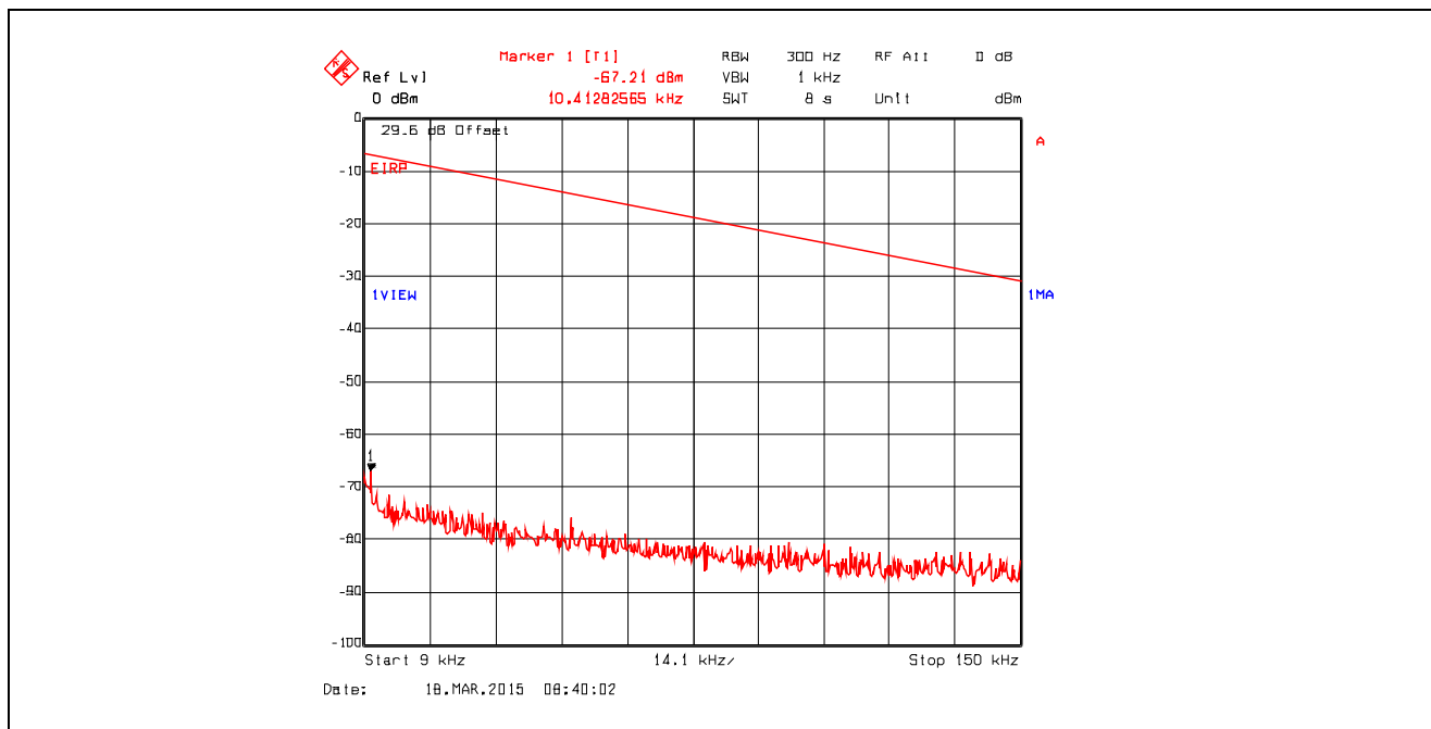
Plot 5.4.4.3.62. Conducted Spurious Emissions in Restricted Frequency Bands Chain #2 , Data Rate 11, Ch 1, 2412 MHz, Software Output Power Setting 19, 9 kHz - 150 kHz, Peak Detector
