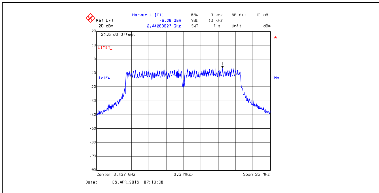
Plot 5.6.4.34. Power Spectral Density Data Rate 6, Chain # 2, Ch 6, 2437 MHz, Software Output Power Setting 18
