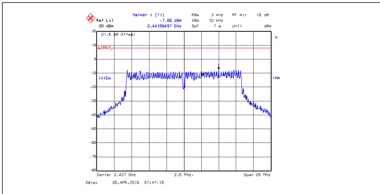
Plot 5.6.4.40. Power Spectral Density Data Rate 7, Chain # 2, Ch 6, 2437 MHz, Software Output Power Setting 18
