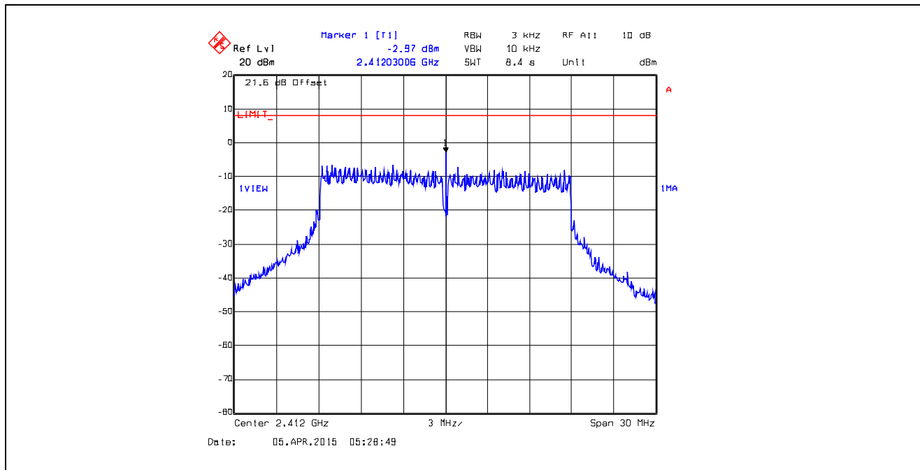
Plot 5.6.4.55. Power Spectral Density Data Rate 10, Chain # 1, Ch 1, 2412 MHz, Software Output Power Setting 19
