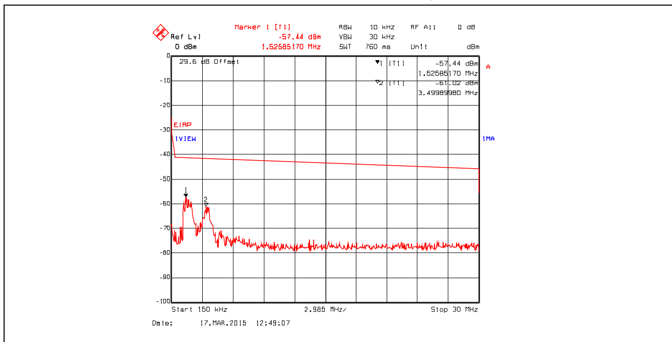
Plot 5.4.4.3.34. Conducted Spurious Emissions in Restricted Frequency Bands Chain #2 , Data Rate 7, Ch 1, 2412 MHz, Software Output Power Setting 18, 150 kHz - 30 MHz, Peak Detector
