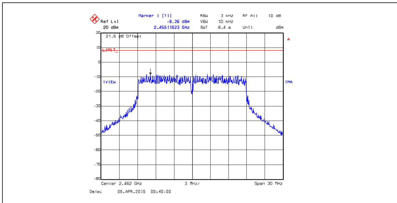
Plot 5.6.4.66. Power Spectral Density Data Rate 11, Chain # 2, Ch 11, 2462 MHz, Software Output Power Setting 19
