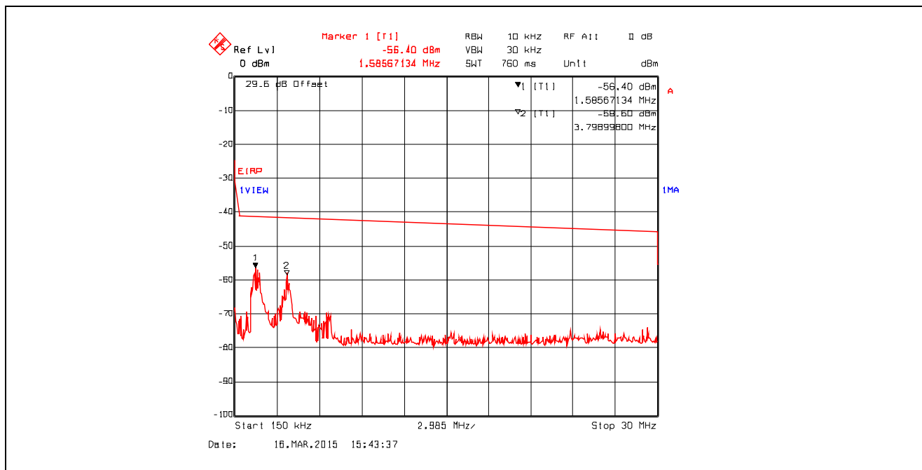
Plot 5.4.4.3.3. Conducted Spurious Emissions in Restricted Frequency Bands Chain #1 , Data Rate 3, Ch 1, 2412 MHz, Software Output Power Setting 26, 150 kHz - 30 MHz, Peak Detector
