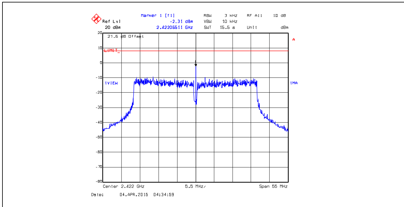
Plot 5.6.4.73. Power Spectral Density Data Rate 13, Chain # 1, Ch 3, 2422 MHz, Software Output Power Setting 17
