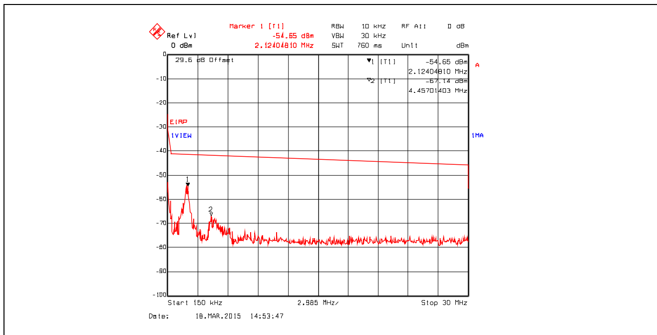
Plot 5.4.4.3.103. Conducted Spurious Emissions in Restricted Frequency Bands Chain #1 , Data Rate 15, Ch 6, 2437 MHz, Software Output Power Setting 17, 150 kHz - 30 MHz, Peak Detector
