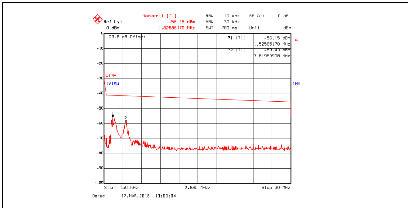
Plot 5.4.4.3.54. Conducted Spurious Emissions in Restricted Frequency Bands Chain #2 , Data Rate 7, Ch 11, 2462 MHz, Software Output Power Setting 18, 150 kHz - 30 MHz, Peak Detector
