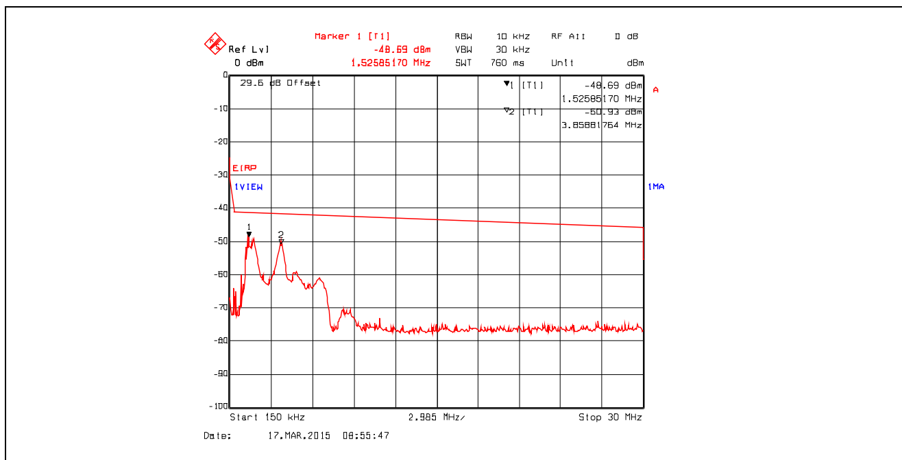
Plot 5.4.4.3.14. Conducted Spurious Emissions in Restricted Frequency Bands Chain #2 , Data Rate 3, Ch 6, 2437 MHz, Software Output Power Setting 26, 150 kHz - 30 MHz, Peak Detector
