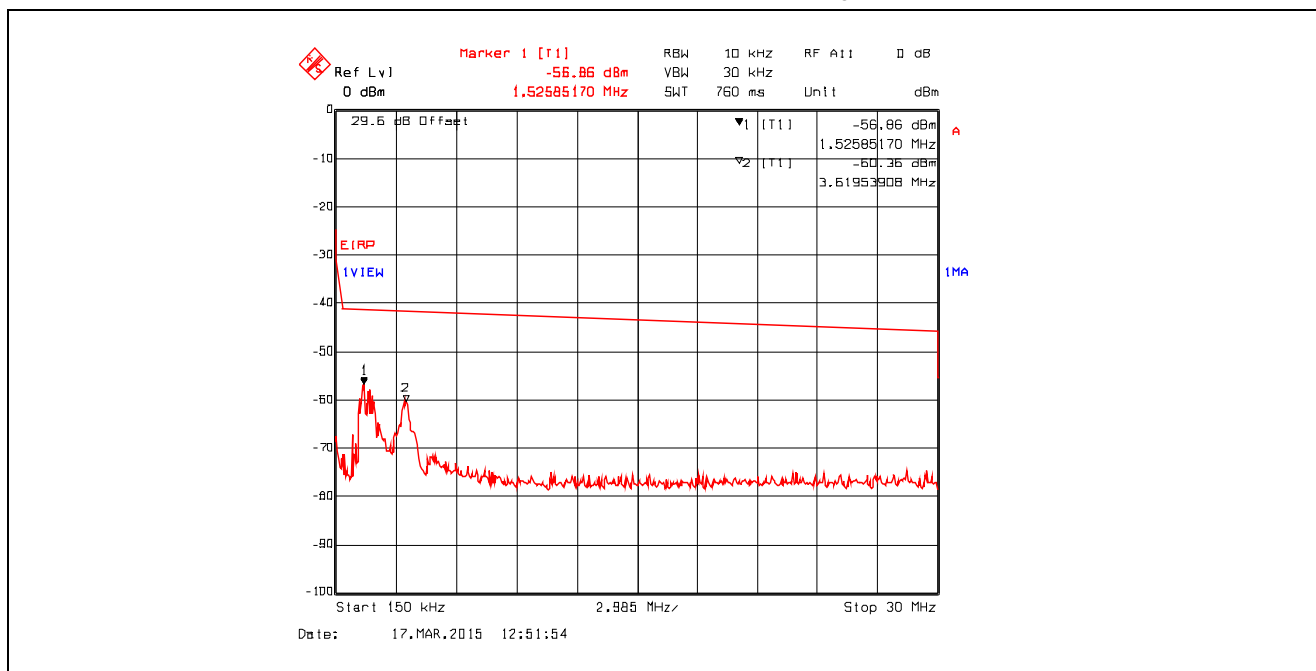
Plot 5.4.4.3.44. Conducted Spurious Emissions in Restricted Frequency Bands Chain #2 , Data Rate 7, Ch 6, 2437 MHz, Software Output Power Setting 18, 150 kHz - 30 MHz, Peak Detector
