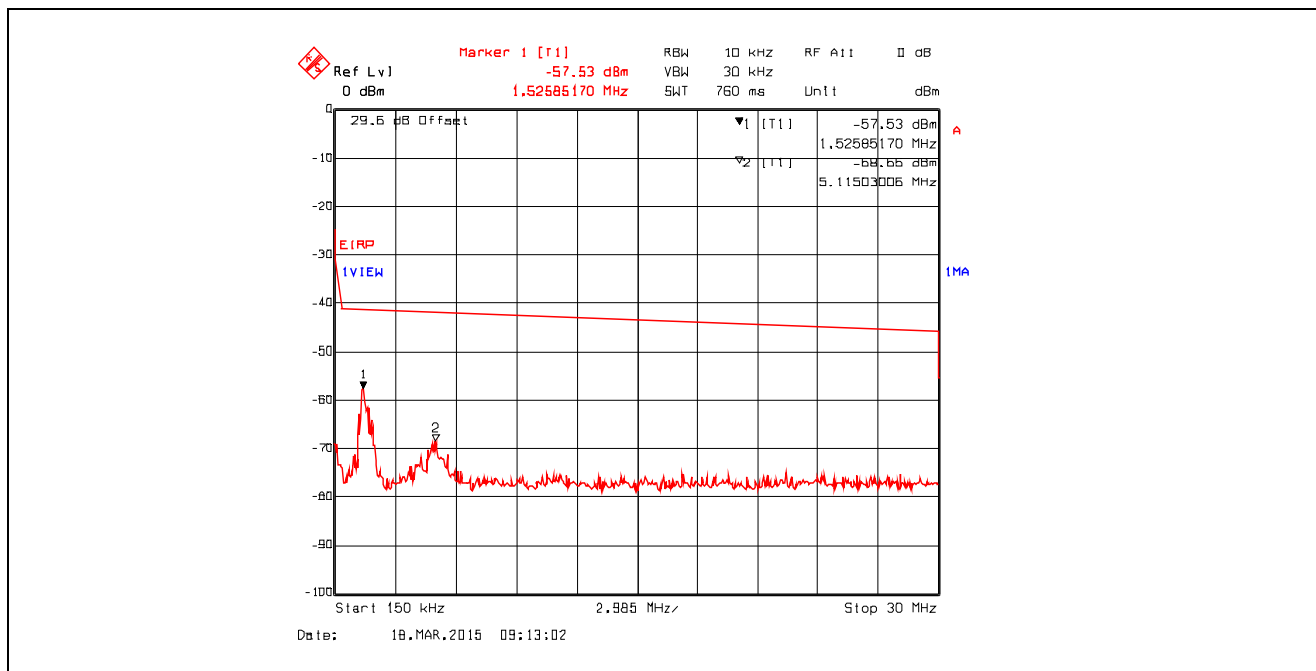
Plot 5.4.4.3.83. Conducted Spurious Emissions in Restricted Frequency Bands Chain #1 , Data Rate 11, Ch 11, 2462 MHz, Software Output Power Setting 19, 150 kHz - 30 MHz, Peak Detector
