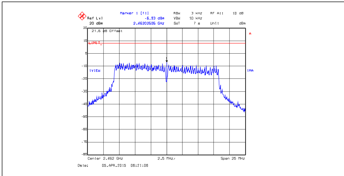
Plot 5.6.4.29. Power Spectral Density Data Rate 5, Chain # 1, Ch 11, 2462 MHz, Software Output Power Setting 18
