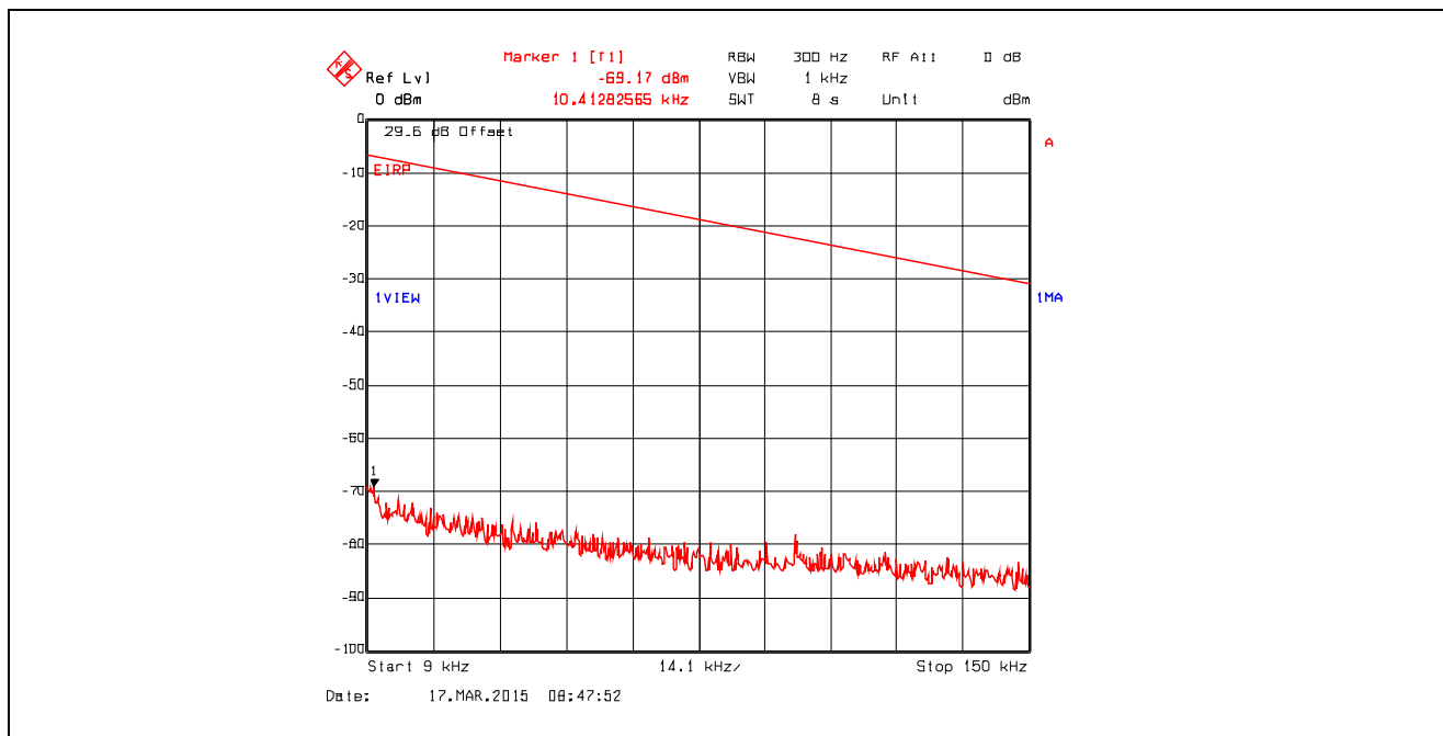
Plot 5.4.4.3.22. Conducted Spurious Emissions in Restricted Frequency Bands Chain #2 , Data Rate 3, Ch 11, 2462 MHz, Software Output Power Setting 26, 9 kHz - 150 kHz, Peak Detector
