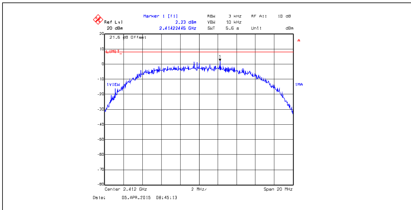
Plot 5.6.4.14. Power Spectral Density Data Rate 3, Chain # 2, Ch 1, 2412 MHz, Software Output Power Setting 26
