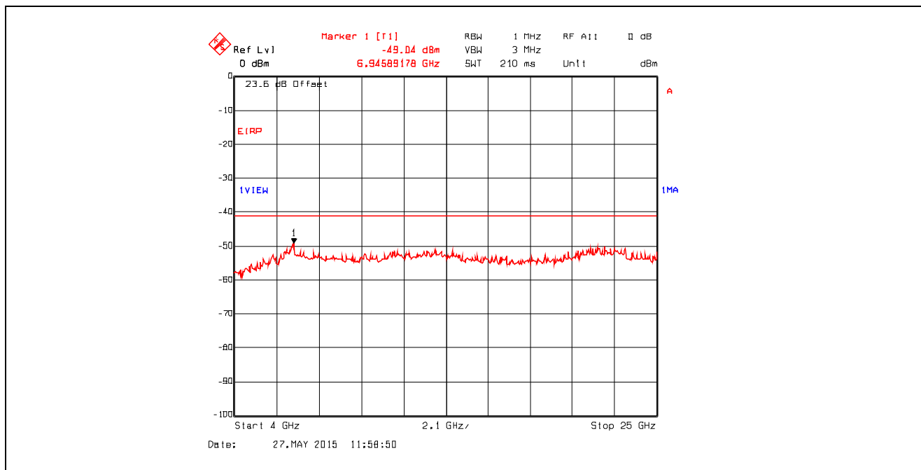
Plot 5.4.4.3.79. Conducted Spurious Emissions in Restricted Frequency Bands Chain #1 , Data Rate 11, Ch 6, 2437 MHz, Software Output Power Setting 19, 4 GHz - 25 GHz, Peak Detector
