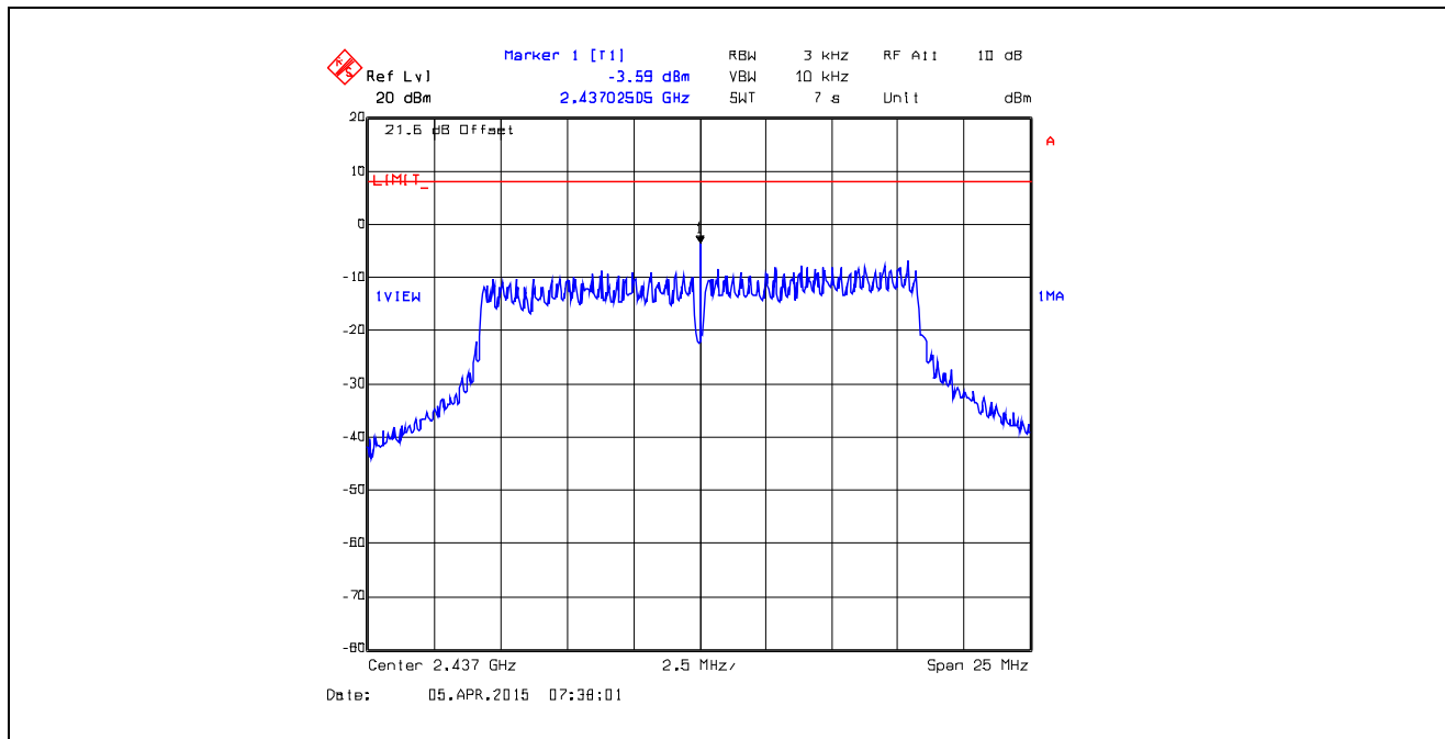
Plot 5.6.4.39. Power Spectral Density Data Rate 7, Chain # 1, Ch 6, 2437 MHz, Software Output Power Setting 18
