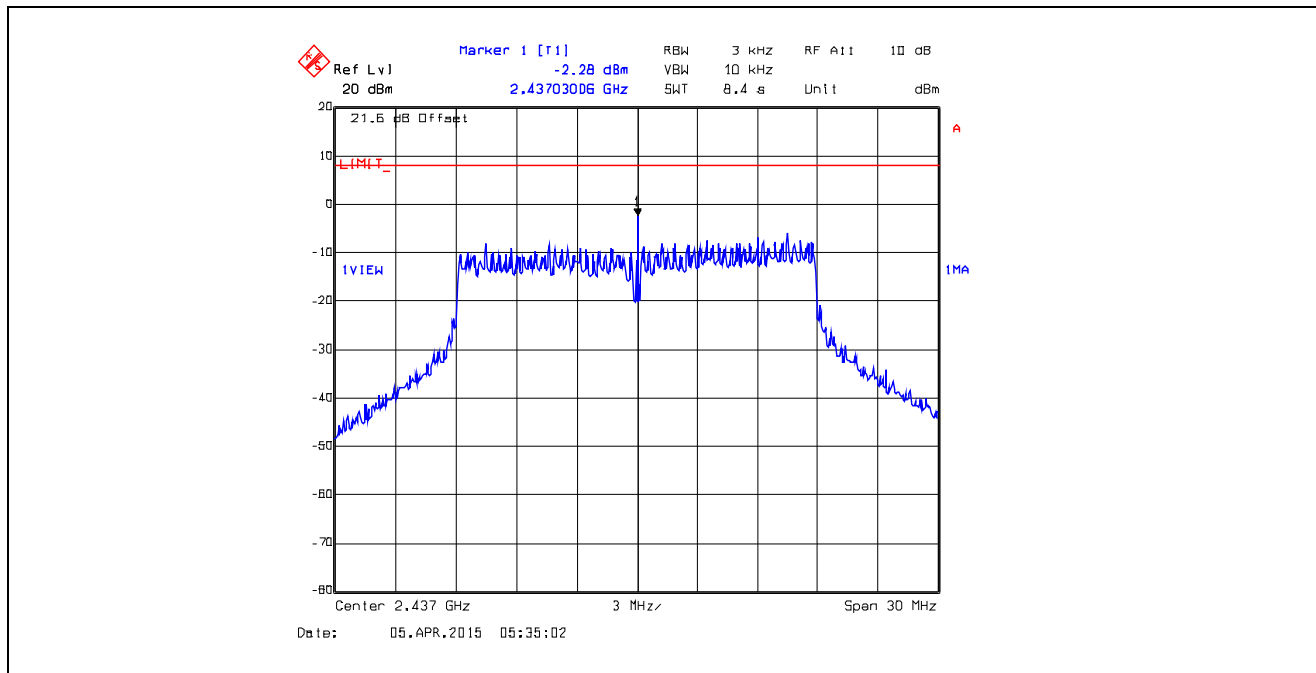
Plot 5.6.4.63. Power Spectral Density Data Rate 11, Chain # 1, Ch 6, 2437 MHz, Software Output Power Setting 19
