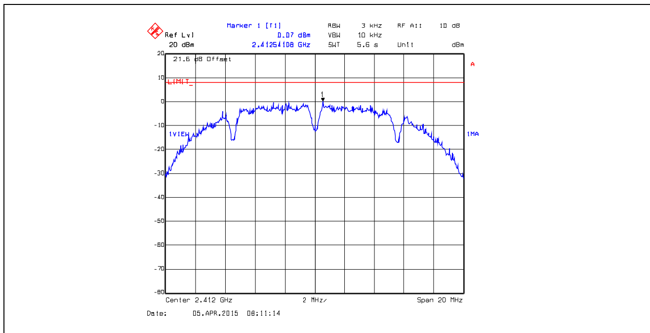
Plot 5.6.4.2. Power Spectral Density Data Rate 1, Chain # 2, Ch 1, 2412 MHz, Software Output Power Setting 26
