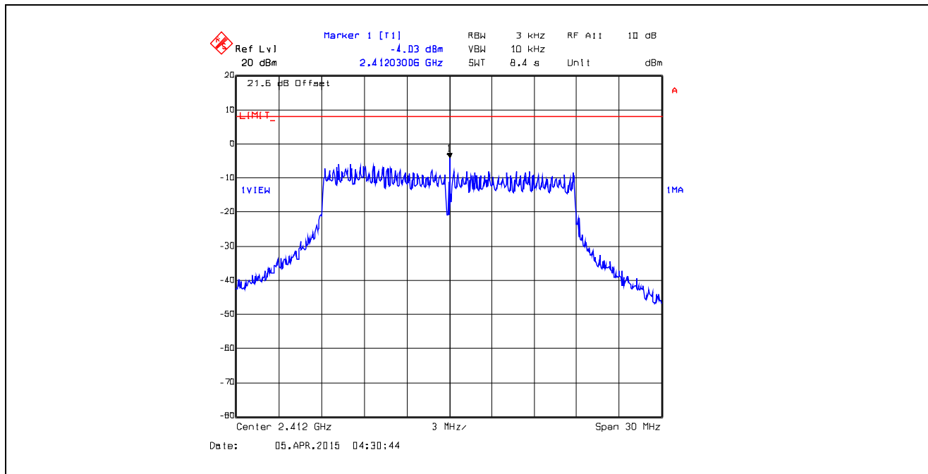
Plot 5.6.4.43. Power Spectral Density Data Rate 8, Chain # 1, Ch 1, 2412 MHz, Software Output Power Setting 19
