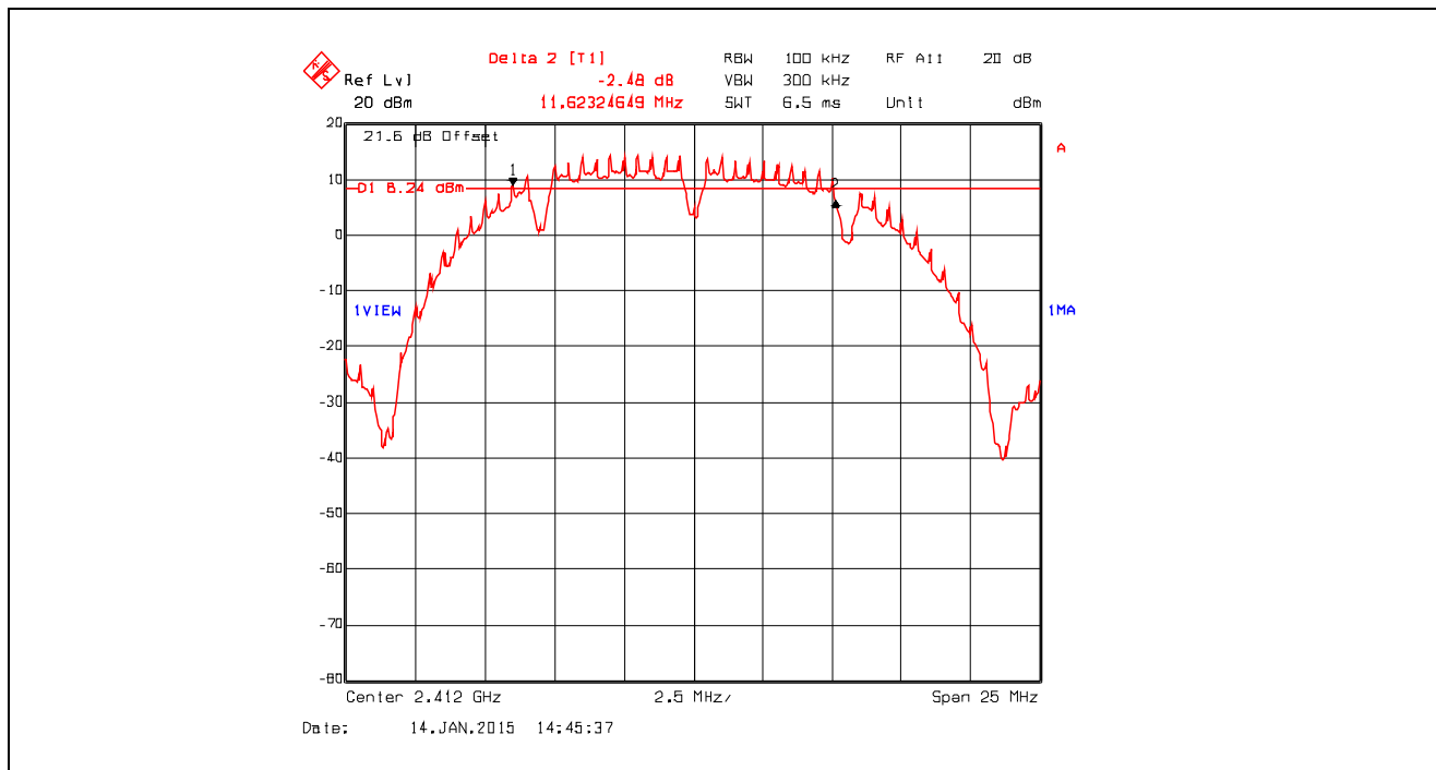
Plot 5.2.4.2. 6 dB Bandwidth, Data Rate 1, Chain # 2, Ch 1, 2412 MHz, Software Output Power Setting 26
