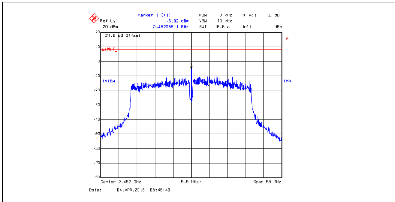
Plot 5.6.4.89. Power Spectral Density Data Rate 15, Chain # 1, Ch 9, 2452 MHz, Software Output Power Setting 17
