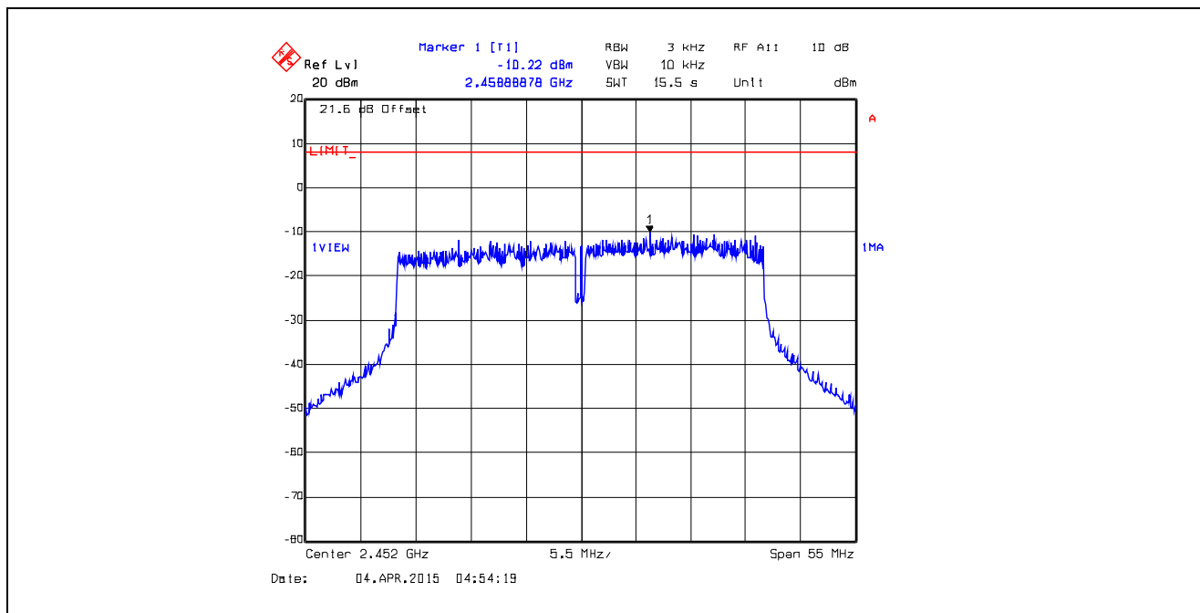
Plot 5.6.4.78. Power Spectral Density Data Rate 13, Chain # 2, Ch 9, 2452 MHz, Software Output Power Setting 17
