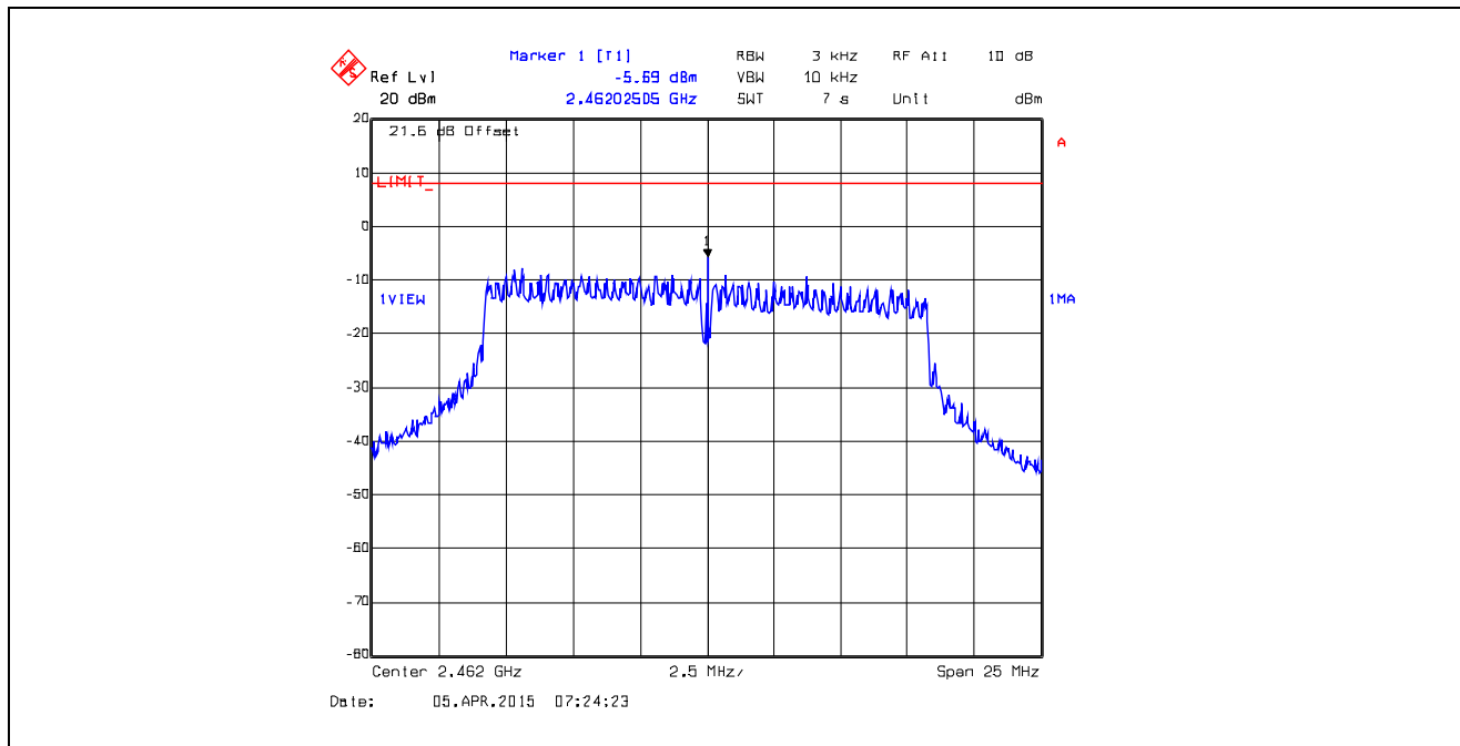
Plot 5.6.4.35. Power Spectral Density Data Rate 6, Chain # 1, Ch 11, 2462 MHz, Software Output Power Setting 18
