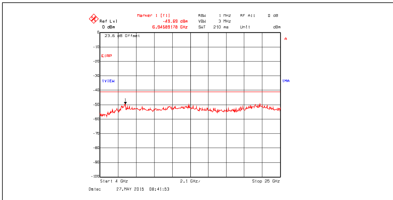
Plot 5.4.4.3.59. Conducted Spurious Emissions in Restricted Frequency Bands Chain #1 , Data Rate 7, Ch 11, 2462 MHz, Software Output Power Setting 18, 4 GHz - 25 GHz, Peak Detector
