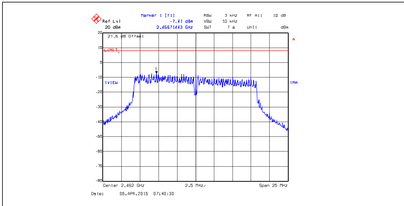
Plot 5.6.4.41. Power Spectral Density Data Rate 7, Chain # 1, Ch 11, 2462 MHz, Software Output Power Setting 18
