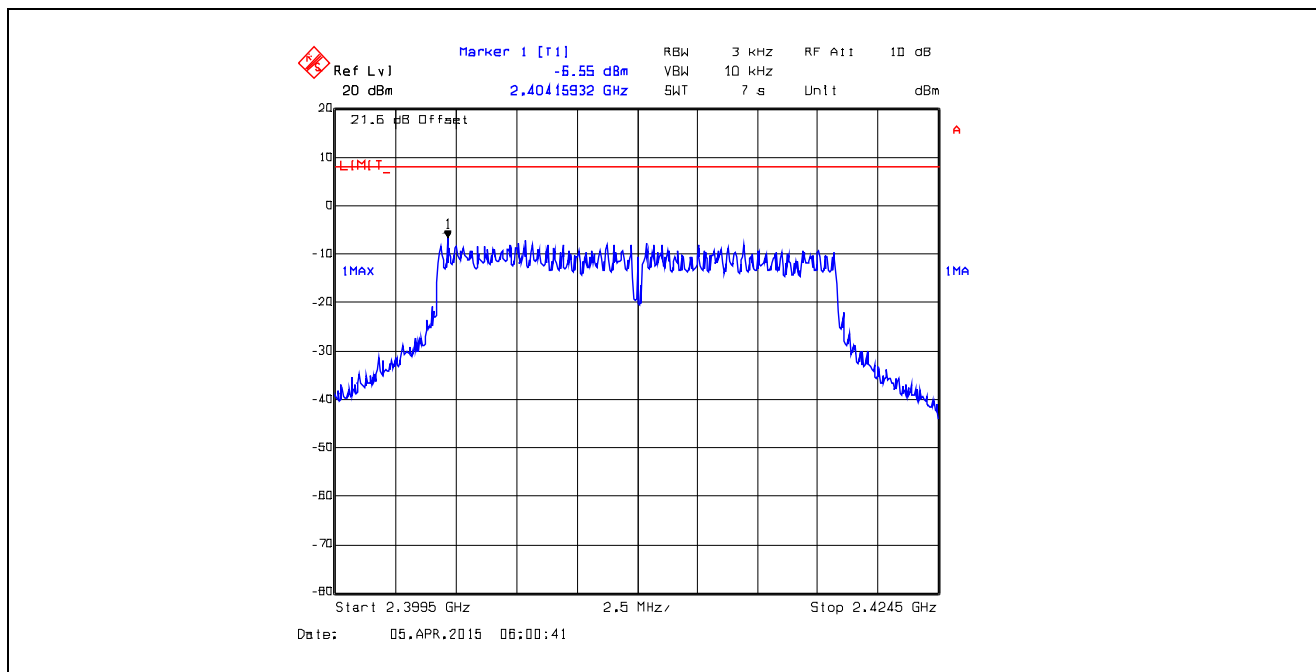
Plot 5.6.4.20. Power Spectral Density Data Rate 4, Chain # 2, Ch 1, 2412 MHz, Software Output Power Setting 18
