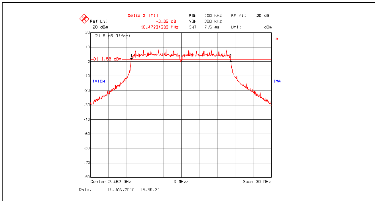
Plot 5.2.4.24. 6 dB Bandwidth, Data Rate 4, Chain # 2, Ch 11, 2462 MHz, Software Output Power Setting 18
