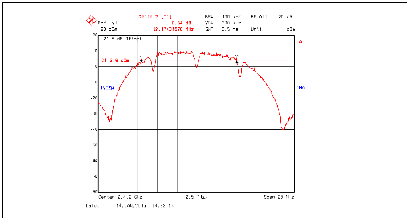
Plot 5.2.4.7. 6 dB Bandwidth, Data Rate 2, Chain # 1, Ch 1, 2412 MHz, Software Output Power Setting 26
