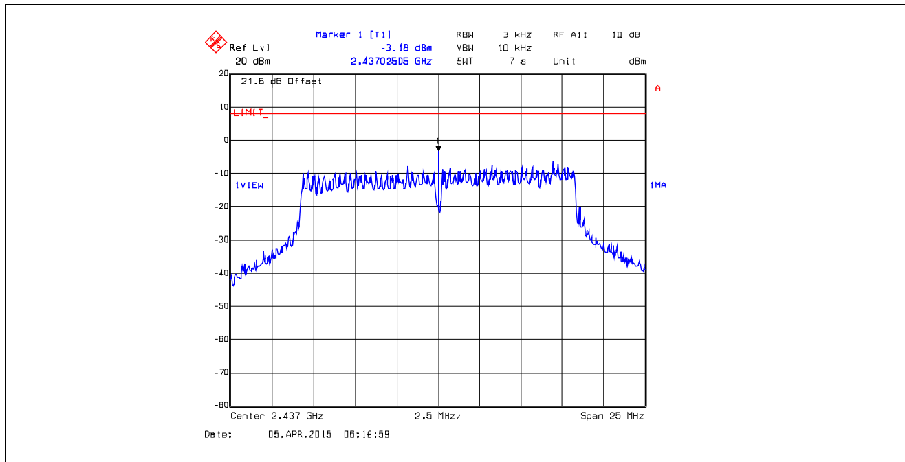
Plot 5.6.4.27. Power Spectral Density Data Rate 5, Chain # 1, Ch 6, 2437 MHz, Software Output Power Setting 18
