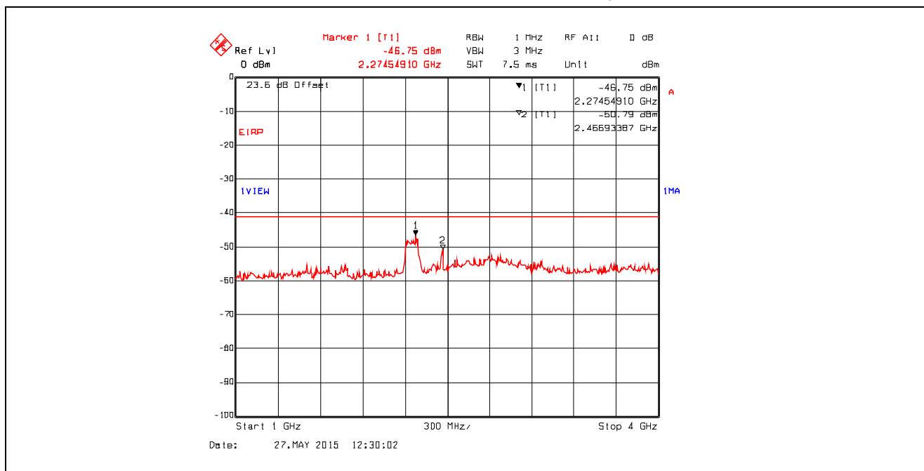
Plot 5.4.4.3.118. Conducted Spurious Emissions in Restricted Frequency Bands Chain #2 , Data Rate 15, Ch 9, 2452 MHz, Software Output Power Setting 17, 1 GHz - 4 GHz, Peak Detector
