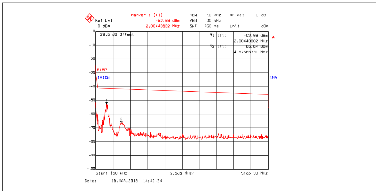
Plot 5.4.4.3.94. Conducted Spurious Emissions in Restricted Frequency Bands Chain #2 , Data Rate 15, Ch 3, 2422 MHz, Software Output Power Setting 17, 150 kHz - 30 MHz, Peak Detector
