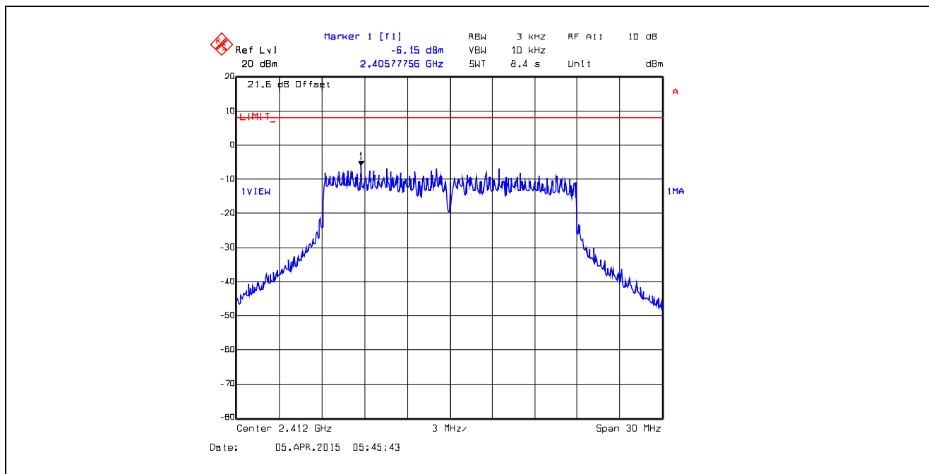
Plot 5.6.4.62. Power Spectral Density Data Rate 11, Chain # 2, Ch 1, 2412 MHz, Software Output Power Setting 19
