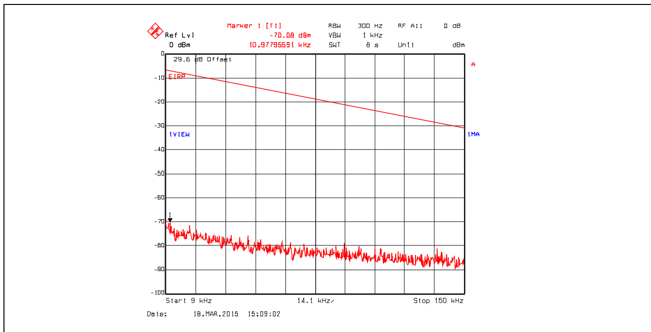
Plot 5.4.4.3.91. Conducted Spurious Emissions in Restricted Frequency Bands Chain #1 , Data Rate 15, Ch 3, 2422 MHz, Software Output Power Setting 17, 9 kHz - 150 kHz, Peak Detector
