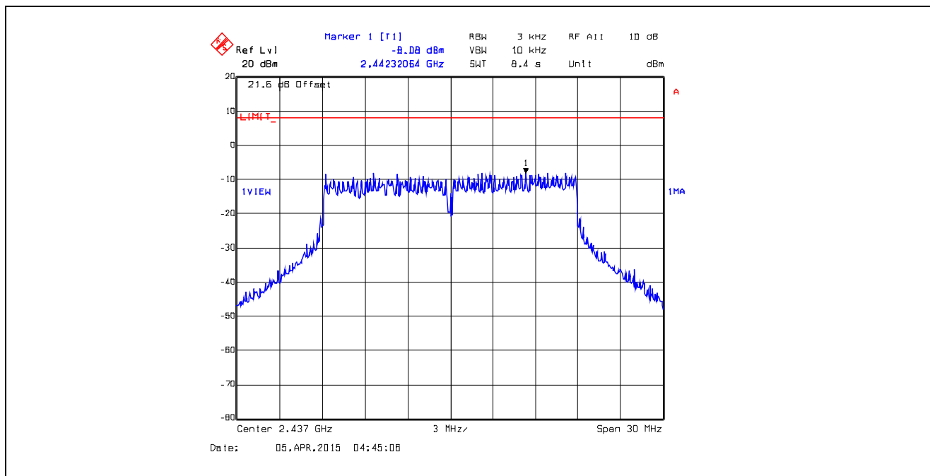
Plot 5.6.4.52. Power Spectral Density Data Rate 9, Chain # 2, Ch 6, 2437 MHz, Software Output Power Setting 19
