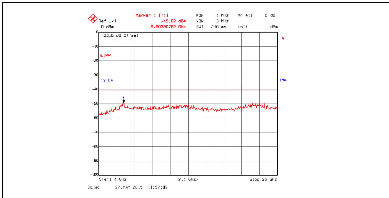
Plot 5.4.4.3.89. Conducted Spurious Emissions in Restricted Frequency Bands Chain #1 , Data Rate 11, Ch 11, 2462 MHz, Software Output Power Setting 19, 4 GHz - 25 GHz, Peak Detector
