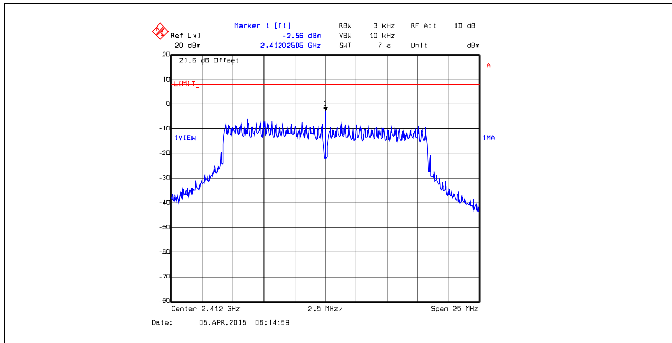
Plot 5.6.4.25. Power Spectral Density Data Rate 5, Chain # 1, Ch 1, 2412 MHz, Software Output Power Setting 18
