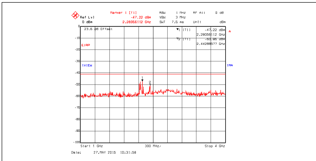
Plot 5.4.4.3.78. Conducted Spurious Emissions in Restricted Frequency Bands Chain #2 , Data Rate 11, Ch 6, 2437 MHz, Software Output Power Setting 19, 1 GHz - 4 GHz, Peak Detector
