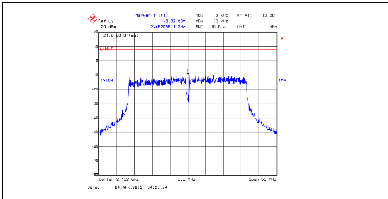
Plot 5.6.4.72. Power Spectral Density Data Rate 12, Chain # 2, Ch 9, 2452 MHz, Software Output Power Setting 17
