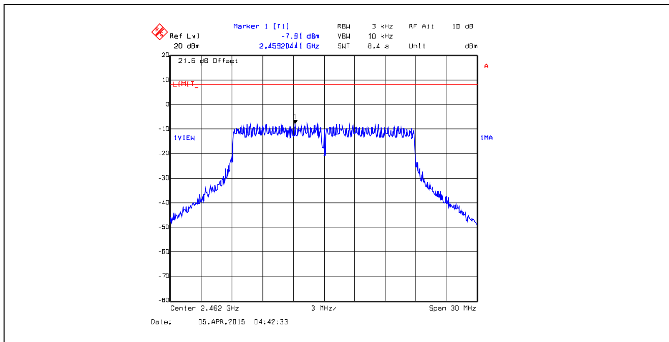
Plot 5.6.4.54. Power Spectral Density Data Rate 9, Chain # 2, Ch 11, 2462 MHz, Software Output Power Setting 19
