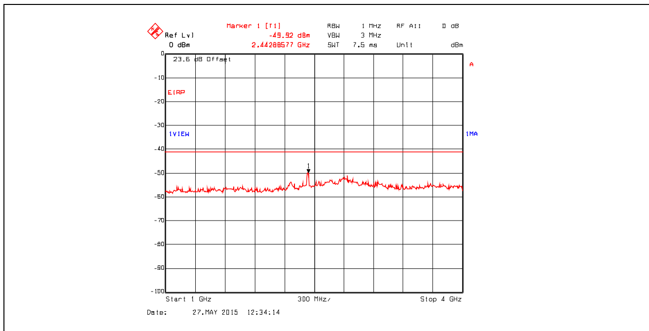
Plot 5.4.4.3.107. Conducted Spurious Emissions in Restricted Frequency Bands Chain #1 , Data Rate 15, Ch 6, 2437 MHz, Software Output Power Setting 17, 1 GHz - 4 GHz, Peak Detector
