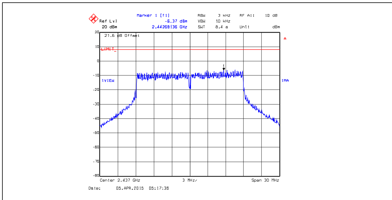
Plot 5.6.4.58. Power Spectral Density Data Rate 10, Chain # 2, Ch 6, 2437 MHz, Software Output Power Setting 19
