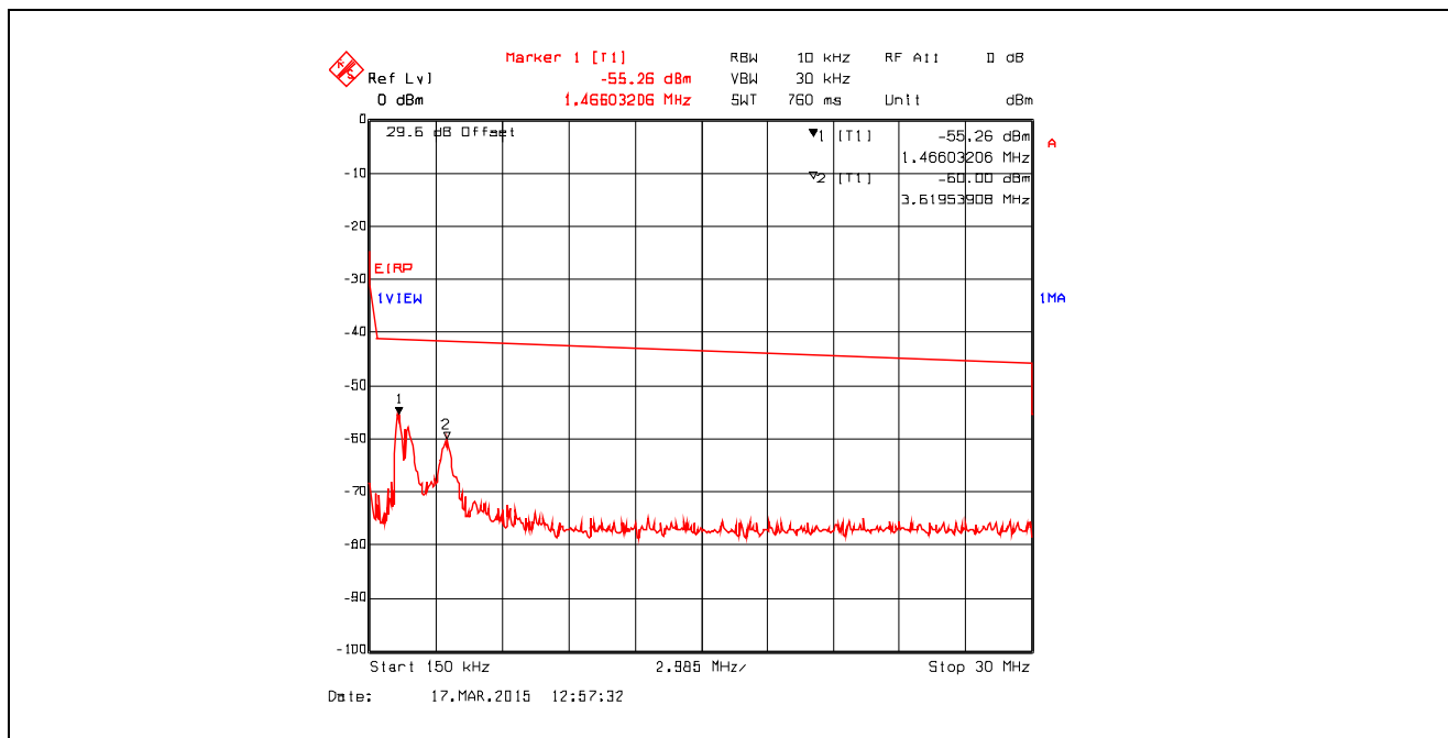
Plot 5.4.4.3.53. Conducted Spurious Emissions in Restricted Frequency Bands Chain #1 , Data Rate 7, Ch 11, 2462 MHz, Software Output Power Setting 18, 150 kHz - 30 MHz, Peak Detector
