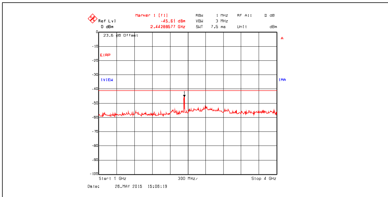
Plot 5.4.4.3.17. Conducted Spurious Emissions in Restricted Frequency Bands Chain #1 , Data Rate 3, Ch 6, 2437 MHz, Software Output Power Setting 26, 1 GHz - 4 GHz, Peak Detector
