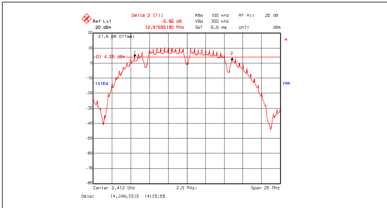
Plot 5.2.4.1. 6 dB Bandwidth, Data Rate 1, Chain # 1, Ch 1, 2412 MHz, Software Output Power Setting 26
