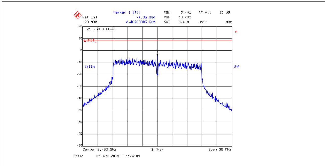
Plot 5.6.4.59. Power Spectral Density Data Rate 10, Chain # 1, Ch 11, 2462 MHz, Software Output Power Setting 19
