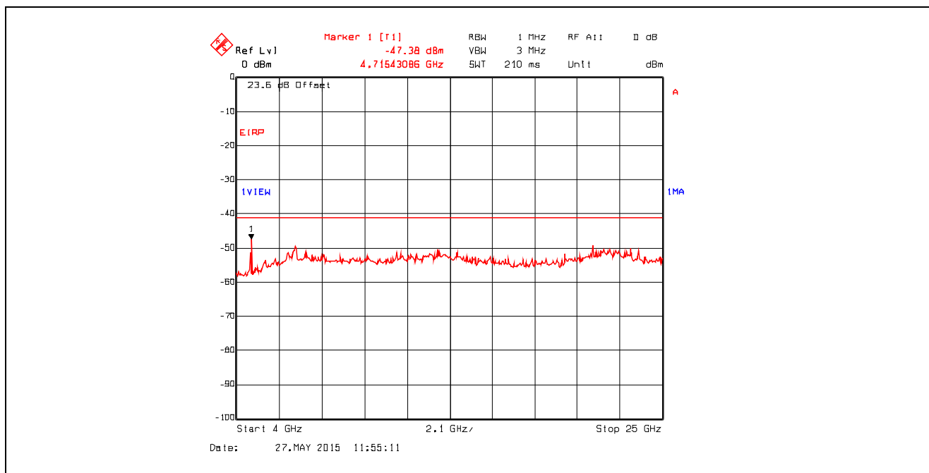
Plot 5.4.4.3.90. Conducted Spurious Emissions in Restricted Frequency Bands Chain #2 , Data Rate 11, Ch 11, 2462 MHz, Software Output Power Setting 19, 4 GHz - 25 GHz, Peak Detector
