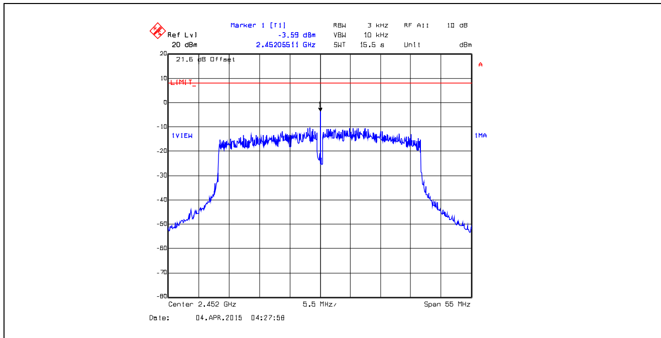
Plot 5.6.4.71. Power Spectral Density Data Rate 12, Chain # 1, Ch 9, 2452 MHz, Software Output Power Setting 17
