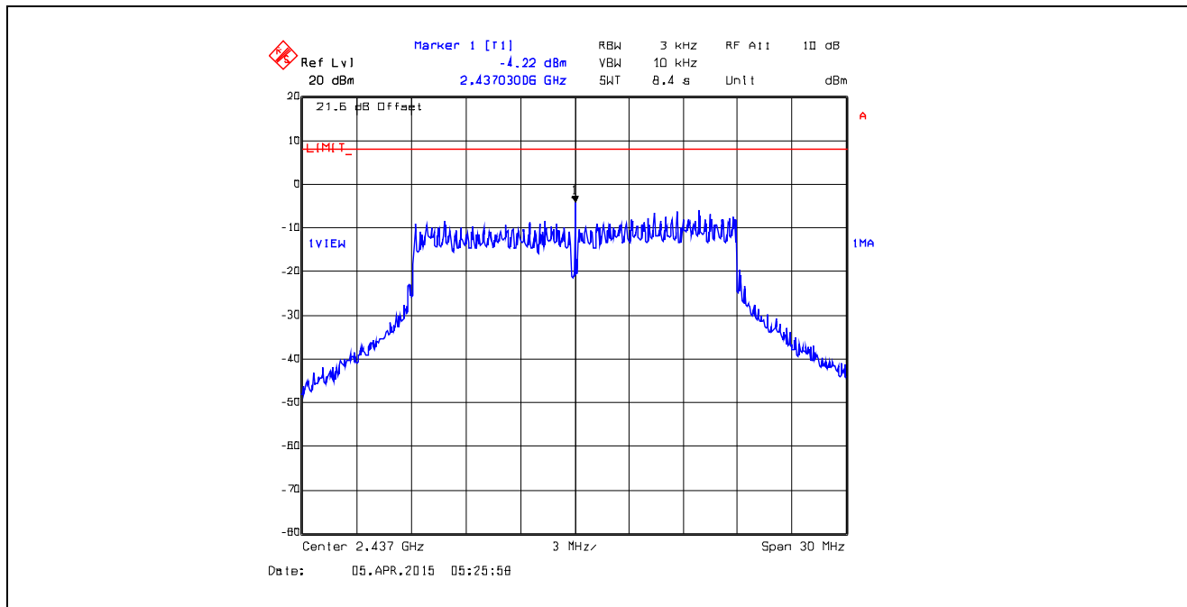
Plot 5.6.4.57. Power Spectral Density Data Rate 10, Chain # 1, Ch 6, 2437 MHz, Software Output Power Setting 19
