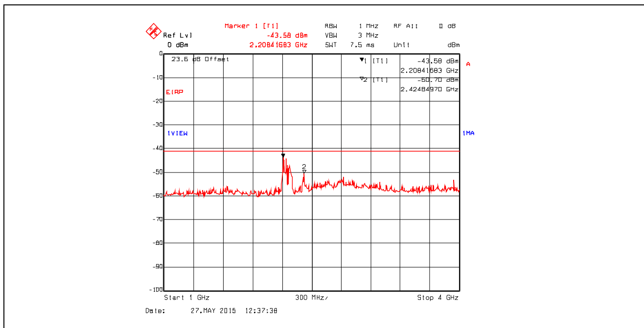
Plot 5.4.4.3.98. Conducted Spurious Emissions in Restricted Frequency Bands Chain #2 , Data Rate 15, Ch 3, 2422 MHz, Software Output Power Setting 17, 1 GHz - 4 GHz, Peak Detector
