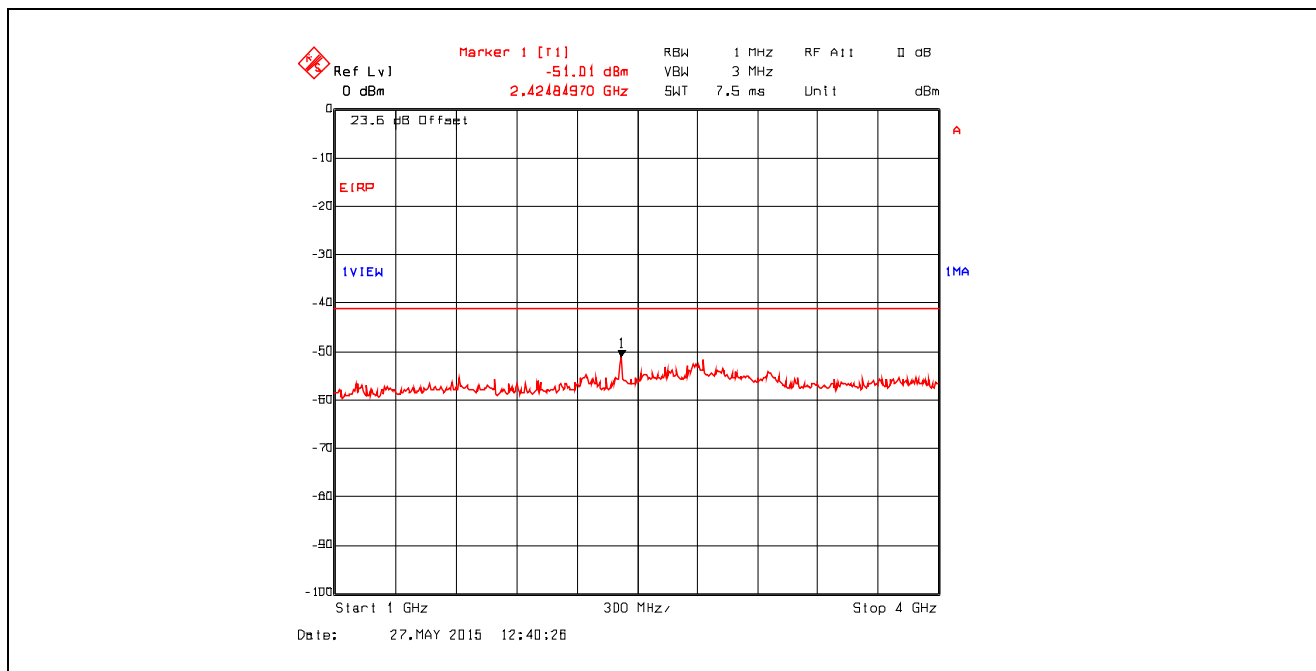
Plot 5.4.4.3.97. Conducted Spurious Emissions in Restricted Frequency Bands Chain #1 , Data Rate 15, Ch 3, 2422 MHz, Software Output Power Setting 17, 1 GHz - 4 GHz, Peak Detector
