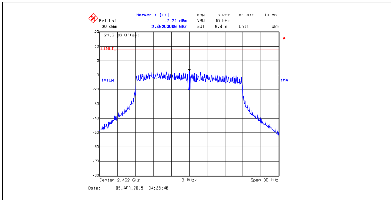
Plot 5.6.4.47. Power Spectral Density Data Rate 8, Chain # 1, Ch 11, 2462 MHz, Software Output Power Setting 19
