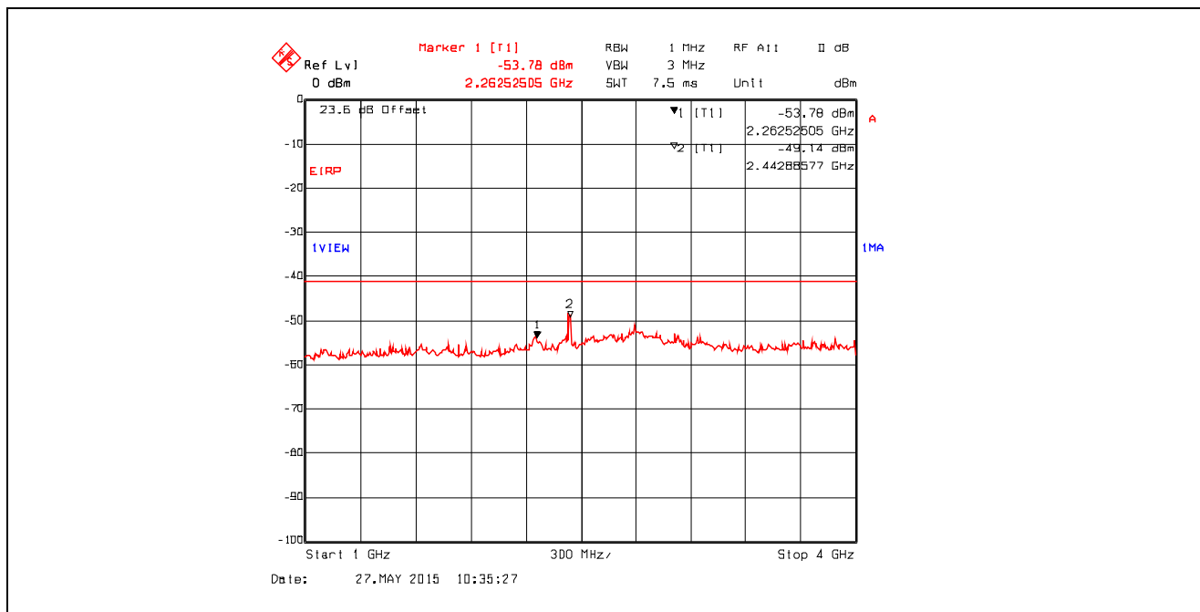
Plot 5.4.4.3.77. Conducted Spurious Emissions in Restricted Frequency Bands Chain #1 , Data Rate 11, Ch 6, 2437 MHz, Software Output Power Setting 19, 1 GHz - 4 GHz, Peak Detector
