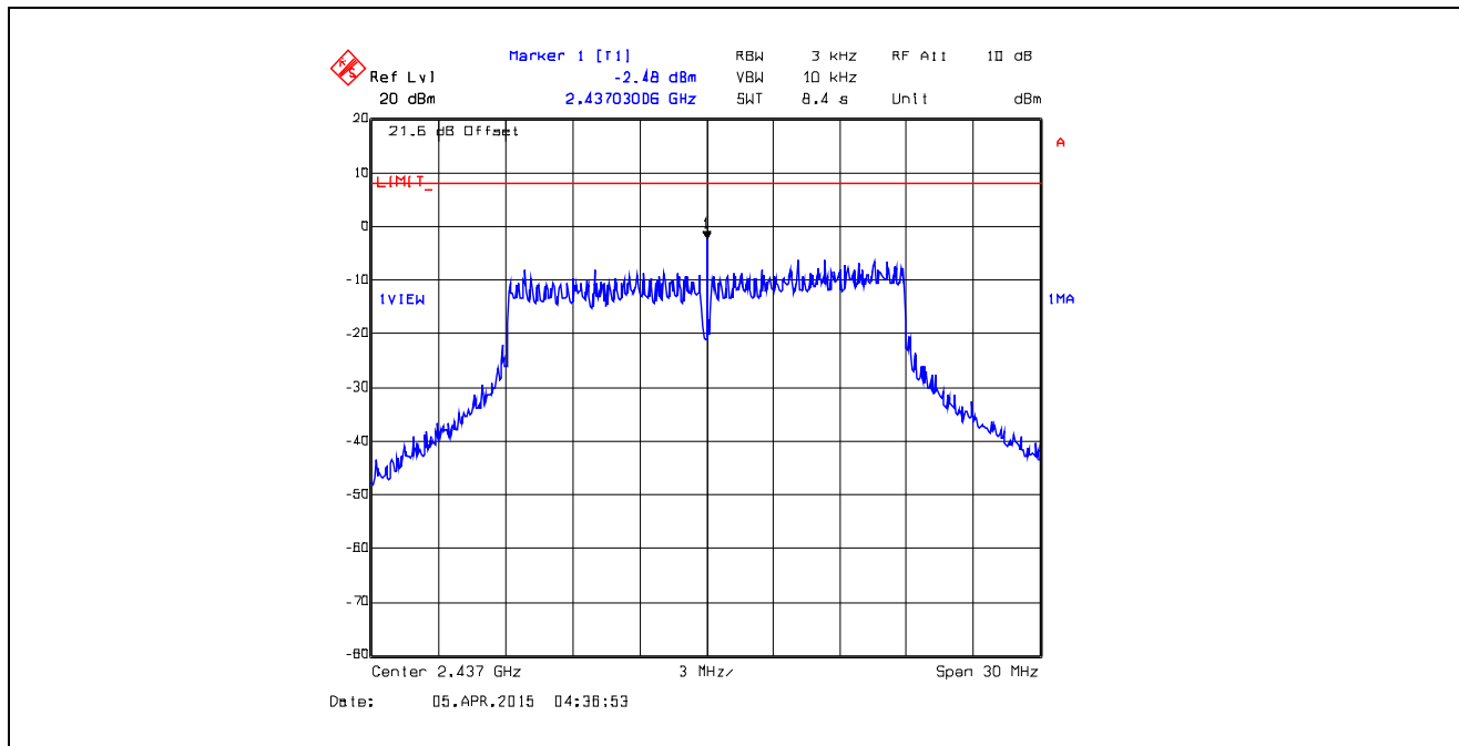
Plot 5.6.4.51. Power Spectral Density Data Rate 9, Chain # 1, Ch 6, 2437 MHz, Software Output Power Setting 19
