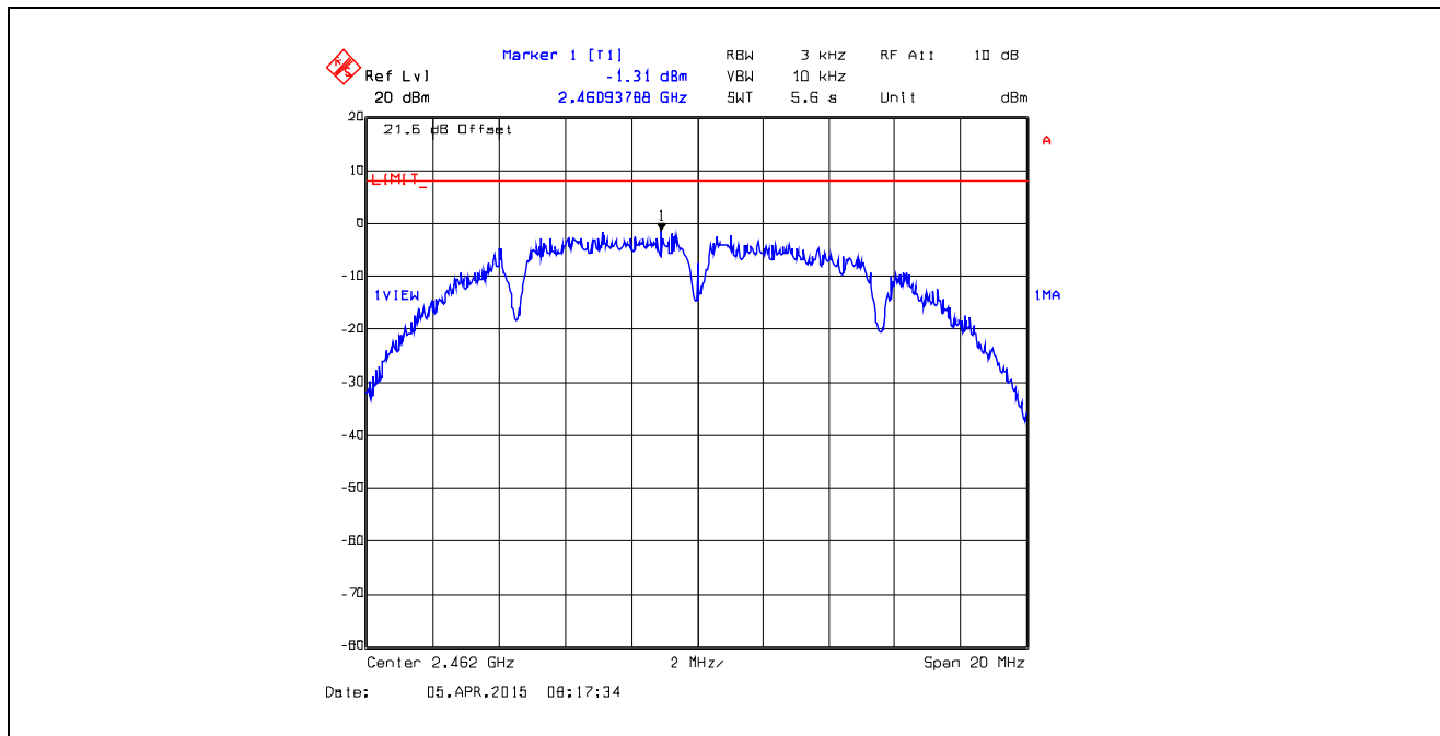
Plot 5.6.4.5. Power Spectral Density Data Rate 1, Chain # 1, Ch 11, 2462 MHz, Software Output Power Setting 26
