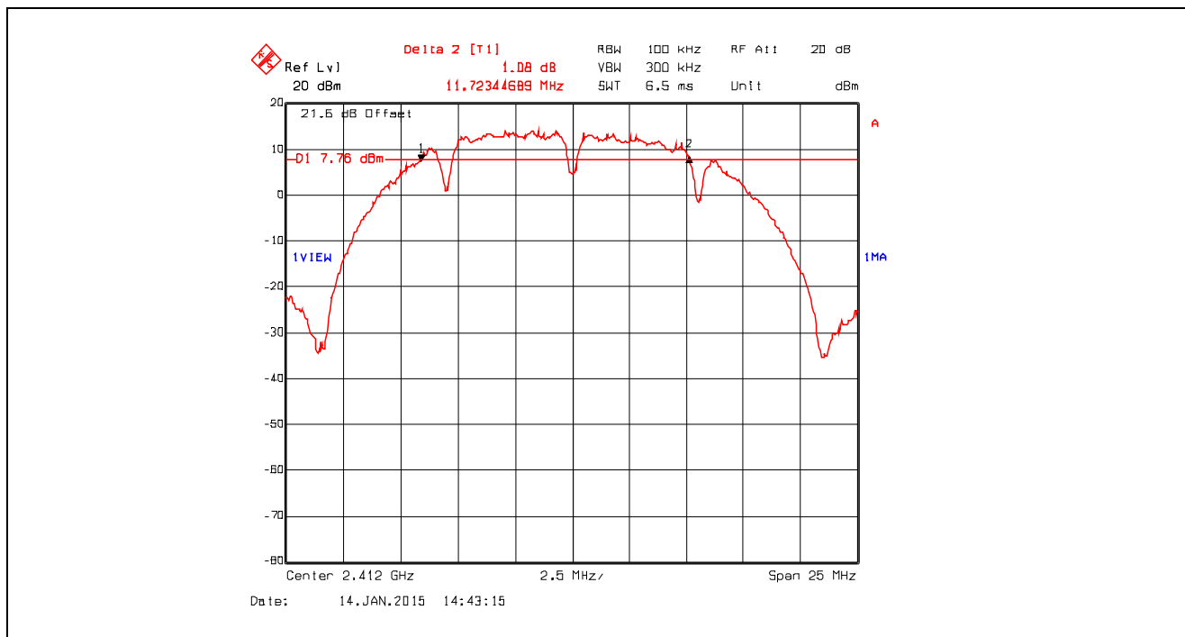
Plot 5.2.4.8. 6 dB Bandwidth, Data Rate 2, Chain # 2, Ch 1, 2412 MHz, Software Output Power Setting 26
