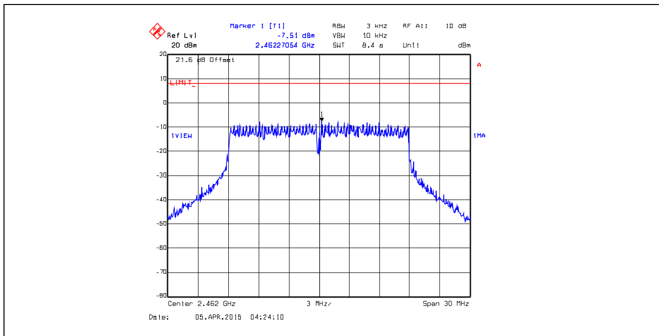
Plot 5.6.4.48. Power Spectral Density Data Rate 8, Chain # 2, Ch 11, 2462 MHz, Software Output Power Setting 19
