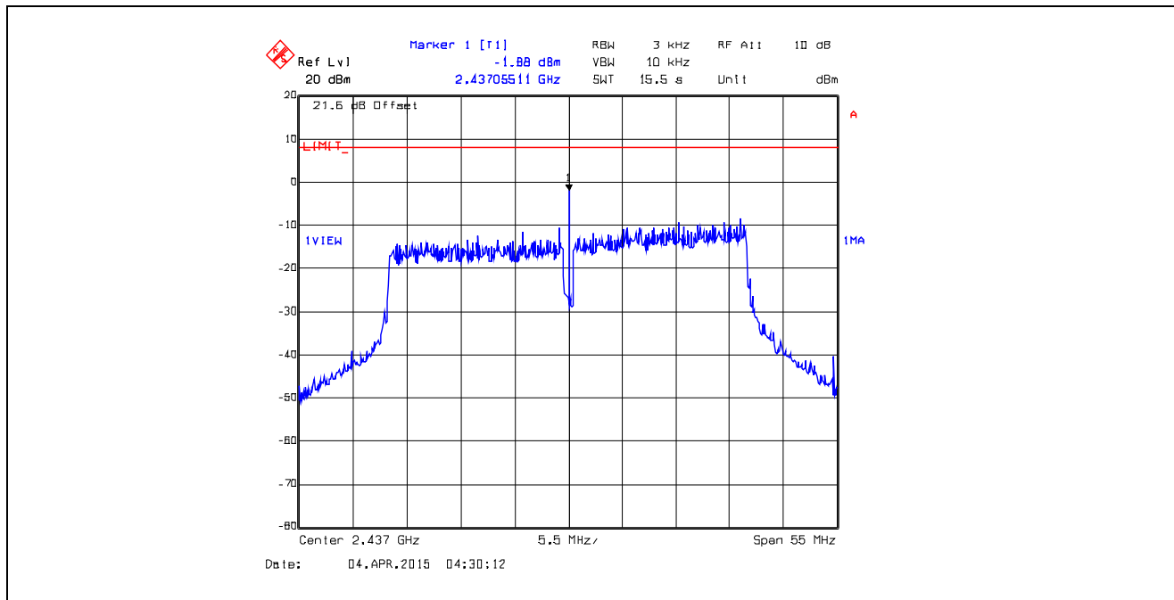
Plot 5.6.4.69. Power Spectral Density Data Rate 12, Chain # 1, Ch 6, 2437 MHz, Software Output Power Setting 17
