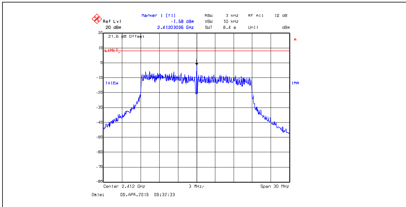
Plot 5.6.4.61. Power Spectral Density Data Rate 11, Chain # 1, Ch 1, 2412 MHz, Software Output Power Setting 19
