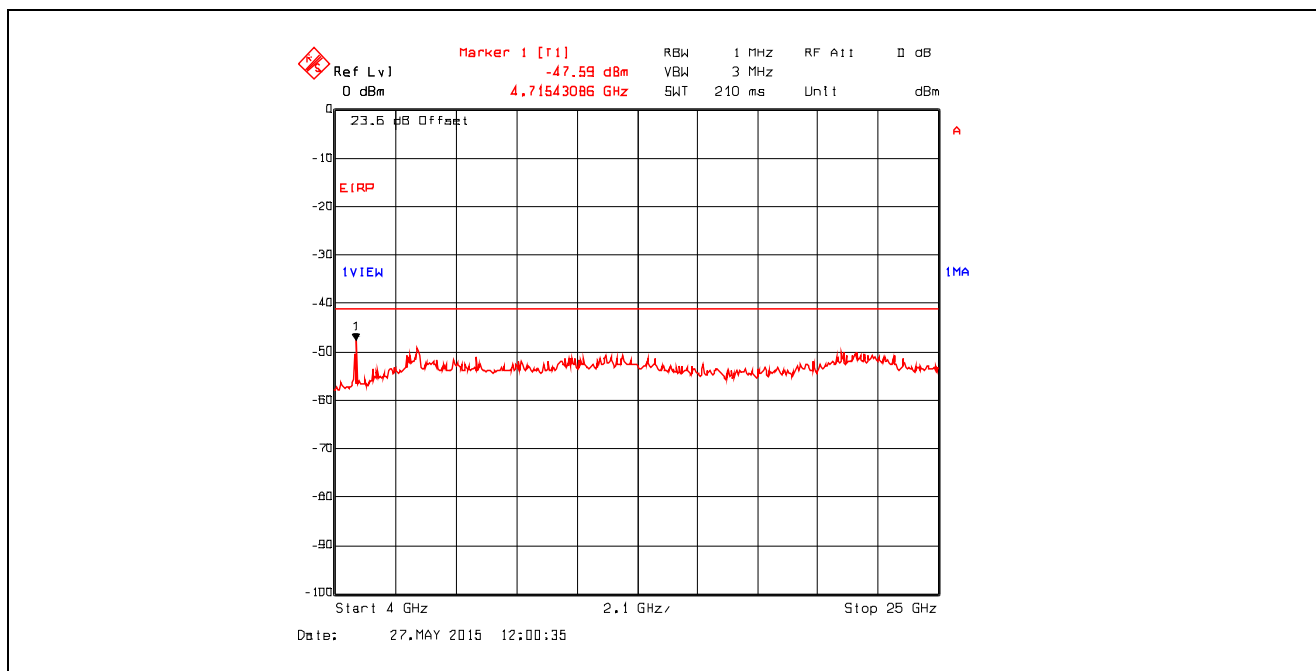
Plot 5.4.4.3.80. Conducted Spurious Emissions in Restricted Frequency Bands Chain #2 , Data Rate 11, Ch 6, 2437 MHz, Software Output Power Setting 19, 4 GHz - 25 GHz, Peak Detector
