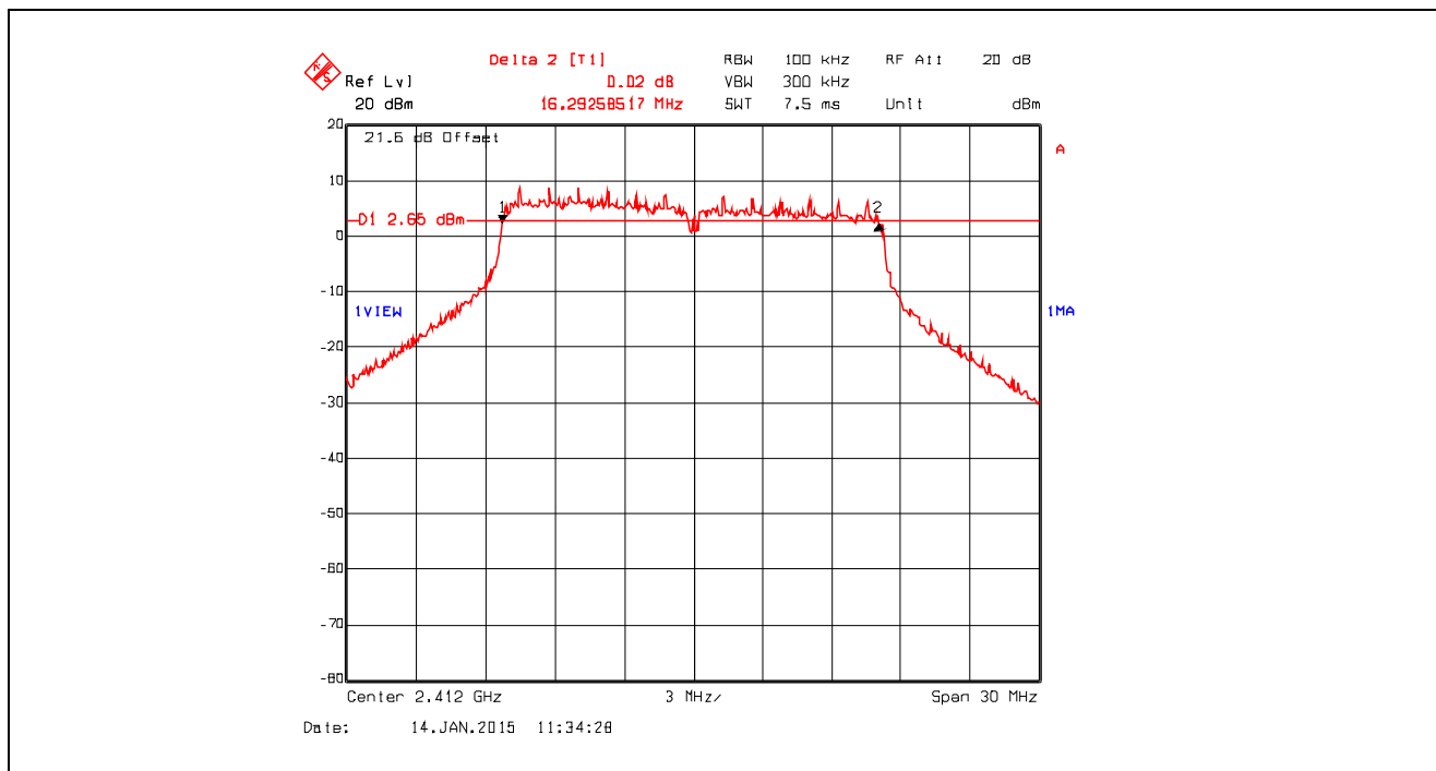
Plot 5.2.4.20. 6 dB Bandwidth, Data Rate 4, Chain # 2, Ch 1, 2412 MHz, Software Output Power Setting 18
