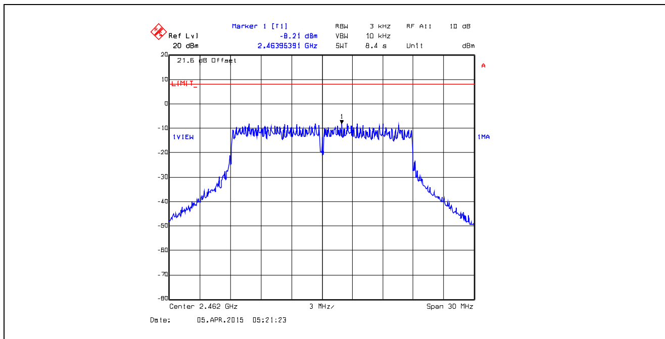
Plot 5.6.4.60. Power Spectral Density Data Rate 10, Chain # 2, Ch 11, 2462 MHz, Software Output Power Setting 19
