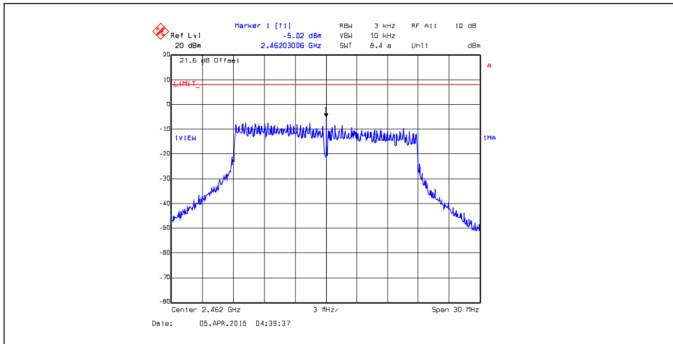
Plot 5.6.4.53. Power Spectral Density Data Rate 9, Chain # 1, Ch 11, 2462 MHz, Software Output Power Setting 19
