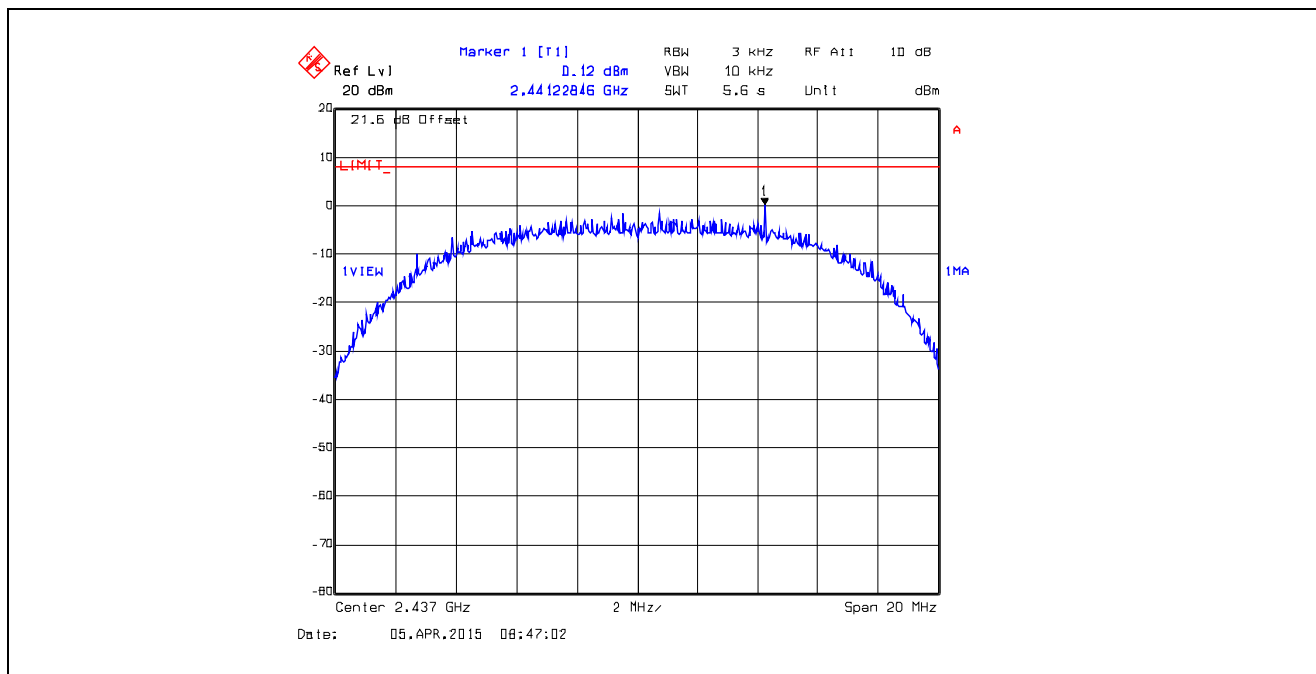
Plot 5.6.4.16. Power Spectral Density Data Rate 3, Chain # 2, Ch 6, 2437 MHz, Software Output Power Setting 26
