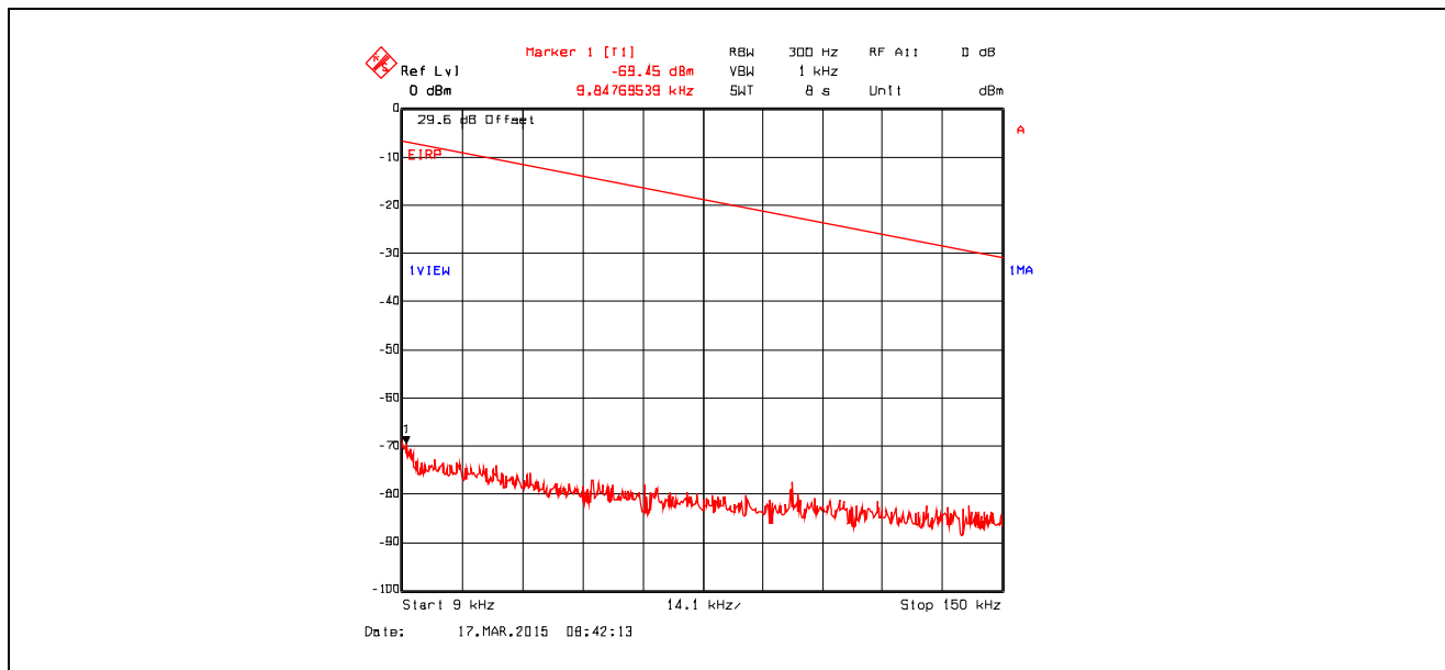
Plot 5.4.4.3.2. Conducted Spurious Emissions in Restricted Frequency Bands Chain #2 , Data Rate 3, Ch 1, 2412 MHz, Software Output Power Setting 26, 9 kHz - 150 kHz, Peak Detector
