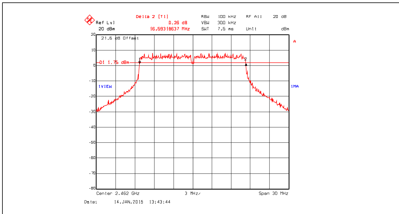
Plot 5.2.4.36. 6 dB Bandwidth, Data Rate 6, Chain # 2, Ch 11, 2462 MHz, Software Output Power Setting 18
