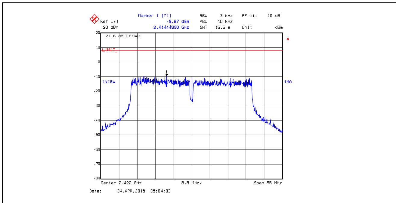
Plot 5.6.4.74. Power Spectral Density Data Rate 13, Chain # 2, Ch 3, 2422 MHz, Software Output Power Setting 17
