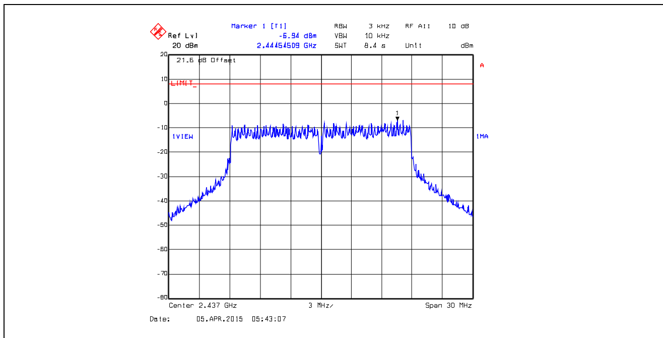
Plot 5.6.4.64. Power Spectral Density Data Rate 11, Chain # 2, Ch 6, 2437 MHz, Software Output Power Setting 19
