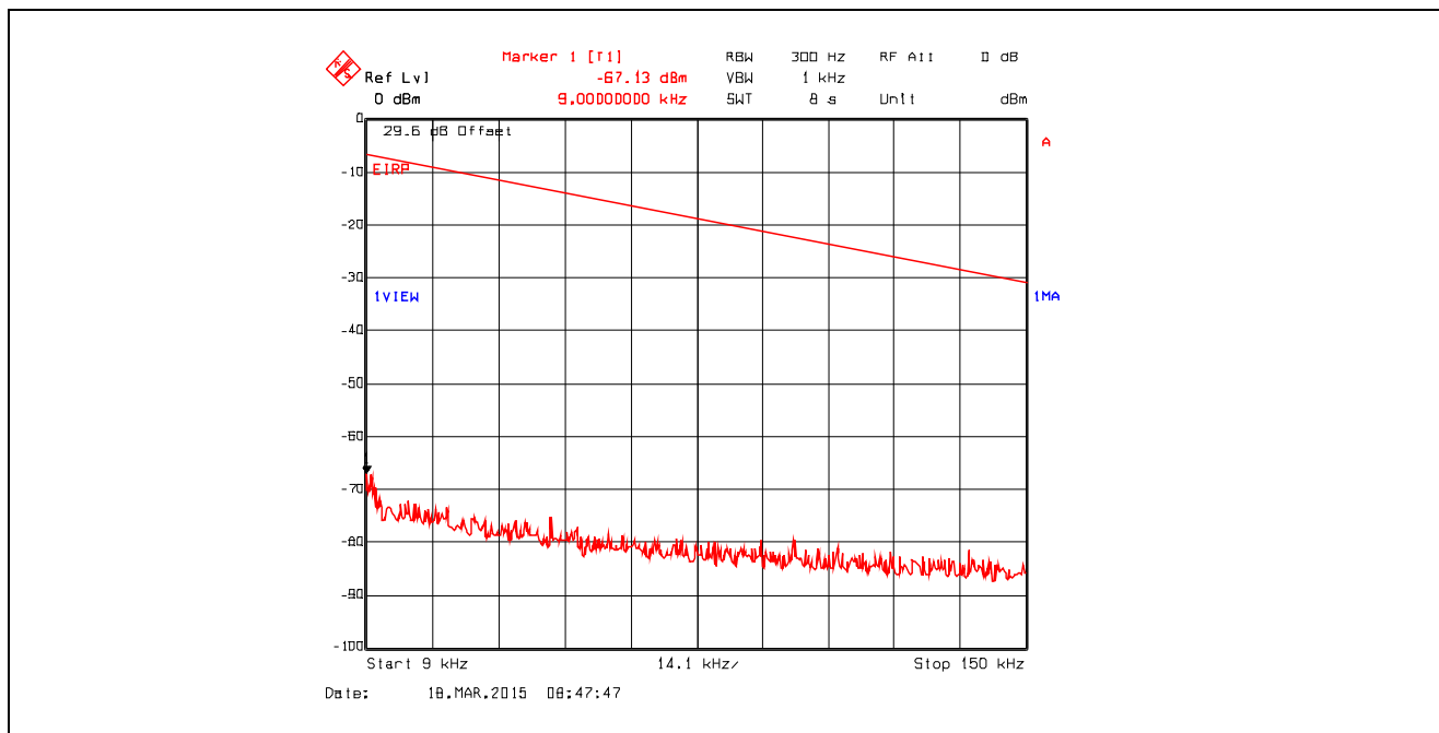
Plot 5.4.4.3.72. Conducted Spurious Emissions in Restricted Frequency Bands Chain #2 , Data Rate 11, Ch 6, 2437 MHz, Software Output Power Setting 19, 9 kHz - 150 kHz, Peak Detector
