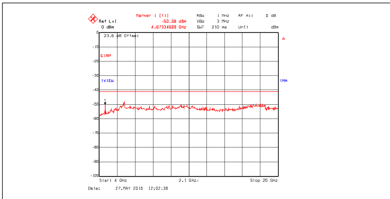
Plot 5.4.4.3.70. Conducted Spurious Emissions in Restricted Frequency Bands Chain #2 , Data Rate 11, Ch 1, 2412 MHz, Software Output Power Setting 19, 4 GHz - 25 GHz, Peak Detector
