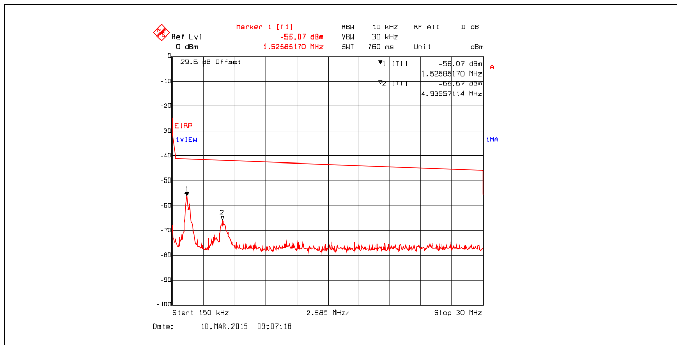
Plot 5.4.4.3.73. Conducted Spurious Emissions in Restricted Frequency Bands Chain #1 , Data Rate 11, Ch 6, 2437 MHz, Software Output Power Setting 19, 150 kHz - 30 MHz, Peak Detector
