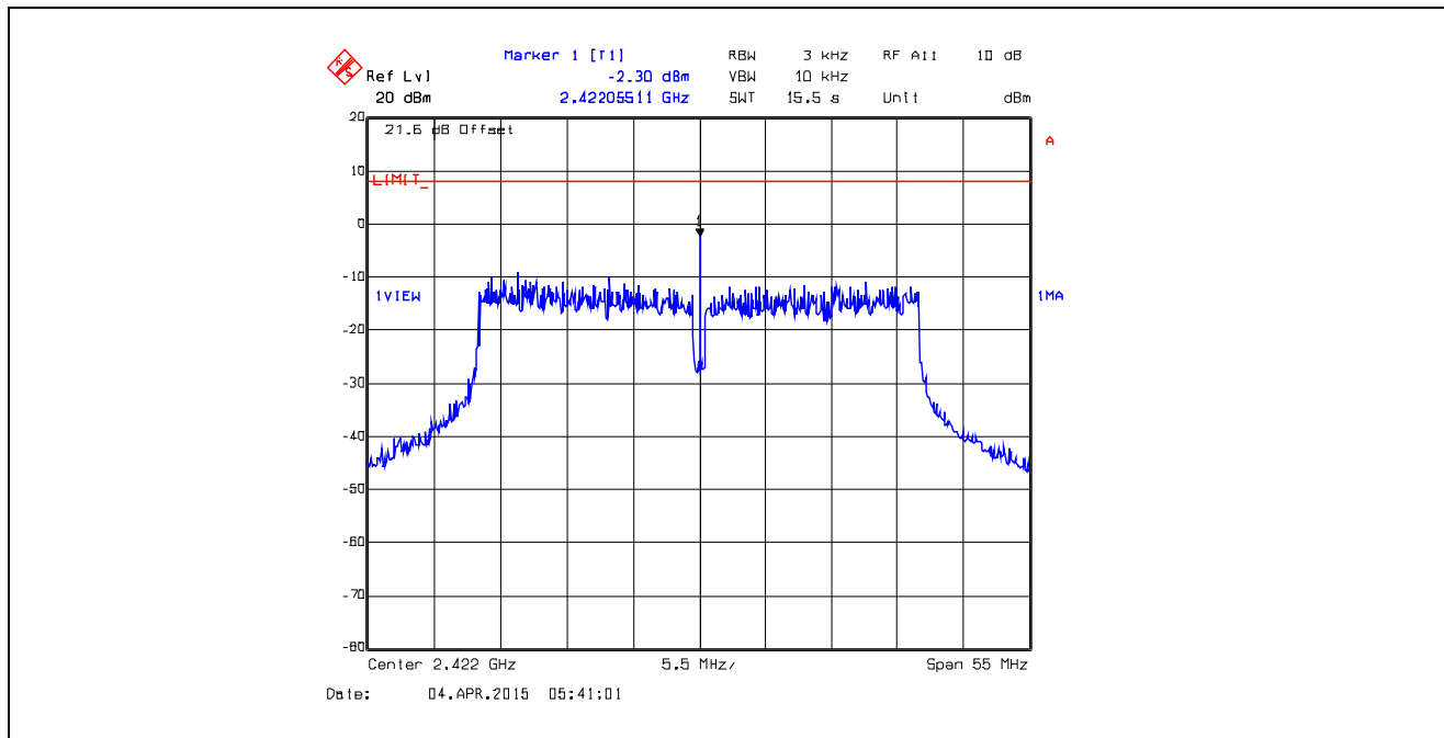
Plot 5.6.4.85. Power Spectral Density Data Rate 15, Chain # 1, Ch 3, 2422 MHz, Software Output Power Setting 17
