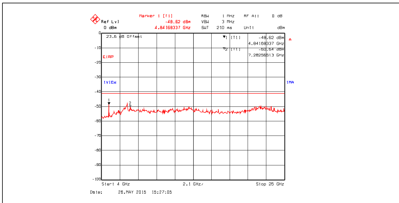
Plot 5.4.4.3.20. Conducted Spurious Emissions in Restricted Frequency Bands Chain #2 , Data Rate 3, Ch 6, 2437 MHz, Software Output Power Setting 26, 4 GHz - 25 GHz, Peak Detector
