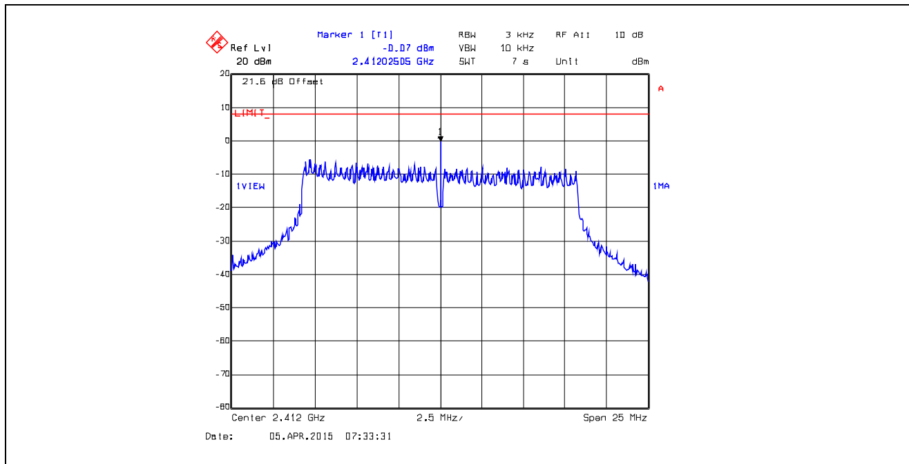
Plot 5.6.4.37. Power Spectral Density Data Rate 7, Chain # 1, Ch 1, 2412 MHz, Software Output Power Setting 18
