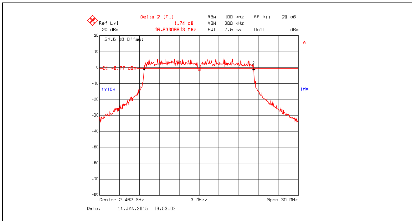
Plot 5.2.4.35. 6 dB Bandwidth, Data Rate 6, Chain # 1, Ch 11, 2462 MHz, Software Output Power Setting 18
