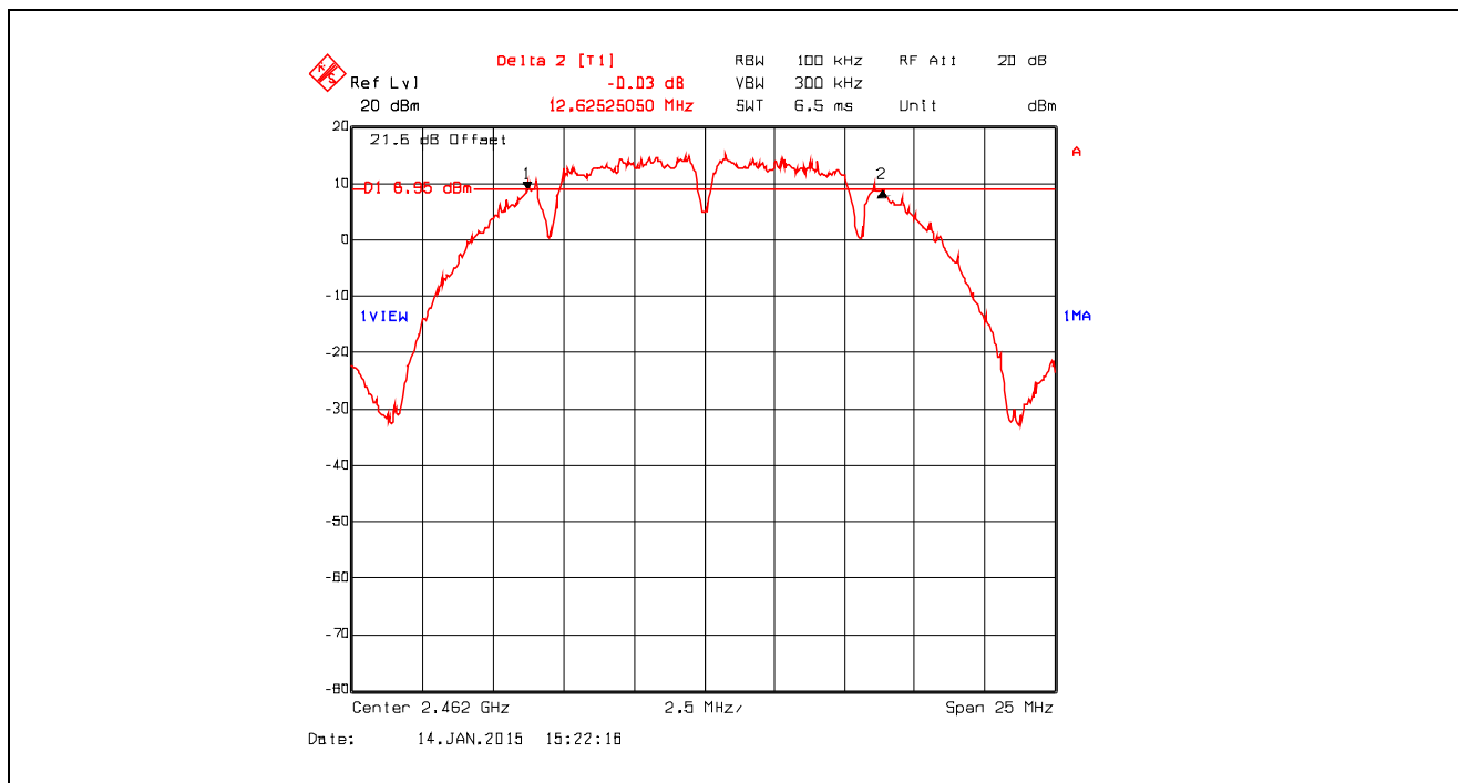
Plot 5.2.4.12. 6 dB Bandwidth, Data Rate 2, Chain # 2, Ch 11, 2462 MHz, Software Output Power Setting 26
