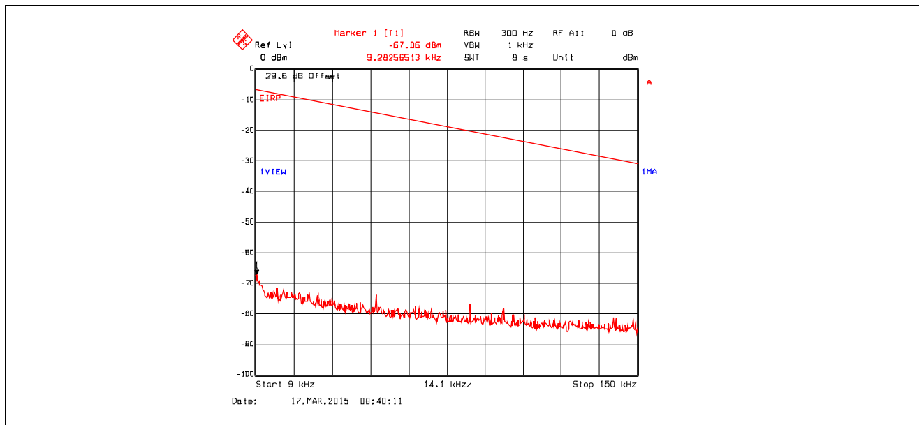
Plot 5.4.4.3.1. Conducted Spurious Emissions in Restricted Frequency Bands Chain #1 , Data Rate 3, Ch 1, 2412 MHz, Software Output Power Setting 26, 9 kHz - 150 kHz, Peak Detector
