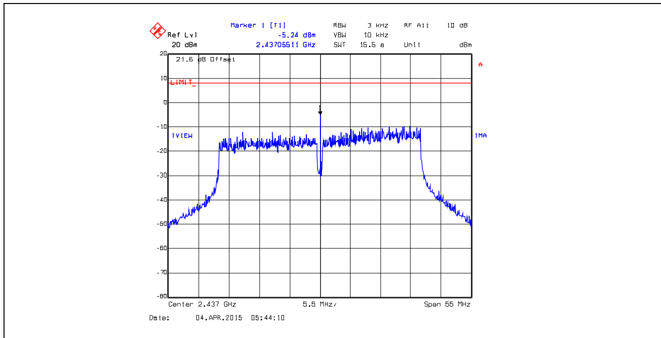
Plot 5.6.4.87. Power Spectral Density Data Rate 15, Chain # 1, Ch 6, 2437 MHz, Software Output Power Setting 17
