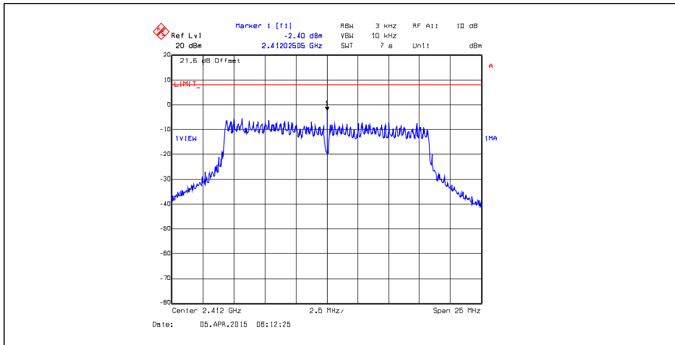
Plot 5.6.4.19. Power Spectral Density Data Rate 4, Chain # 1, Ch 1, 2412 MHz, Software Output Power Setting 18
