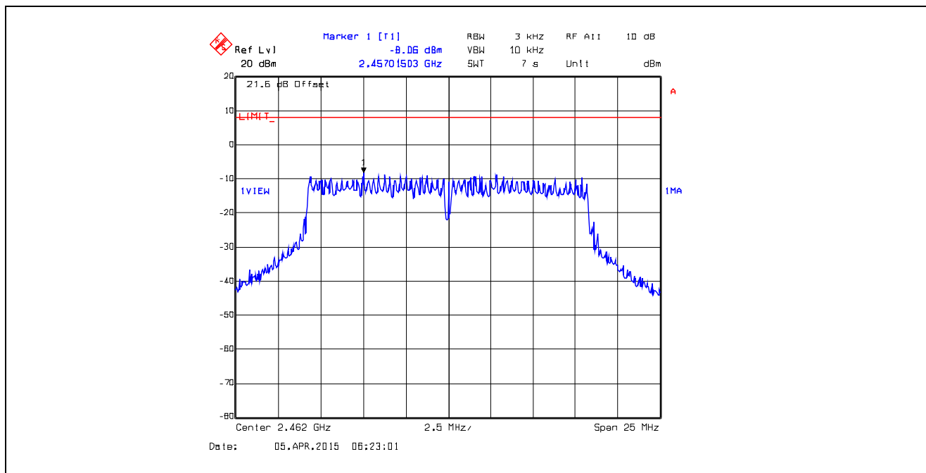
Plot 5.6.4.30. Power Spectral Density Data Rate 5, Chain # 2, Ch 11, 2462 MHz, Software Output Power Setting 18
