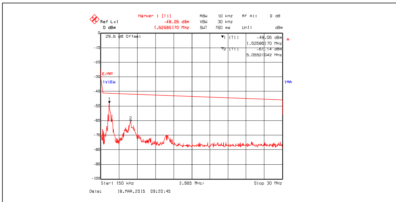
Plot 5.4.4.3.74. Conducted Spurious Emissions in Restricted Frequency Bands Chain #2 , Data Rate 11, Ch 6, 2437 MHz, Software Output Power Setting 19, 150 kHz - 30 MHz, Peak Detector
