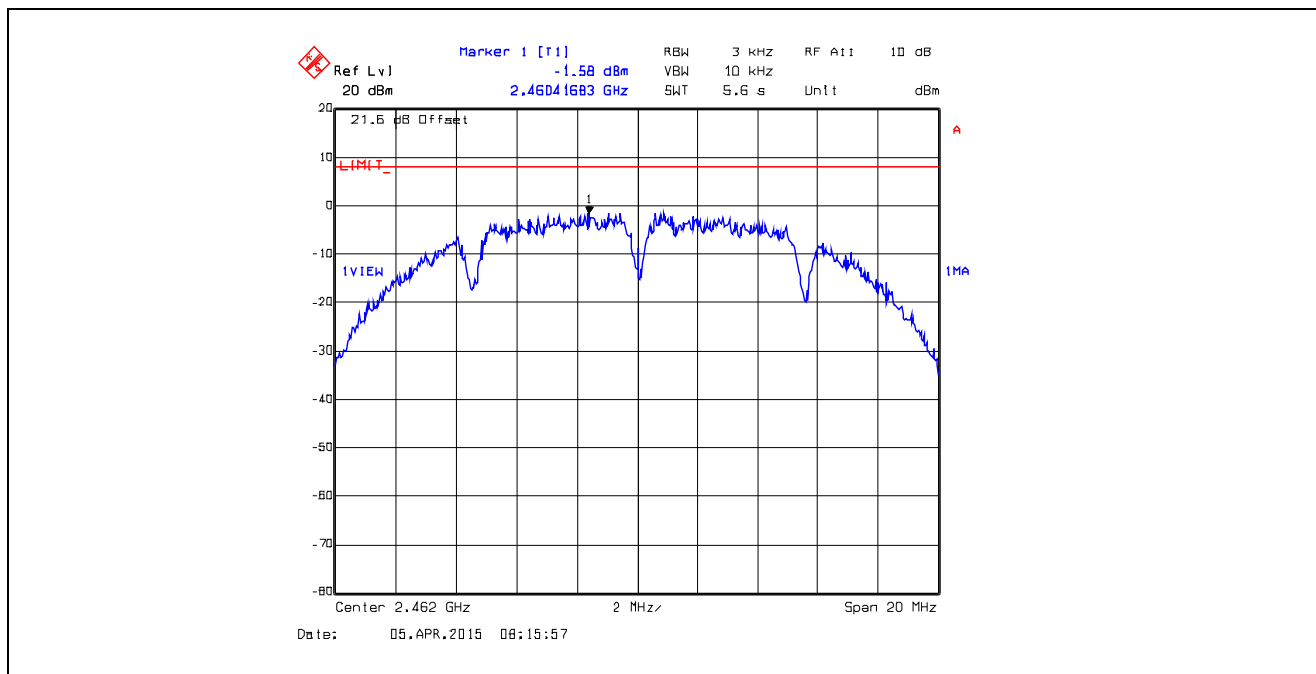
Plot 5.6.4.6. Power Spectral Density Data Rate 1, Chain # 2, Ch 11, 2462 MHz, Software Output Power Setting 26
