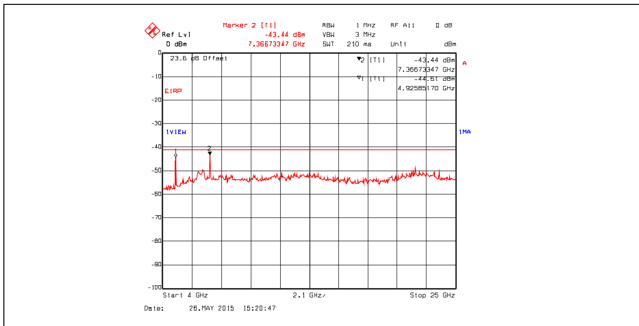
Plot 5.4.4.3.29. Conducted Spurious Emissions in Restricted Frequency Bands Chain #1 , Data Rate 3, Ch 11, 2462 MHz, Software Output Power Setting 26, 4 GHz - 25 GHz, Peak Detector
