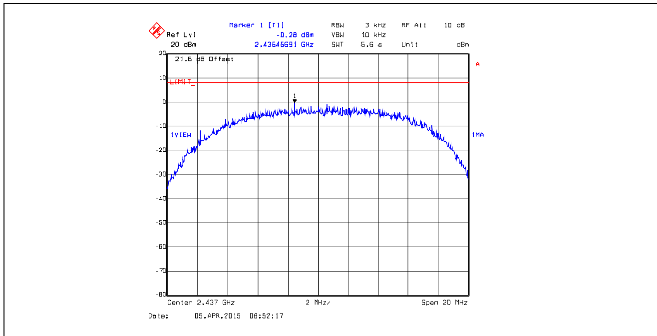
Plot 5.6.4.15. Power Spectral Density Data Rate 3, Chain # 1, Ch 6, 2437 MHz, Software Output Power Setting 26
