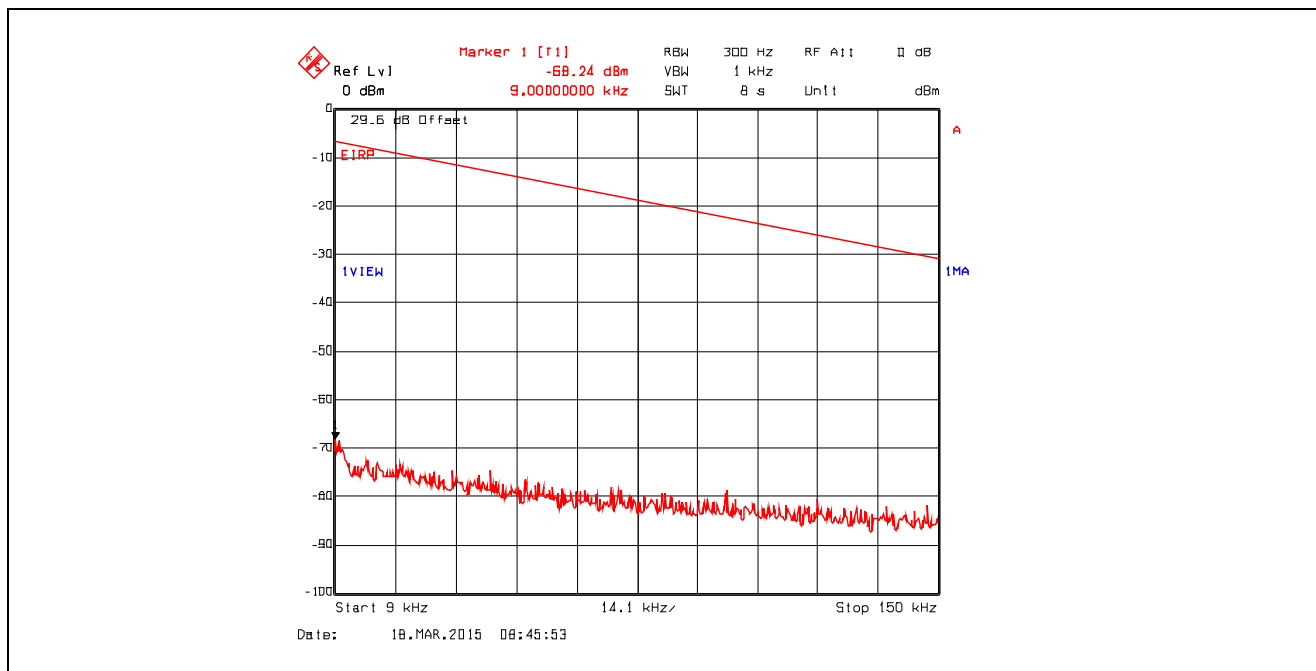
Plot 5.4.4.3.71. Conducted Spurious Emissions in Restricted Frequency Bands Chain #1 , Data Rate 11, Ch 6, 2437 MHz, Software Output Power Setting 19, 9 kHz - 150 kHz, Peak Detector
