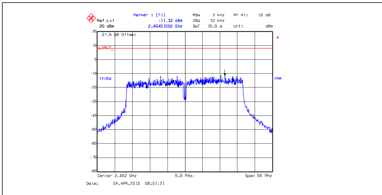
Plot 5.6.4.90. Power Spectral Density Data Rate 15, Chain # 2, Ch 9, 2452 MHz, Software Output Power Setting 17
