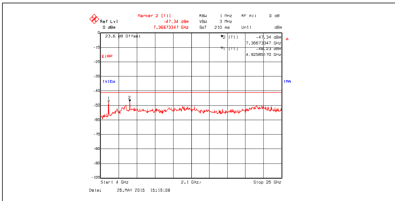
Plot 5.4.4.3.30. Conducted Spurious Emissions in Restricted Frequency Bands Chain #2 , Data Rate 3, Ch 11, 2462 MHz, Software Output Power Setting 26, 4 GHz - 25 GHz, Peak Detector
