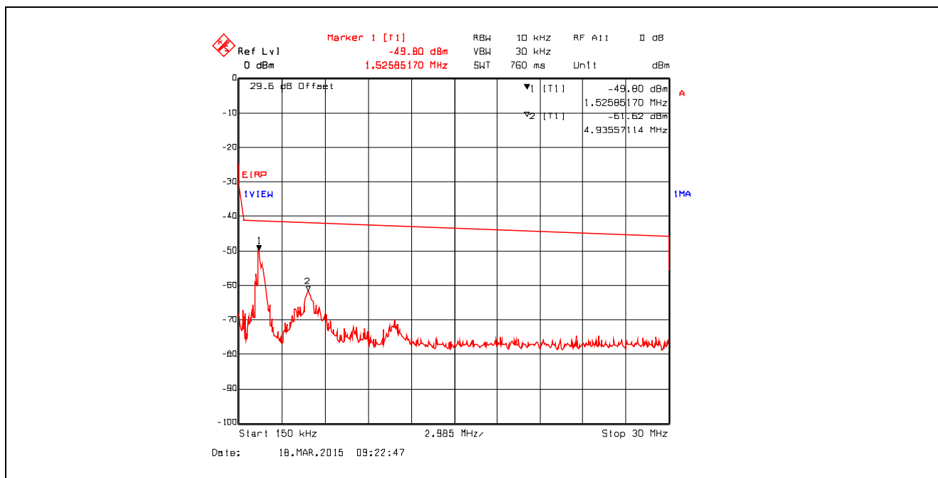
Plot 5.4.4.3.84. Conducted Spurious Emissions in Restricted Frequency Bands Chain #2 , Data Rate 11, Ch 11, 2462 MHz, Software Output Power Setting 19, 150 kHz - 30 MHz, Peak Detector
