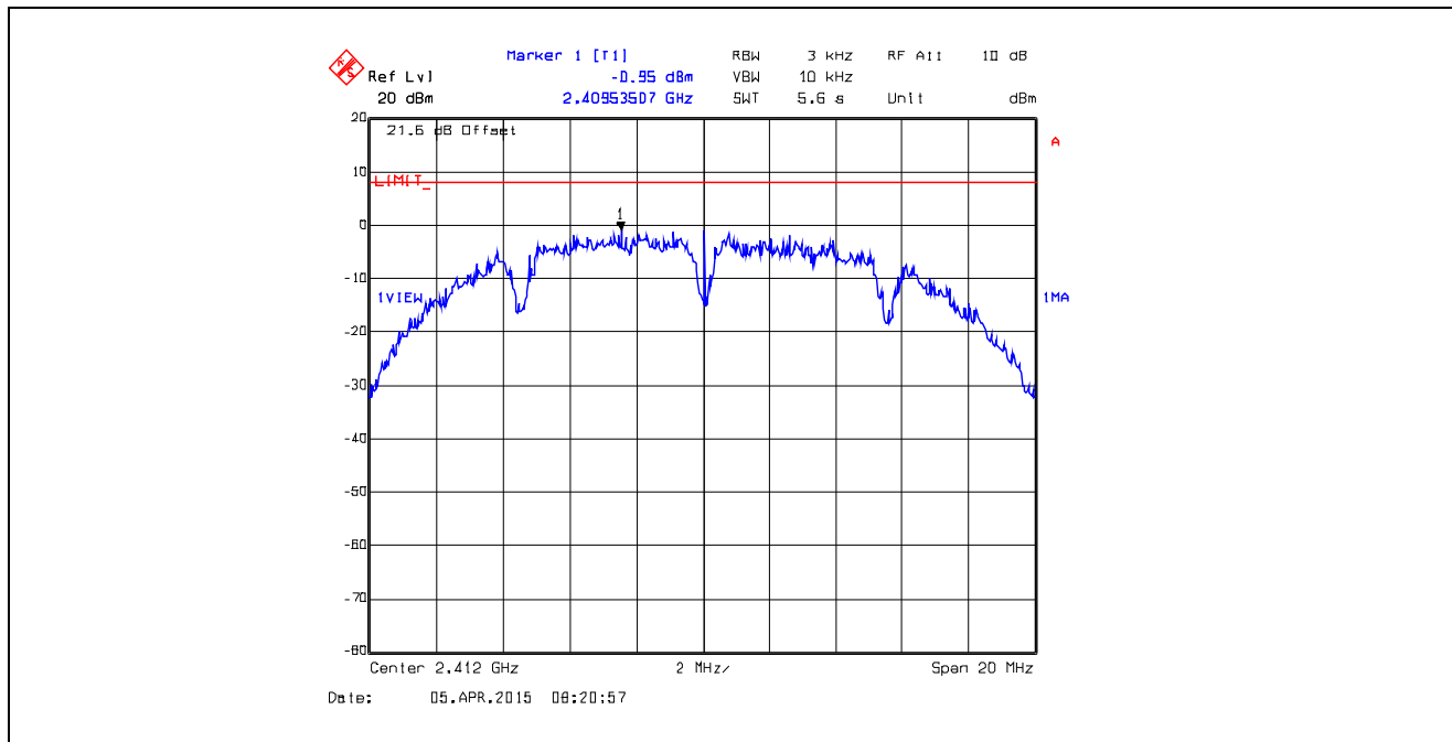
Plot 5.6.4.1. Power Spectral Density Data Rate 1, Chain # 1, Ch 1, 2412 MHz, Software Output Power Setting 26
