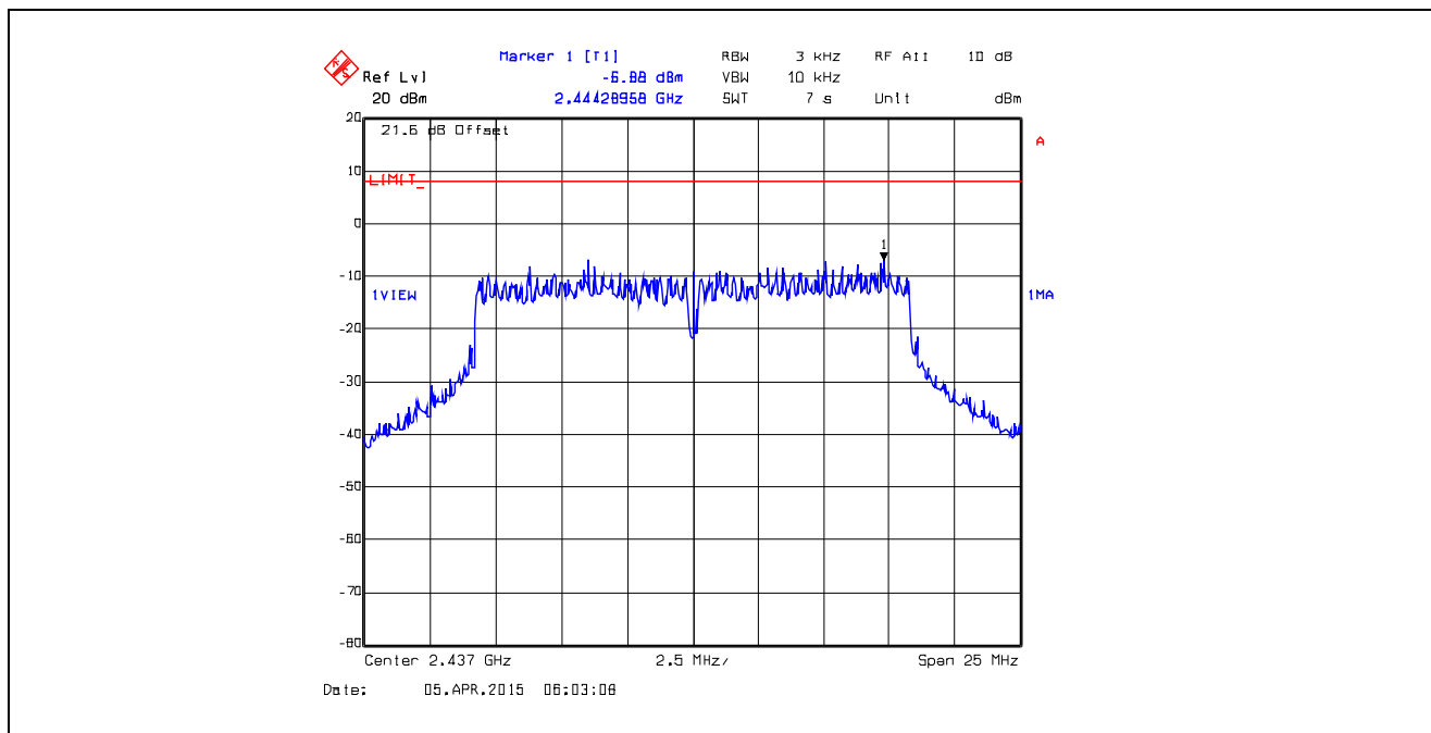
Plot 5.6.4.22. Power Spectral Density Data Rate 4, Chain # 2, Ch 6, 2437 MHz, Software Output Power Setting 18
