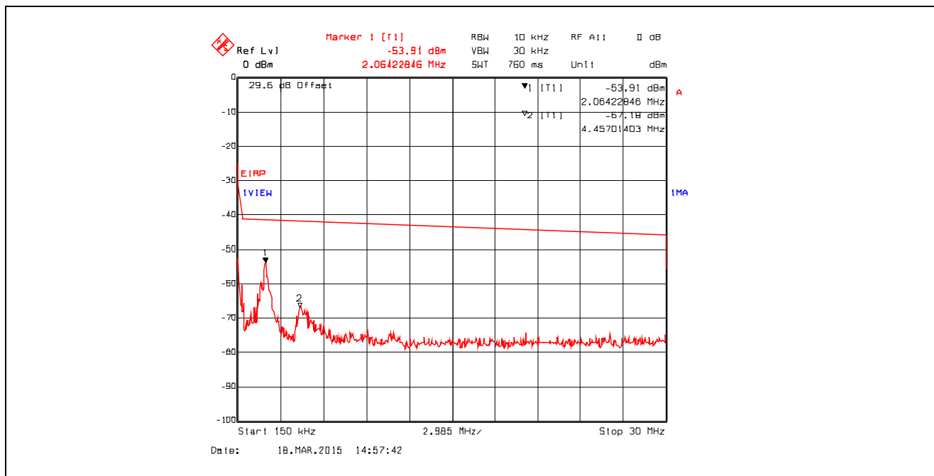
Plot 5.4.4.3.93. Conducted Spurious Emissions in Restricted Frequency Bands Chain #1 , Data Rate 15, Ch 3, 2422 MHz, Software Output Power Setting 17, 150 kHz - 30 MHz, Peak Detector
