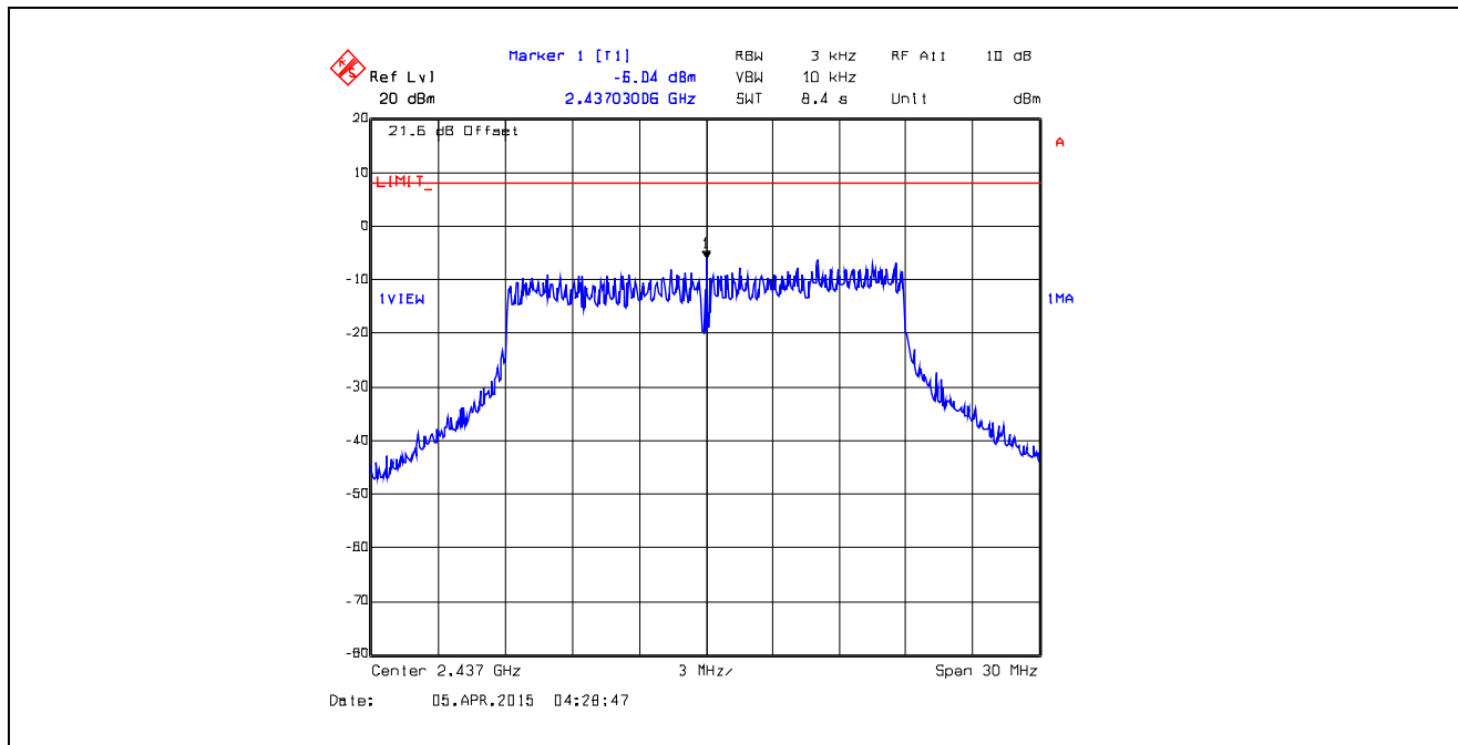
Plot 5.6.4.45. Power Spectral Density Data Rate 8, Chain # 1, Ch 6, 2437 MHz, Software Output Power Setting 19
