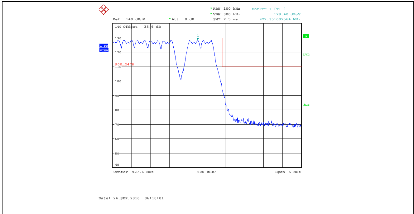
Plot 5.2.4.4.2.6. Band-Edge RF Radiated Emissions at 3 m, Horizontal Polarization Pseudorandom Channel Hopping Mode, High End of Frequency Band, Power Setting 23, Data Rate at 276480 kbps
