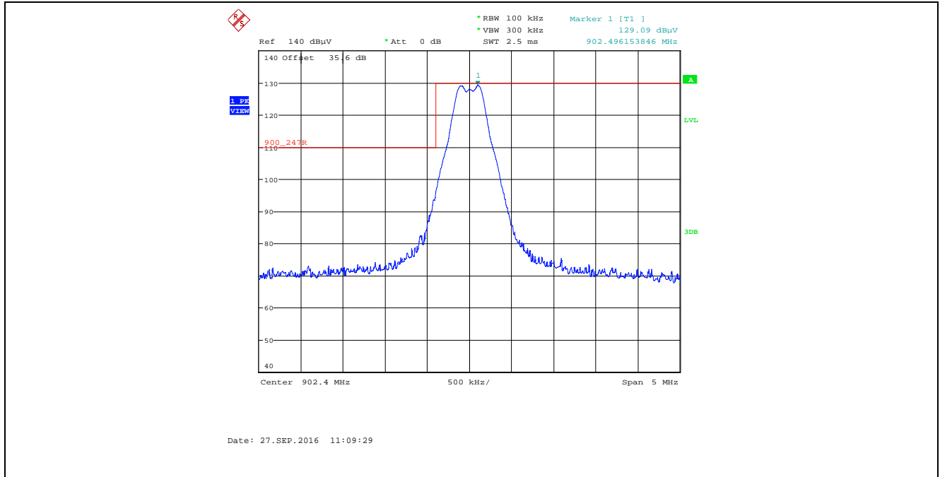
Plot 5.2.4.1.2.1. Band-Edge RF Radiated Emissions at 3 m, Horizontal Polarization Single Frequency Mode, Low End of Frequency Band, Power Setting 28, Data Rate at 276480 kbps
