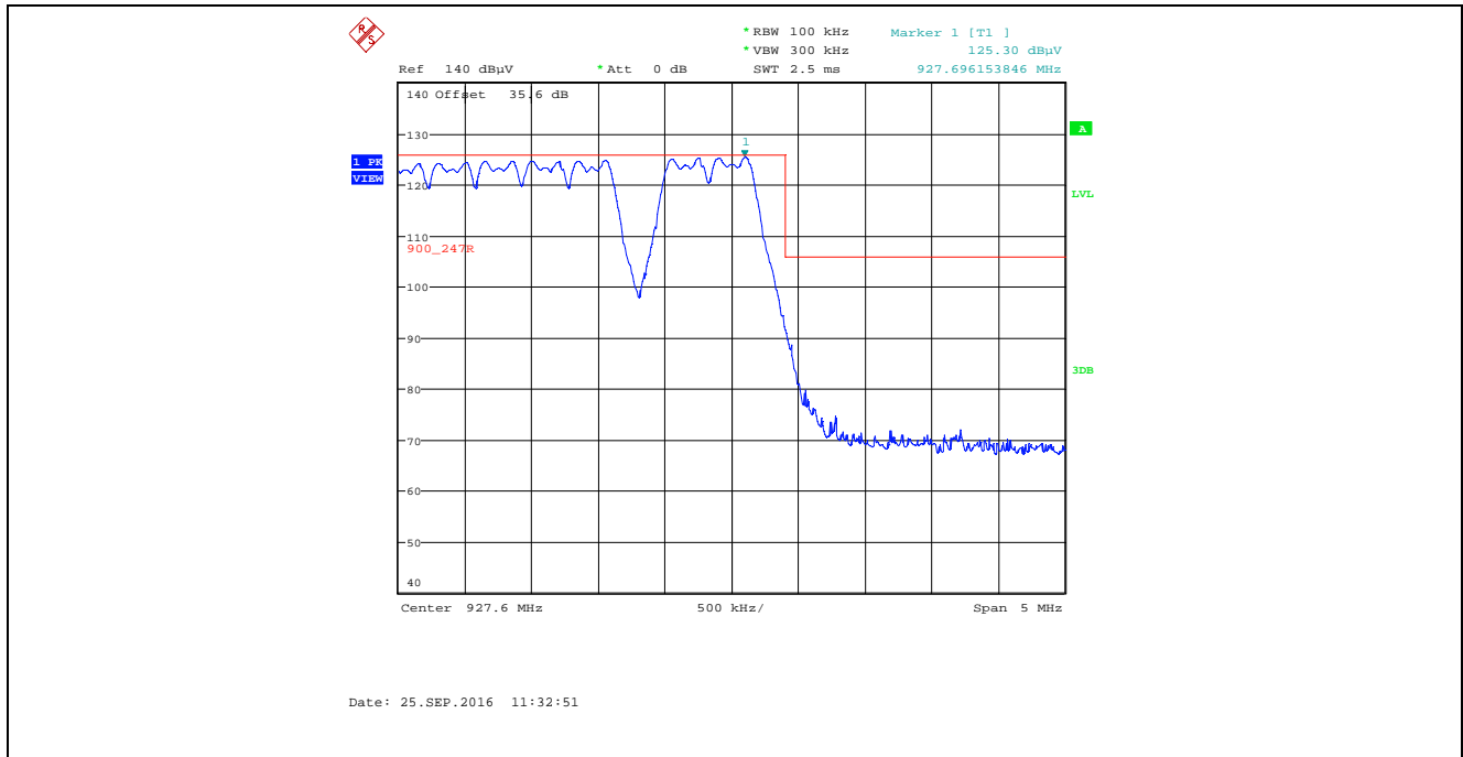
Plot 5.2.4.2.2.6. Band-Edge RF Radiated Emissions at 3 m, Horizontal Polarization Pseudorandom Channel Hopping Mode, High End of Frequency Band, Power Setting 28, Data Rate at 276480 kbps
