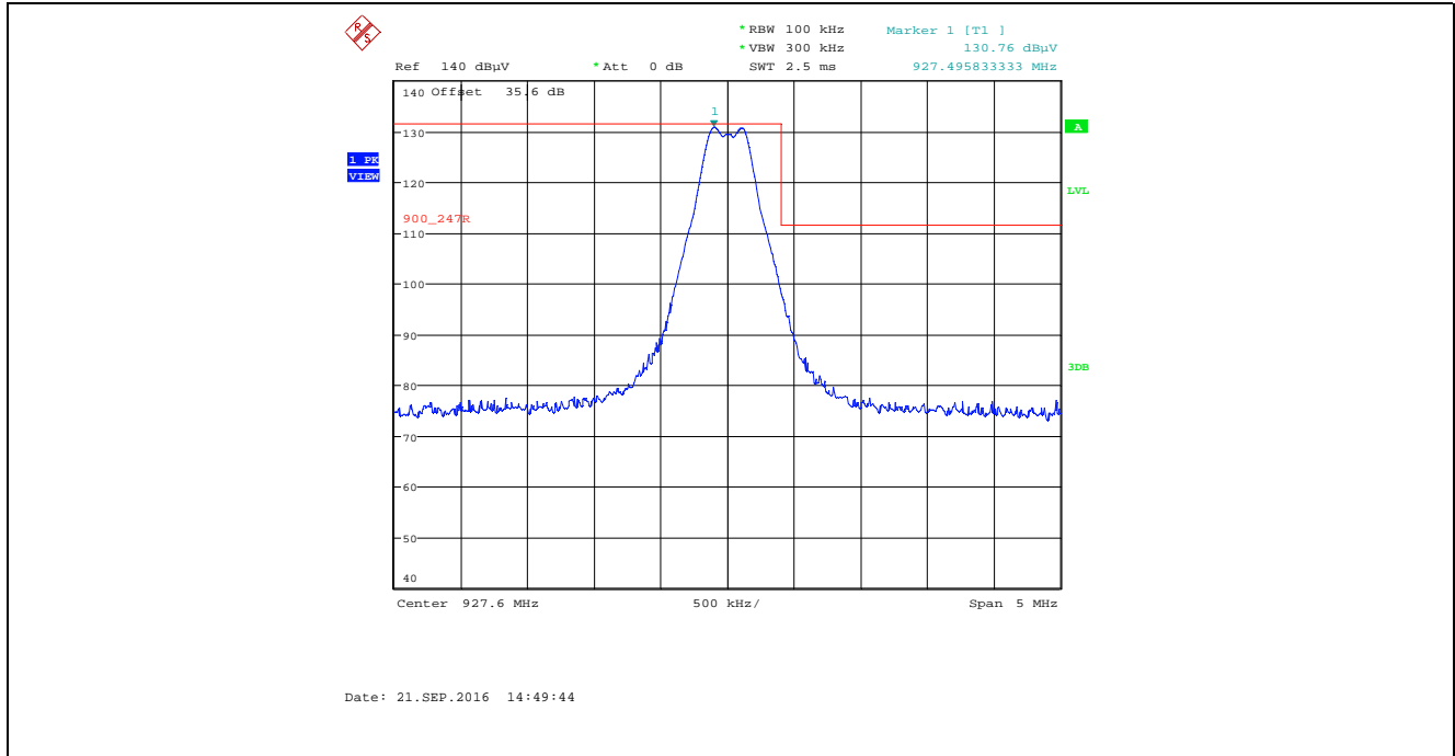
Plot 5.2.4.5.2.7. Band-Edge RF Radiated Emissions at 3 m, Vertical Polarization Single Frequency Mode, High of Frequency Band, Power Setting 12, Data Rate at 276480 kbps
