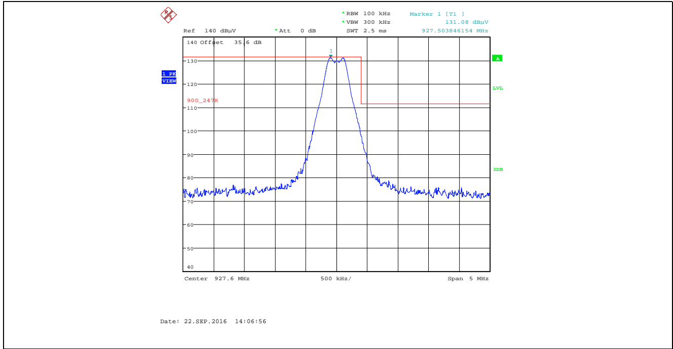
Plot 5.2.4.5.2.5. Band-Edge RF Radiated Emissions at 3 m, Horizontal Polarization Single Frequency Mode, High End of Frequency Band, Power Setting 12, Data Rate at 276480 kbps
