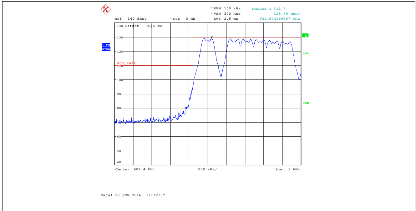
Plot 5.2.4.1.2.2. Band-Edge RF Radiated Emissions at 3 m, Horizontal Polarization Pseudorandom Channel Hopping Mode, Low End of Frequency Band, Power Setting 28, Data Rate at 276480 kbps
