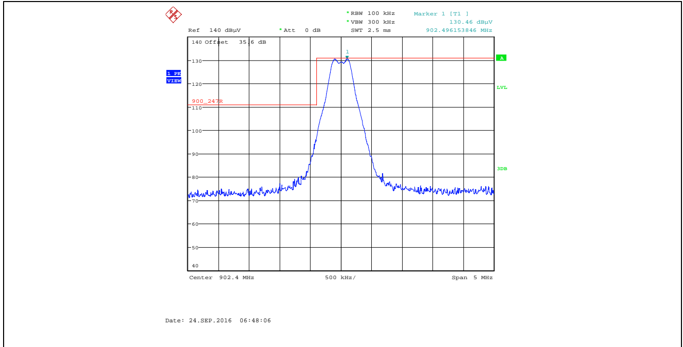
Plot 5.2.4.4.2.1. Band-Edge RF Radiated Emissions at 3 m, Horizontal Polarization Single Frequency Mode, Low End of Frequency Band, Power Setting 23, Data Rate at 276480 kbps
