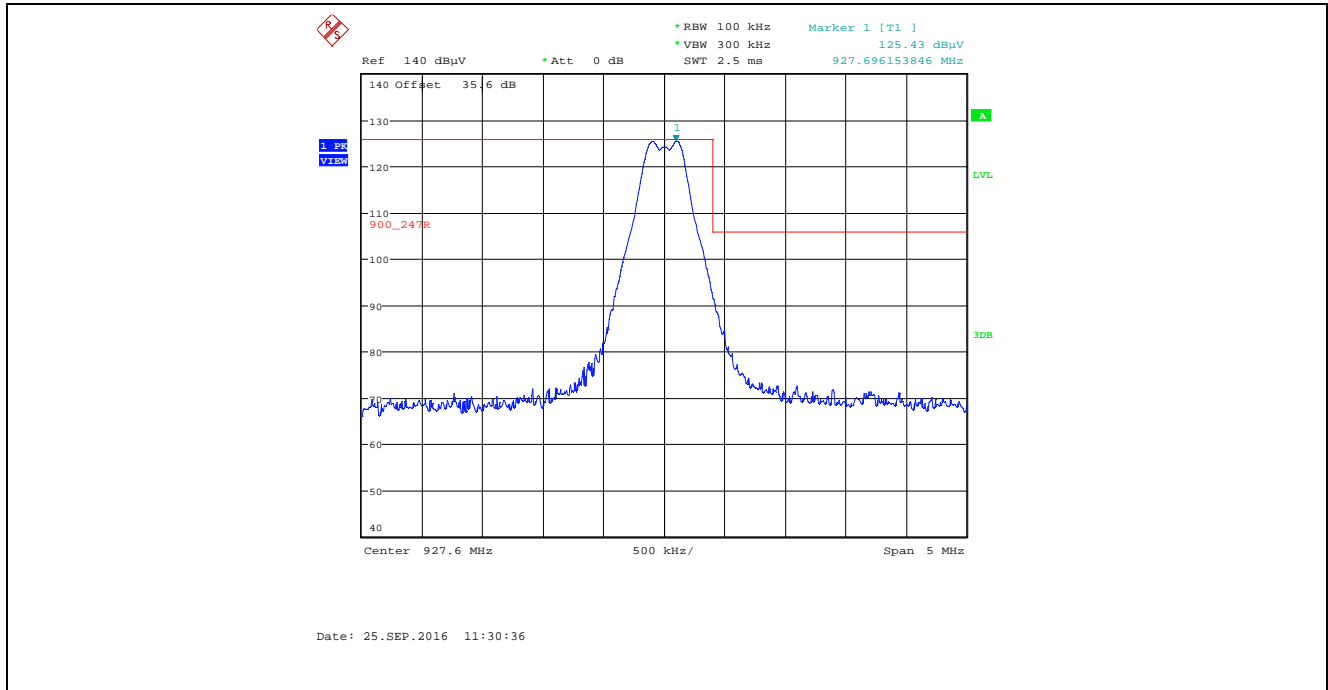
Plot 5.2.4.2.2.5. Band-Edge RF Radiated Emissions at 3 m, Horizontal Polarization Single Frequency Mode, High End of Frequency Band, Power Setting 28, Data Rate at 276480 kbps
