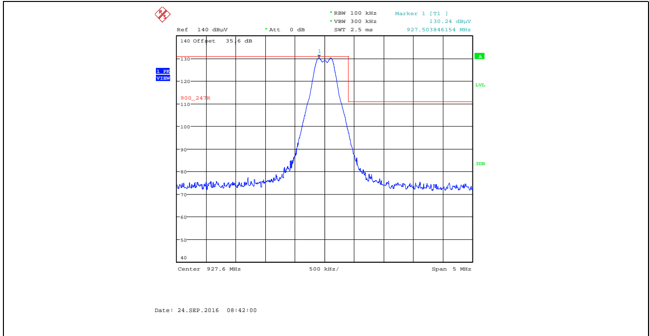
Plot 5.2.4.3.2.7. Band-Edge RF Radiated Emissions at 3 m, Vertical Polarization Single Frequency Mode, High of Frequency Band, Power Setting 22, Data Rate at 276480 kbps
