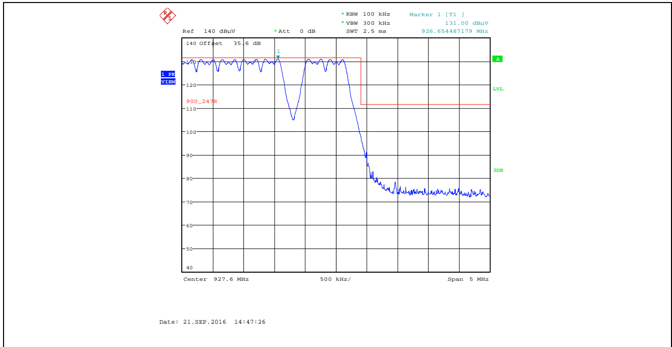
Plot 5.2.4.5.2.8. Band-Edge RF Radiated Emissions at 3 m, Vertical Polarization Pseudorandom Channel Hopping Mode, High End of Frequency Band, Power Setting 12, Data Rate at 276480 kbps
