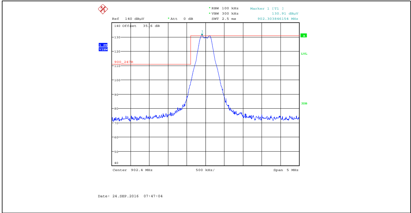
Plot 5.2.4.3.2.3. Band-Edge RF Radiated Emissions at 3 m, Vertical Polarization Single Frequency Mode, Low End of Frequency Band, Power Setting 22, Data Rate at 276480 kbps
