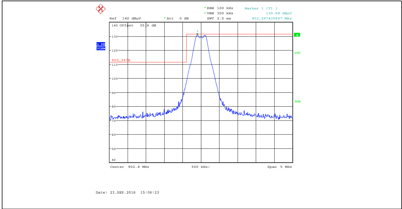
Plot 5.2.4.4.2.3. Band-Edge RF Radiated Emissions at 3 m, Vertical Polarization Single Frequency Mode, Low End of Frequency Band, Power Setting 23, Data Rate at 276480 kbps
