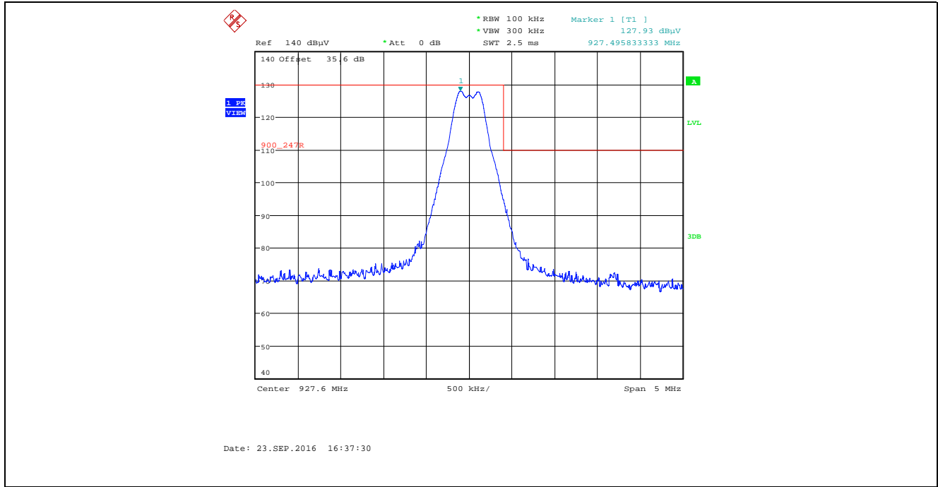
Plot 5.2.4.4.2.7. Band-Edge RF Radiated Emissions at 3 m, Vertical Polarization Single Frequency Mode, High of Frequency Band, Power Setting 23, Data Rate at 276480 kbps
