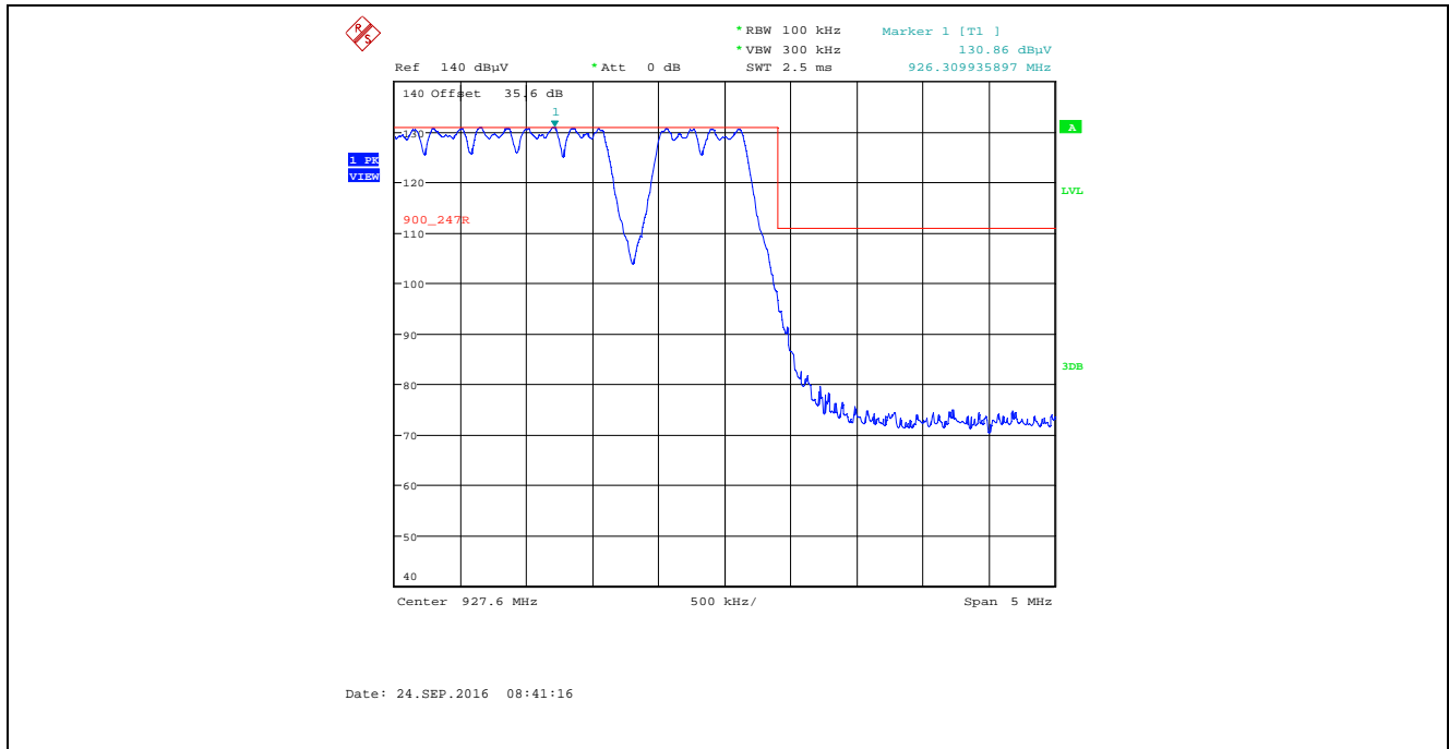
Plot 5.2.4.3.2.8. Band-Edge RF Radiated Emissions at 3 m, Vertical Polarization Pseudorandom Channel Hopping Mode, High End of Frequency Band, Power Setting 22, Data Rate at 276480 kbps
