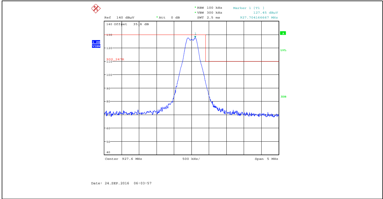
Plot 5.2.4.4.2.5. Band-Edge RF Radiated Emissions at 3 m, Horizontal Polarization Single Frequency Mode, High End of Frequency Band, Power Setting 23, Data Rate at 276480 kbps
