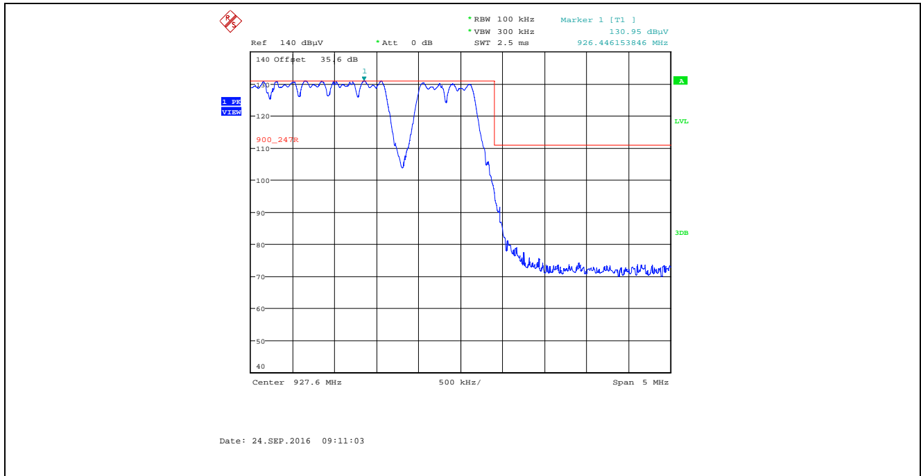
Plot 5.2.4.3.2.6. Band-Edge RF Radiated Emissions at 3 m, Horizontal Polarization Pseudorandom Channel Hopping Mode, High End of Frequency Band, Power Setting 22, Data Rate at 276480 kbps
