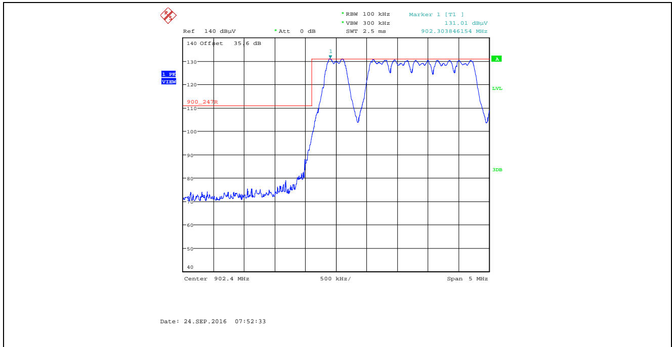
Plot 5.2.4.3.2.4. Band-Edge RF Radiated Emissions at 3 m, Vertical Polarization Pseudorandom Channel Hopping Mode, Low End of Frequency Band, Power Setting 22, Data Rate at 276480 kbps
