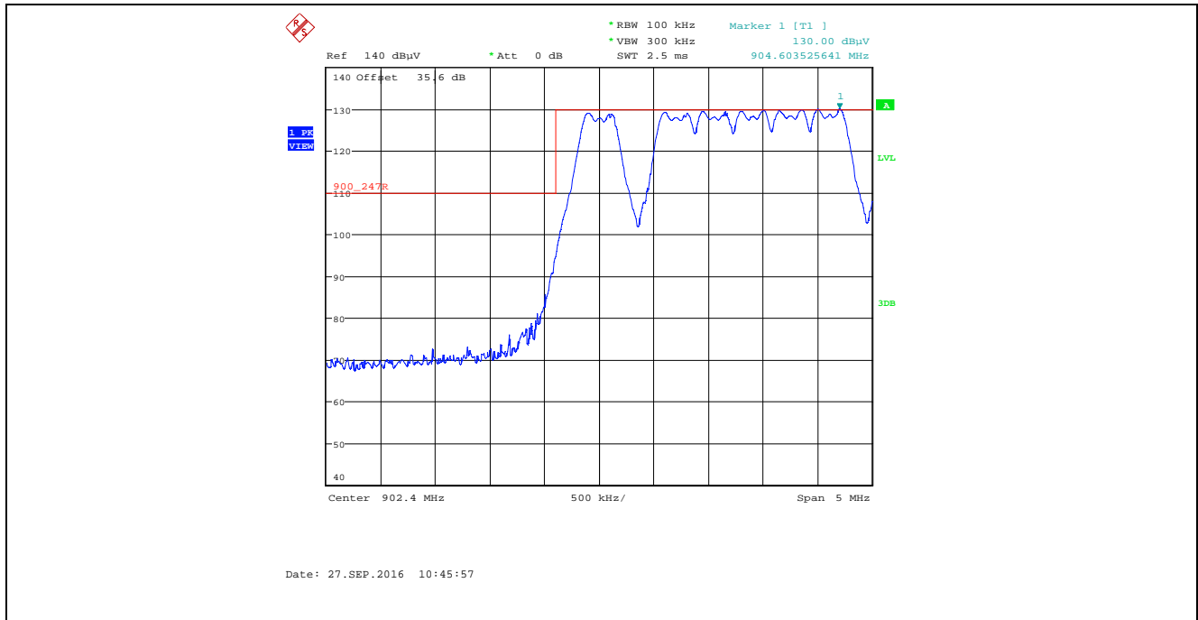
Plot 5.2.4.1.2.4. Band-Edge RF Radiated Emissions at 3 m, Vertical Polarization Pseudorandom Channel Hopping Mode, Low End of Frequency Band, Power Setting 28, Data Rate at 276480 kbps
