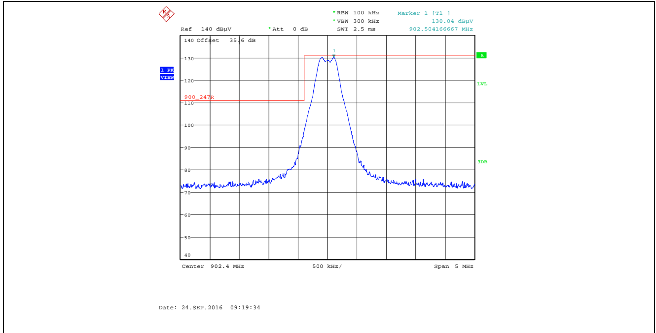
Plot 5.2.4.3.2.1. Band-Edge RF Radiated Emissions at 3 m, Horizontal Polarization Single Frequency Mode, Low End of Frequency Band, Power Setting 22, Data Rate at 276480 kbps
