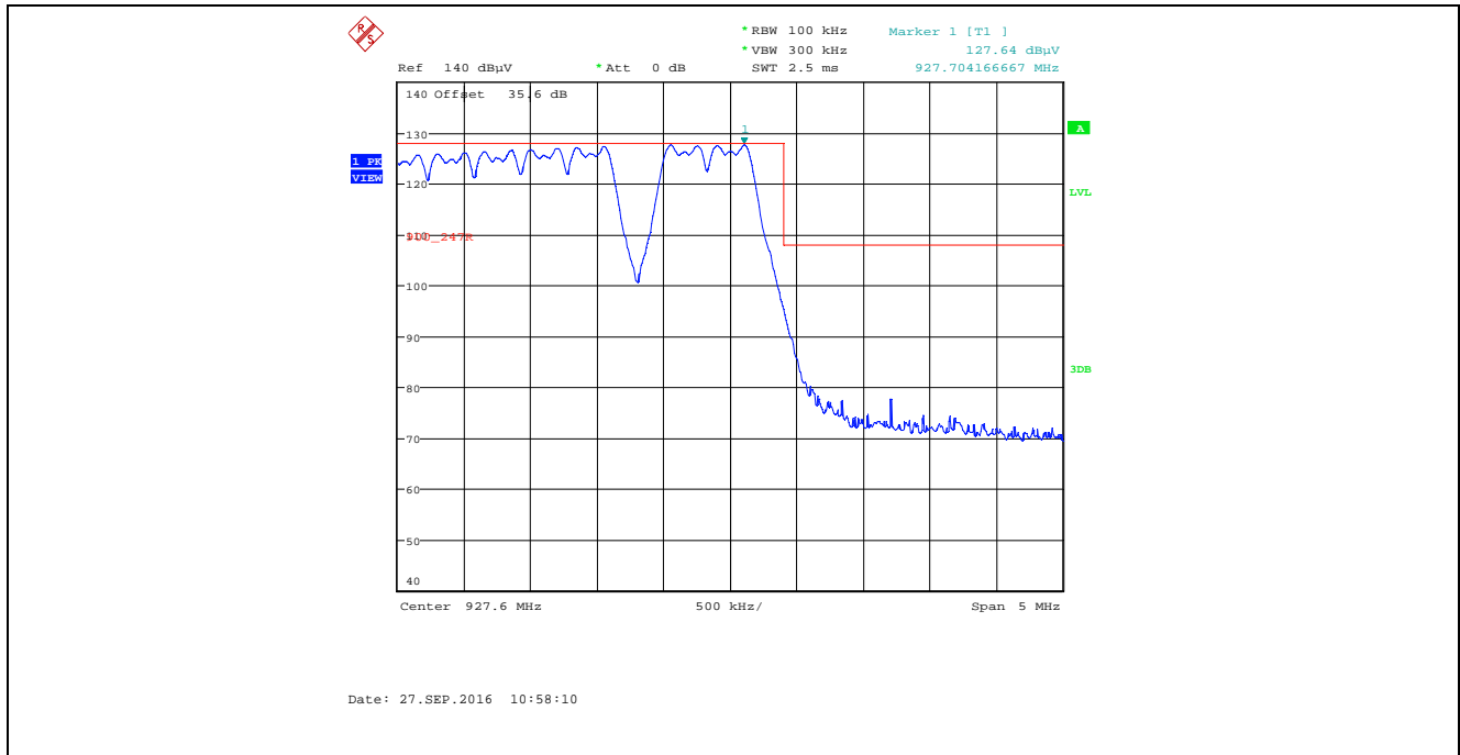
Plot 5.2.4.1.2.8. Band-Edge RF Radiated Emissions at 3 m, Vertical Polarization Pseudorandom Channel Hopping Mode, High End of Frequency Band, Power Setting 28, Data Rate at 276480 kbps
