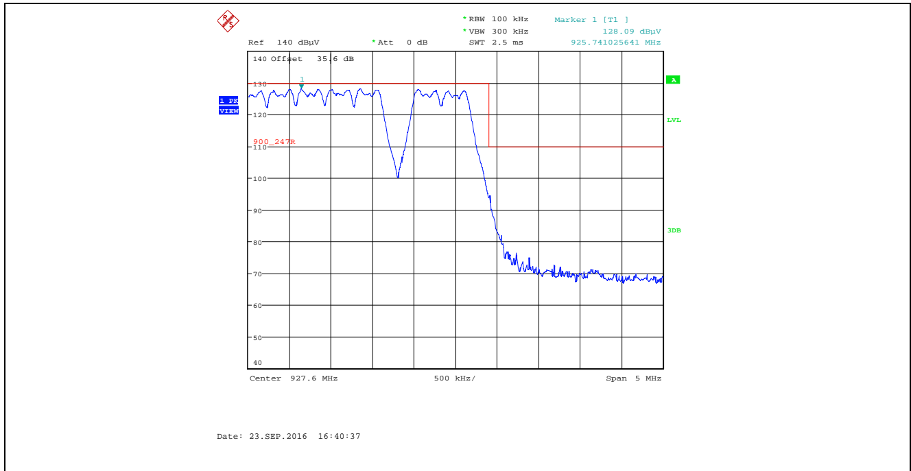
Plot 5.2.4.4.2.8. Band-Edge RF Radiated Emissions at 3 m, Vertical Polarization Pseudorandom Channel Hopping Mode, High End of Frequency Band, Power Setting 23, Data Rate at 276480 kbps
