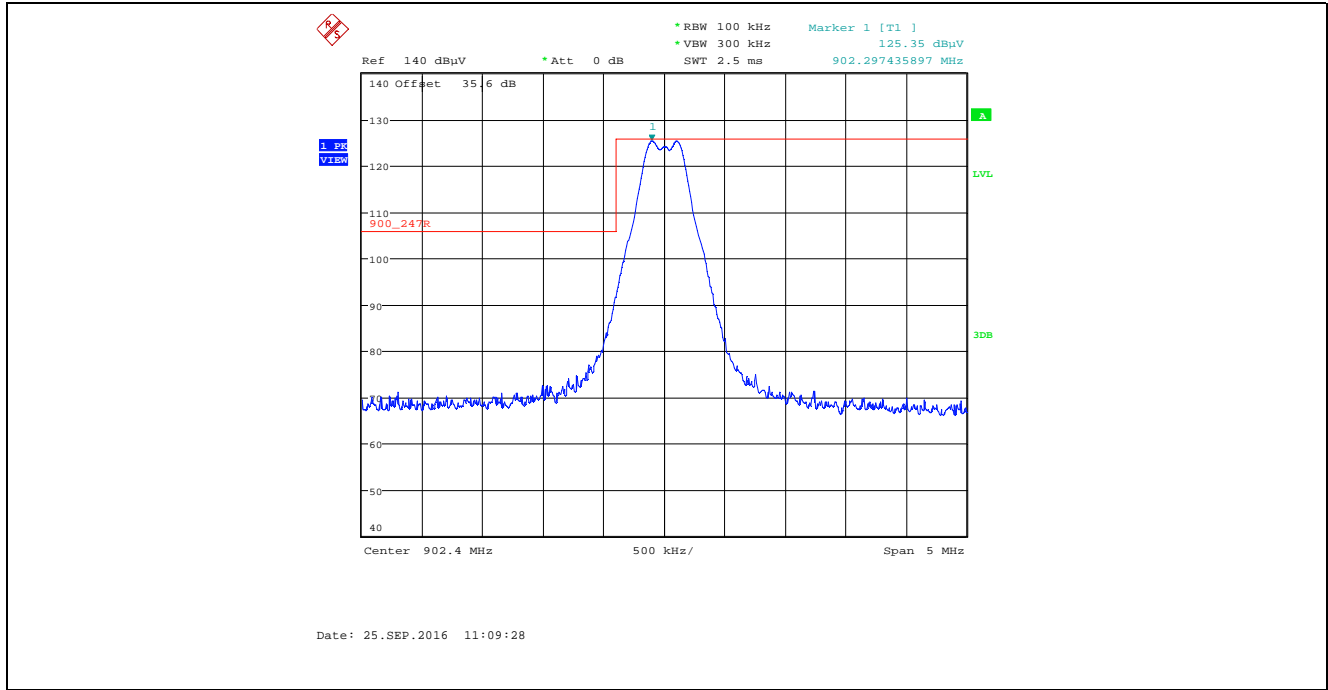
Plot 5.2.4.2.3. Band-Edge RF Radiated Emissions at 3 m, Vertical Polarization Single Frequency Mode, Low End of Frequency Band, Power Setting 28, Data Rate at 276480 kbps
