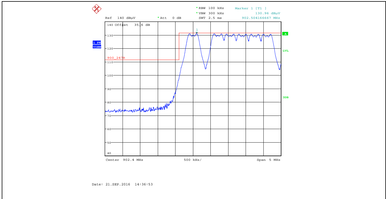
Plot 5.2.4.5.2.4. Band-Edge RF Radiated Emissions at 3 m, Vertical Polarization Pseudorandom Channel Hopping Mode, Low End of Frequency Band, Power Setting 12, Data Rate at 276480 kbps
