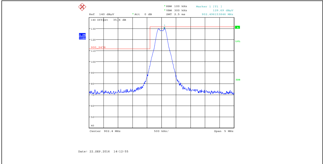
Plot 5.2.4.5.2.1. Band-Edge RF Radiated Emissions at 3 m, Horizontal Polarization Single Frequency Mode, Low End of Frequency Band, Power Setting 12, Data Rate at 276480 kbps
