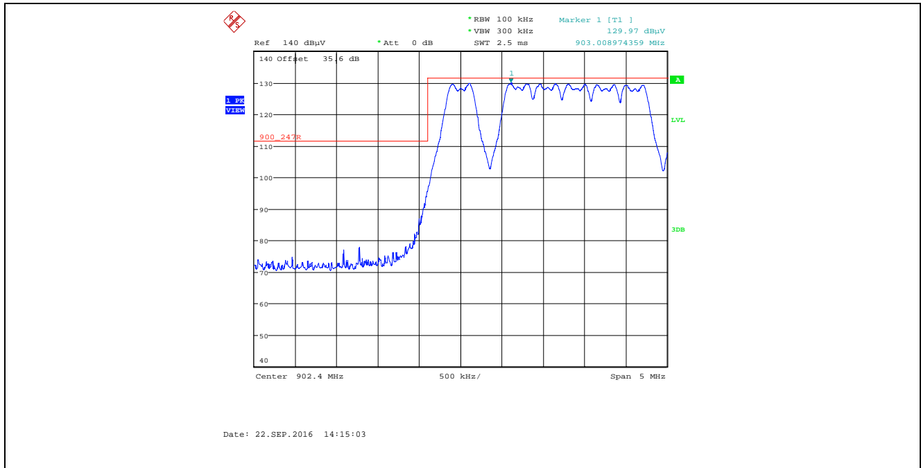
Plot 5.2.4.5.2.2. Band-Edge RF Radiated Emissions at 3 m, Horizontal Polarization Pseudorandom Channel Hopping Mode, Low End of Frequency Band, Power Setting 12, Data Rate at 276480 kbps
