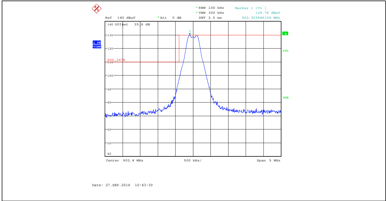
Plot 5.2.4.1.2.3. Band-Edge RF Radiated Emissions at 3 m, Vertical Polarization Single Frequency Mode, Low End of Frequency Band, Power Setting 28, Data Rate at 276480 kbps
