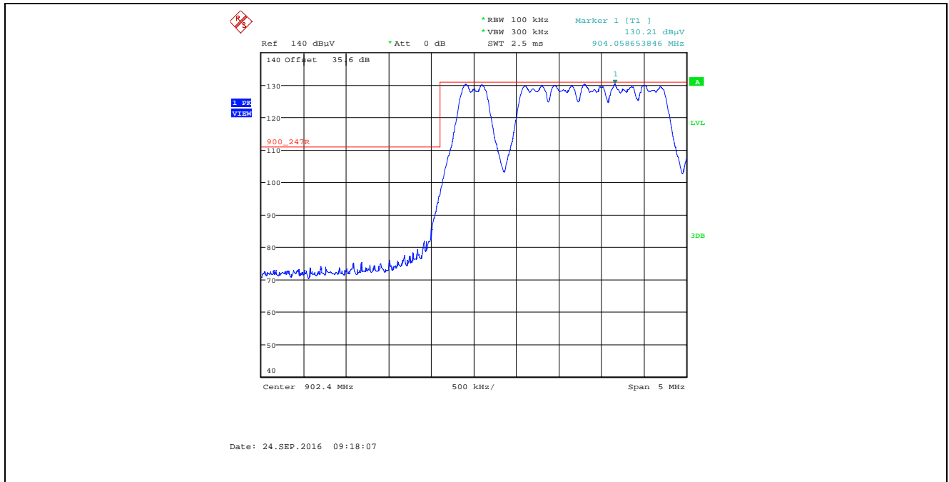
Plot 5.2.4.3.2.2. Band-Edge RF Radiated Emissions at 3 m, Horizontal Polarization Pseudorandom Channel Hopping Mode, Low End of Frequency Band, Power Setting 22, Data Rate at 276480 kbps
