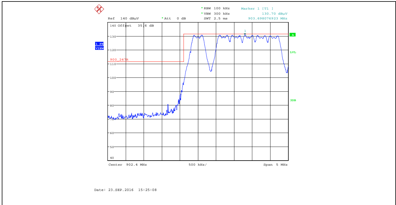
Plot 5.2.4.4.2.4. Band-Edge RF Radiated Emissions at 3 m, Vertical Polarization Pseudorandom Channel Hopping Mode, Low End of Frequency Band, Power Setting 23, Data Rate at 276480 kbps
