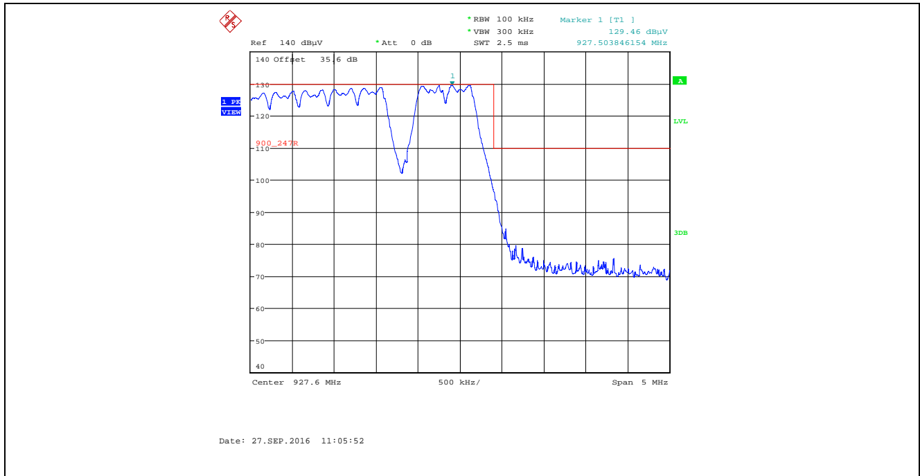
Plot 5.2.4.1.2.6. Band-Edge RF Radiated Emissions at 3 m, Horizontal Polarization Pseudorandom Channel Hopping Mode, High End of Frequency Band, Power Setting 28, Data Rate at 276480 kbps
