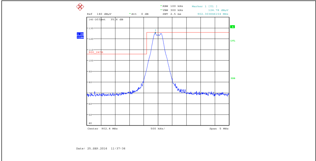
Plot 5.2.4.2.2.1. Band-Edge RF Radiated Emissions at 3 m, Horizontal Polarization Single Frequency Mode, Low End of Frequency Band, Power Setting 28, Data Rate at 276480 kbps
