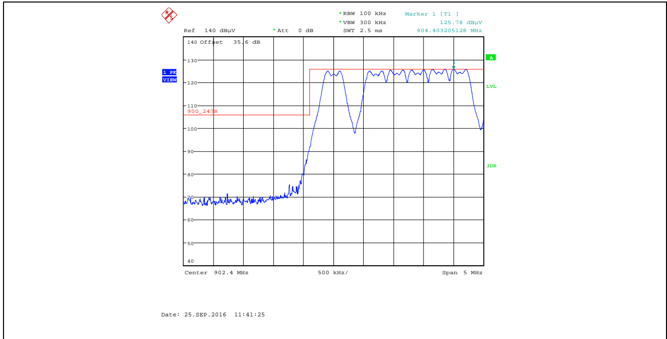
Plot 5.2.4.2.2.2. Band-Edge RF Radiated Emissions at 3 m, Horizontal Polarization Pseudorandom Channel Hopping Mode, Low End of Frequency Band, Power Setting 28, Data Rate at 276480 kbps
