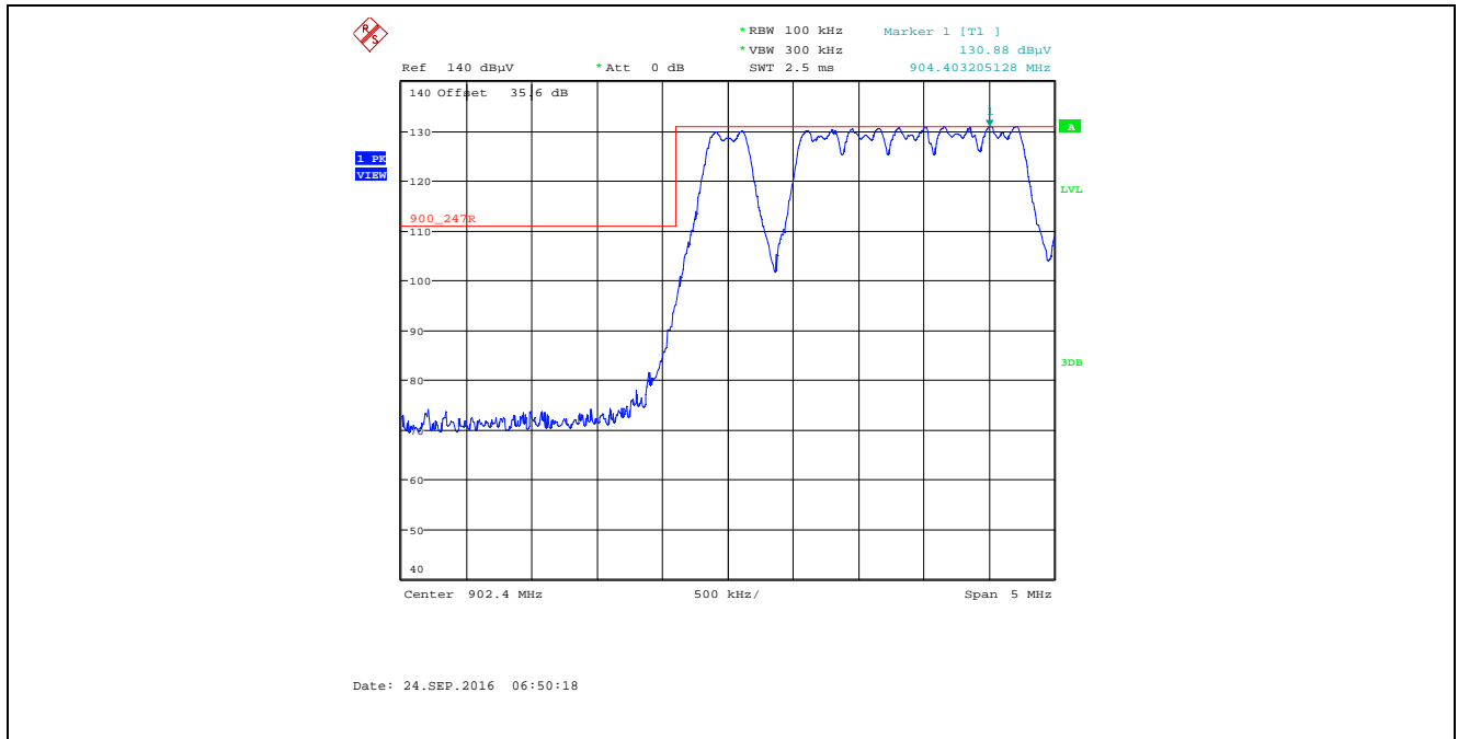
Plot 5.2.4.4.2.2. Band-Edge RF Radiated Emissions at 3 m, Horizontal Polarization Pseudorandom Channel Hopping Mode, Low End of Frequency Band, Power Setting 23, Data Rate at 276480 kbps
