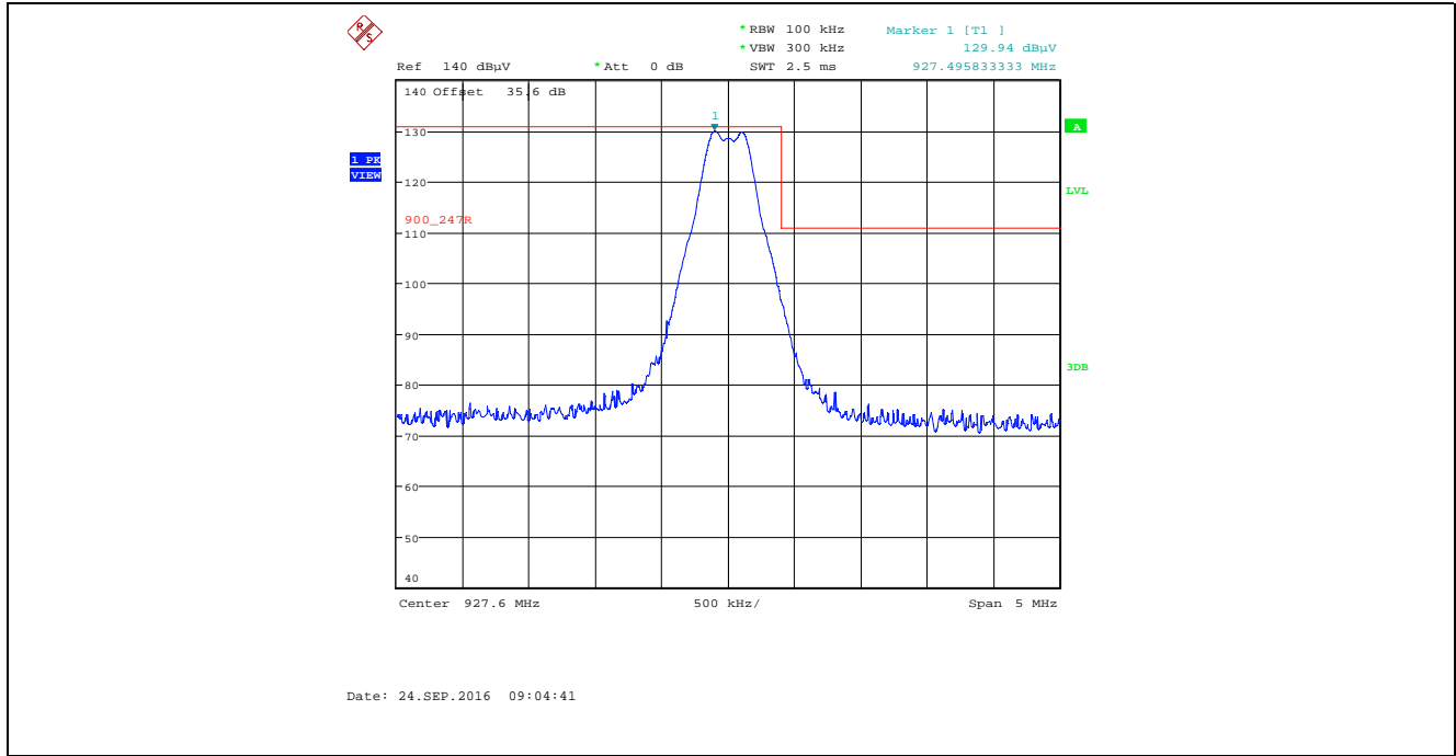
Plot 5.2.4.3.2.5. Band-Edge RF Radiated Emissions at 3 m, Horizontal Polarization Single Frequency Mode, High End of Frequency Band, Power Setting 22, Data Rate at 276480 kbps
