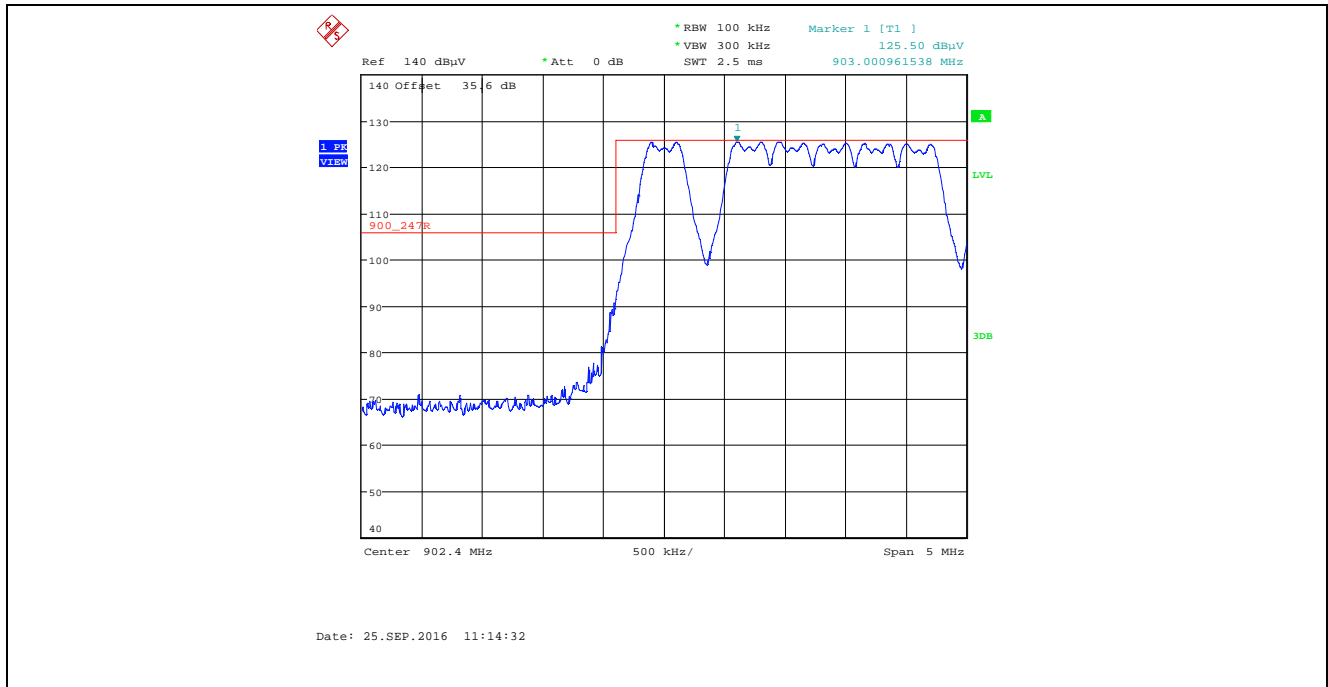
Plot 5.2.4.2.4. Band-Edge RF Radiated Emissions at 3 m, Vertical Polarization Pseudorandom Channel Hopping Mode, Low End of Frequency Band, Power Setting 28, Data Rate at 276480 kbps
