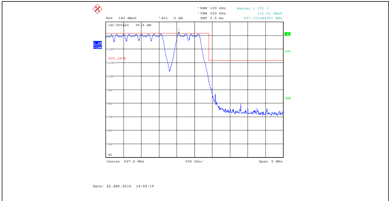
Plot 5.2.4.5.2.6. Band-Edge RF Radiated Emissions at 3 m, Horizontal Polarization Pseudorandom Channel Hopping Mode, High End of Frequency Band, Power Setting 12, Data Rate at 276480 kbps
