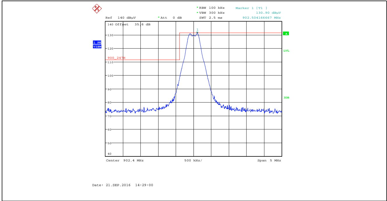
Plot 5.2.4.5.2.3. Band-Edge RF Radiated Emissions at 3 m, Vertical Polarization Single Frequency Mode, Low End of Frequency Band, Power Setting 12, Data Rate at 276480 kbps
