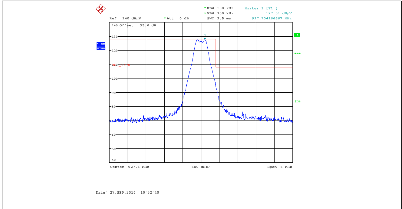
Plot 5.2.4.1.2.7. Band-Edge RF Radiated Emissions at 3 m, Vertical Polarization Single Frequency Mode, High of Frequency Band, Power Setting 28, Data Rate at 276480 kbps
