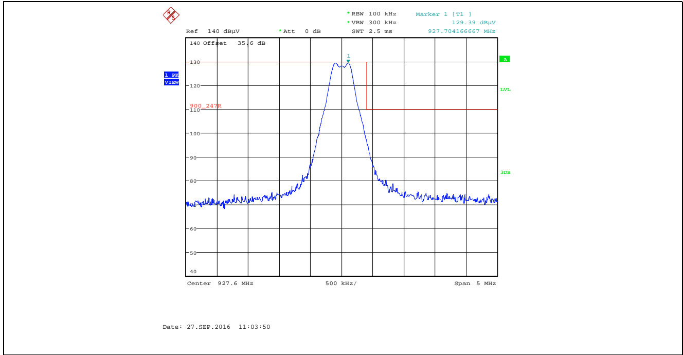
Plot 5.2.4.1.2.5. Band-Edge RF Radiated Emissions at 3 m, Horizontal Polarization Single Frequency Mode, High End of Frequency Band, Power Setting 28, Data Rate at 276480 kbps
