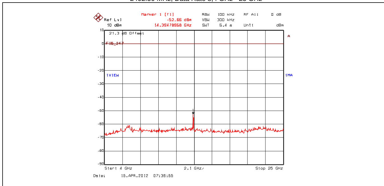
Plot 5.4.4.2.2. Conducted Spurious Emissions - Non Restricted Frequency Bands 2402.50 MHz, Data Rate 8,4 GHz - 25 GHz
