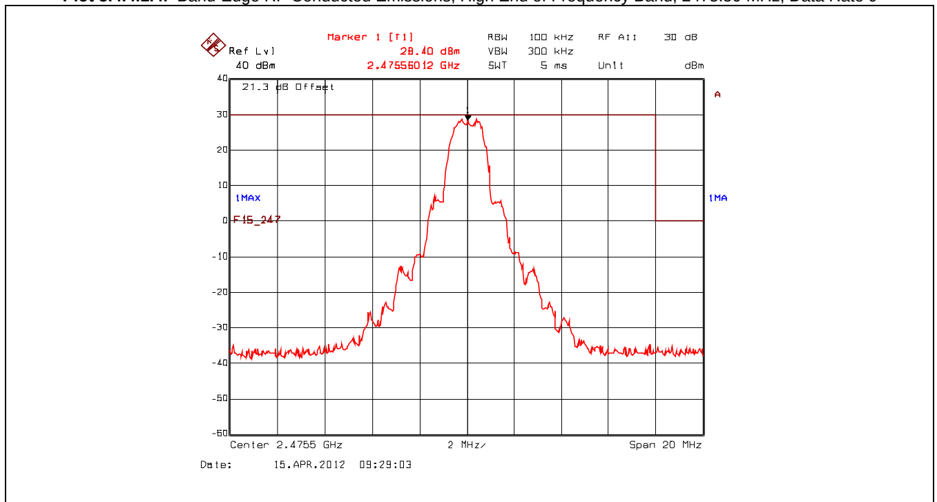
Plot 5.4.4.1.4. Band-Edge RF Conducted Emissions, High End of Frequency Band, 2475.50 MHz, Data Rate 9
