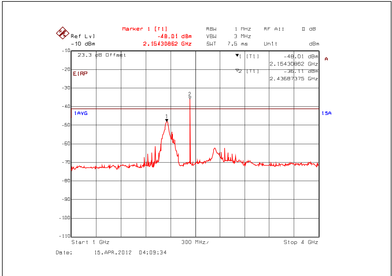
Plot 5.4.4.9. Conducted Spurious Emissions – Restricted Bands 2439.25 MHz, 1 GHz - 4 GHz, Trace Average with Band (Notch) Reject Filter
