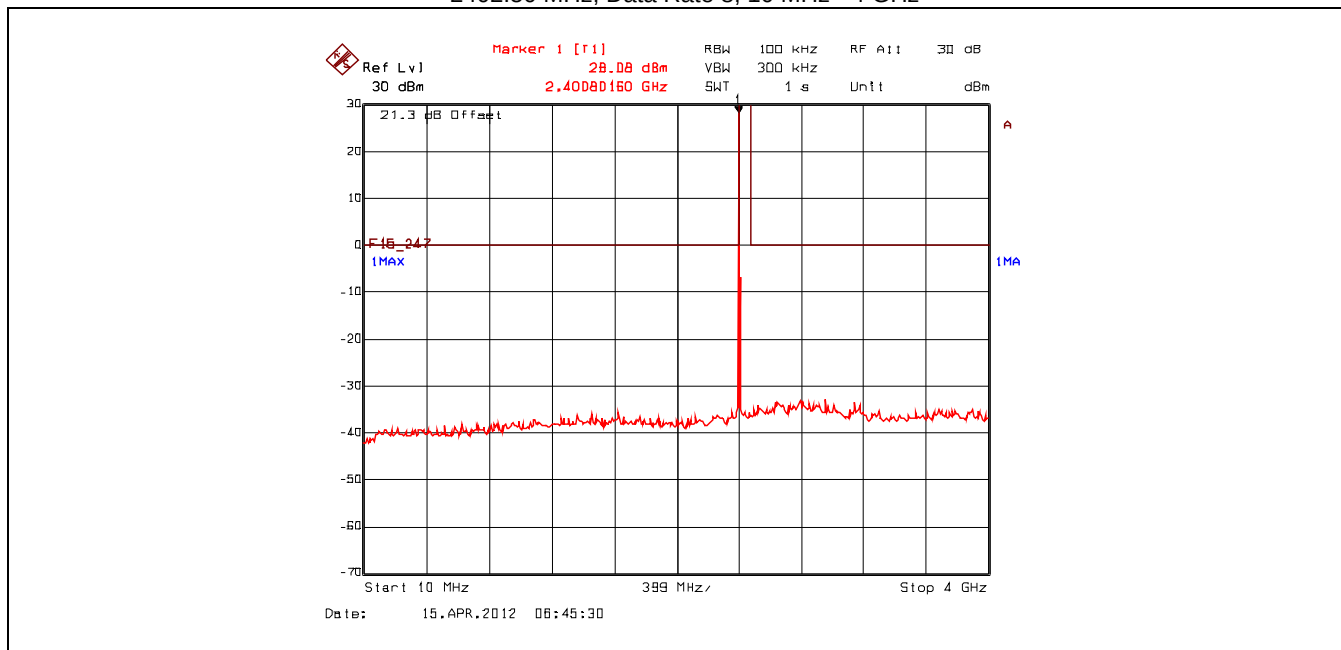
Plot 5.4.4.2.1. Conducted Spurious Emissions - Non Restricted Frequency Bands 2402.50 MHz, Data Rate 8, 10 MHz - 4 GHz
