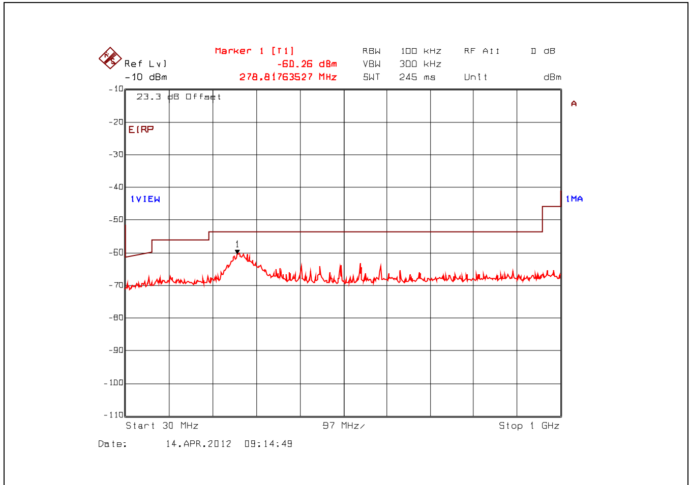
Plot 5.4.4.8. Conducted Spurious Emissions – Restricted Bands 2439.25 MHz, 30 MHz - 1 GHz, Peak Detector with Band (Notch) Reject Filter
