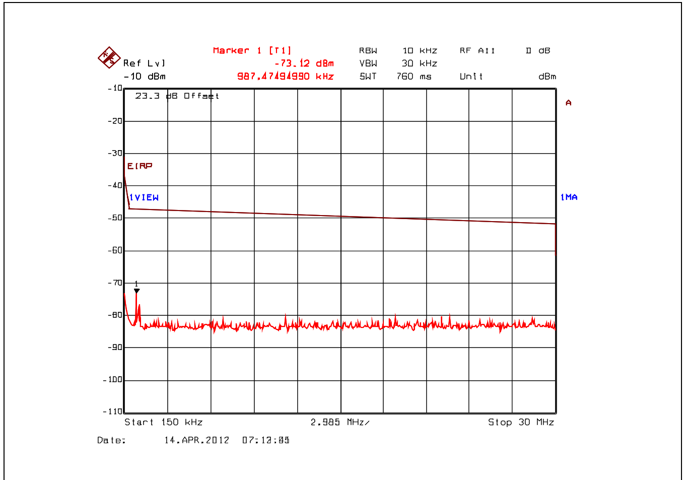
Plot 5.4.4.2. Conducted Spurious Emissions – Restricted Bands 2402.50 MHz, 150 kHz - 30 MHz, Peak Detector
