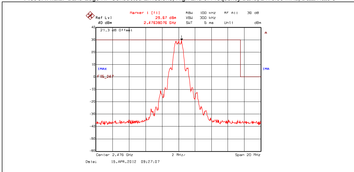
Plot 5.4.4.1.2. Band-Edge RF Conducted Emissions, High End of Frequency Band, 2476.00 MHz, Data Rate 8
