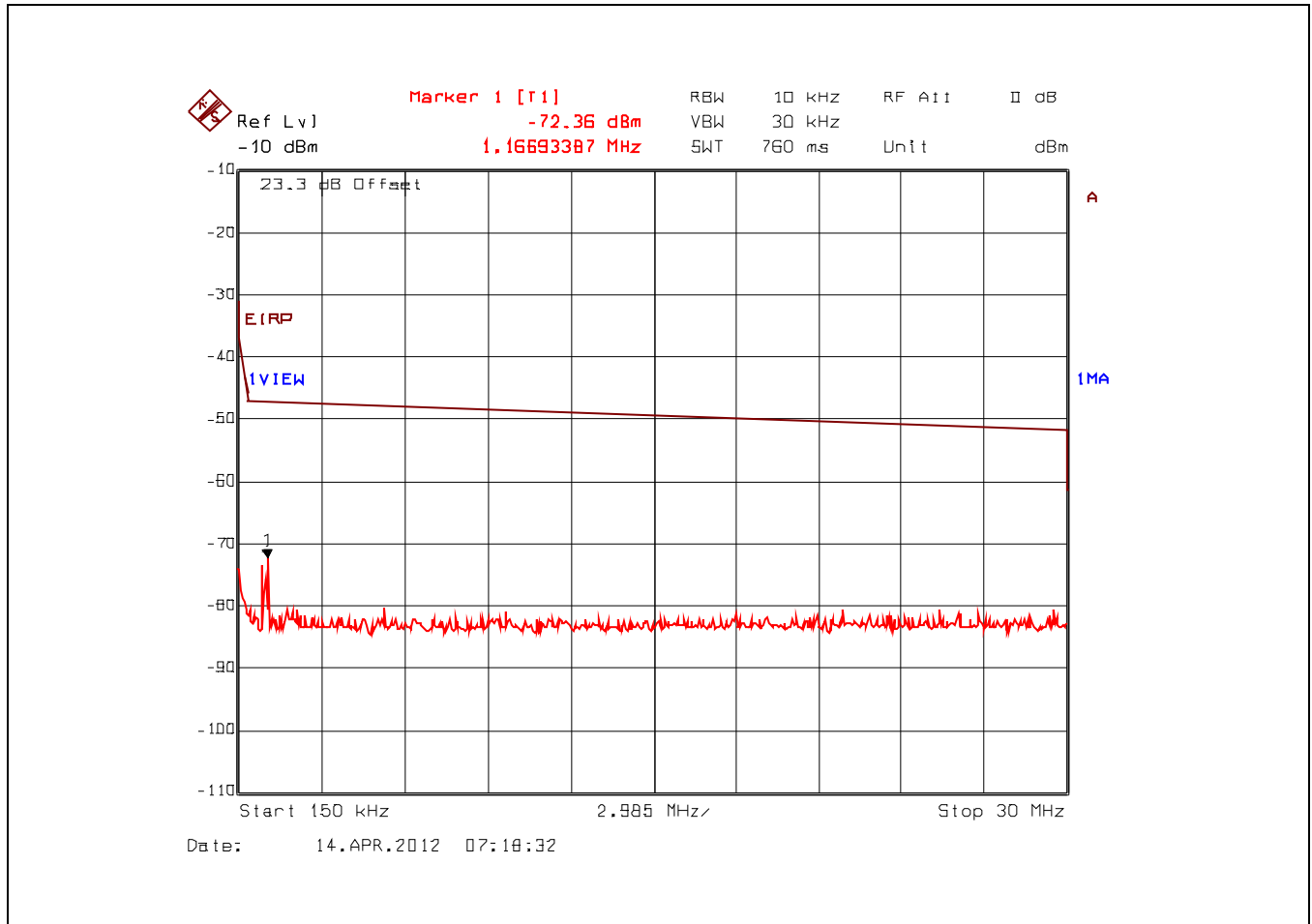
Plot 5.4.4.7. Conducted Spurious Emissions – Restricted Bands 2439.25 MHz, 150 kHz - 30 MHz, Peak Detector
