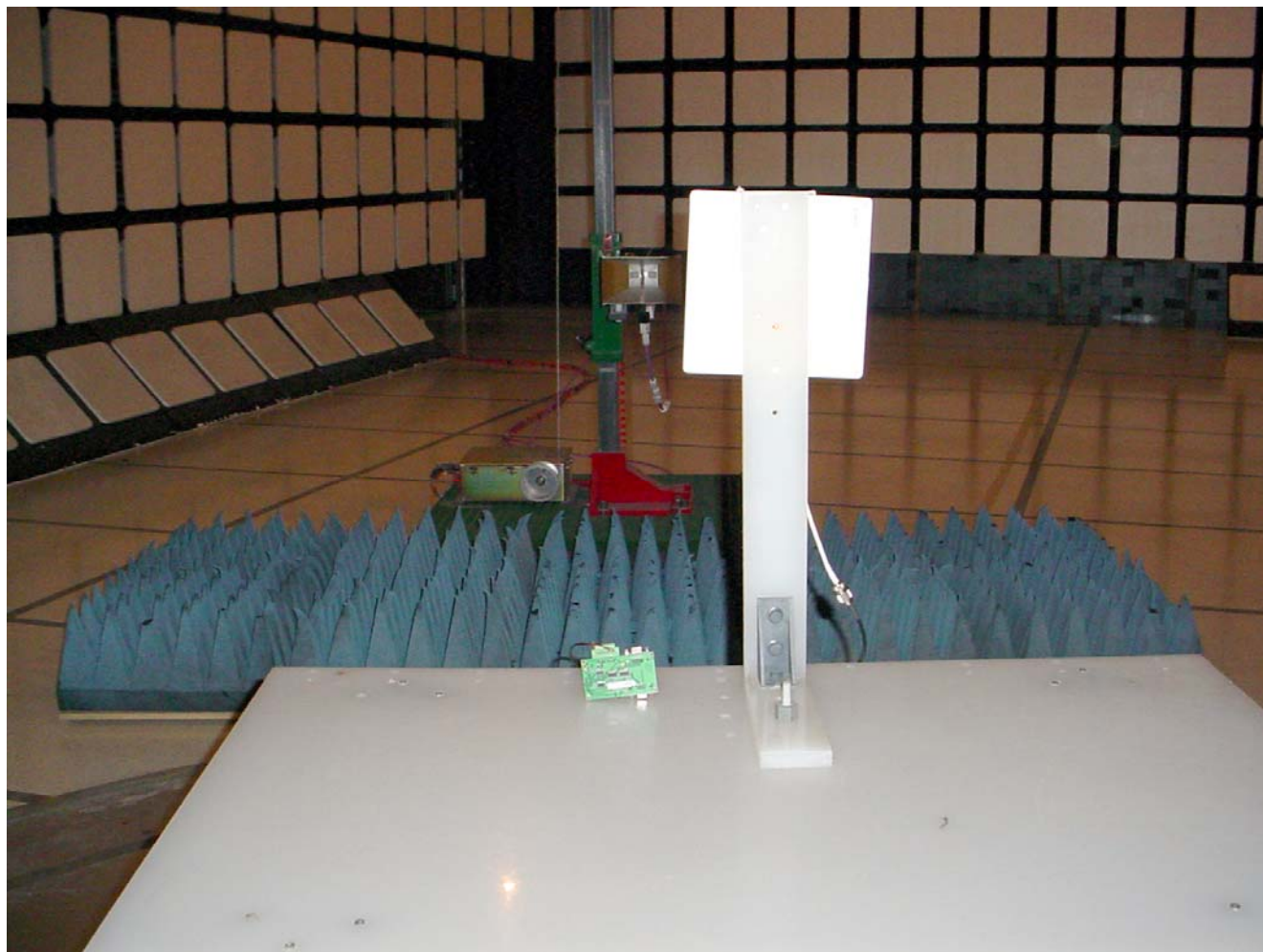
Radiated Emissions @ 3 m EUT with 14 dBi Patch Antenna
