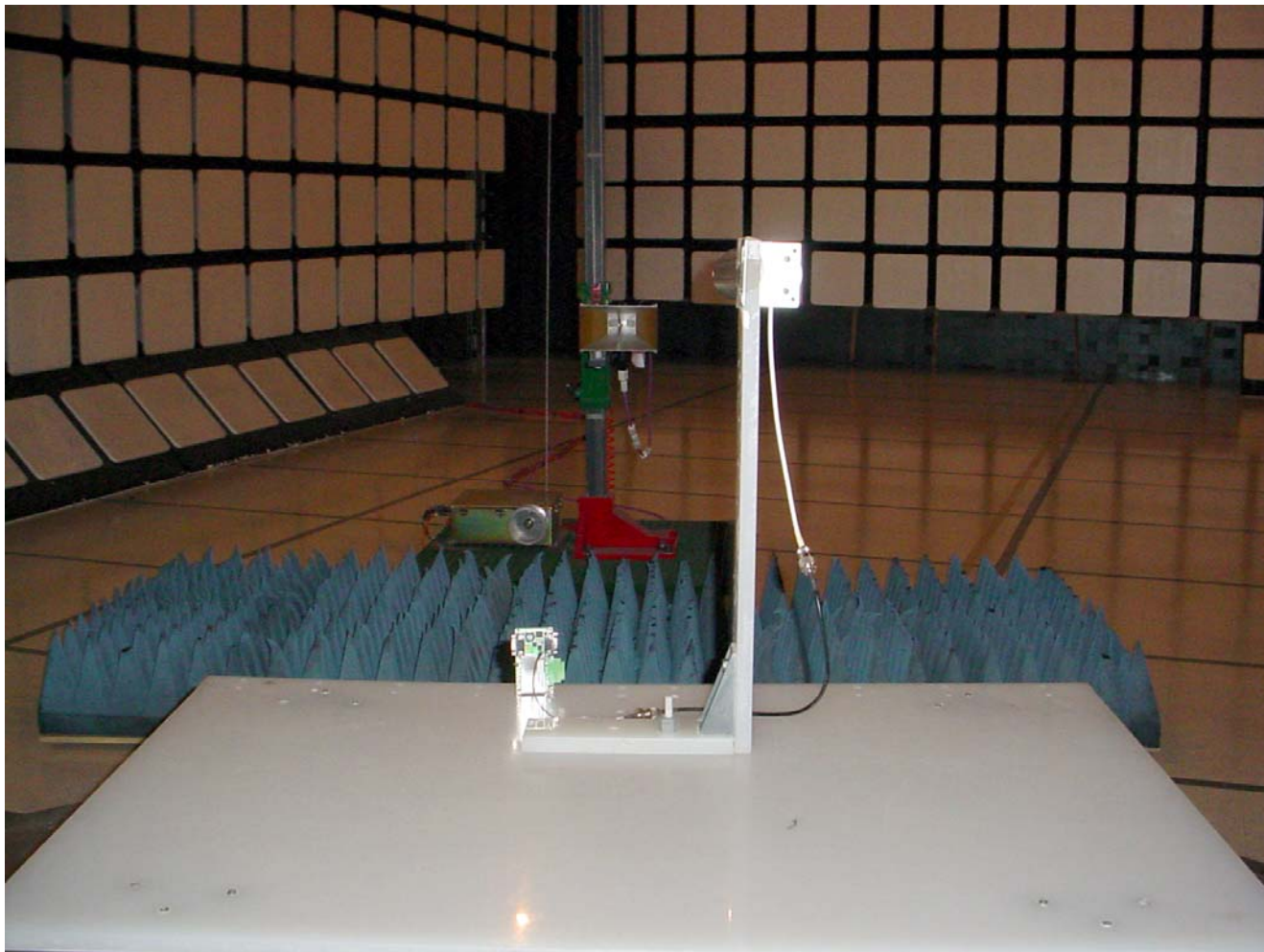
Radiated Emissions @ 3 m EUT with 14.5 dBi Yagi Antenna
