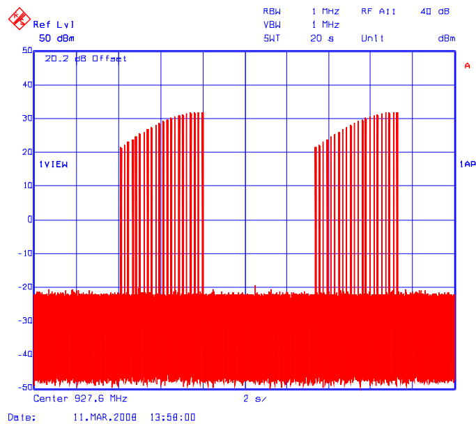
Plot 6.7.5.18(i) Time of Occupancy Test Frequency: 927.6 MHz (at low data rate)
