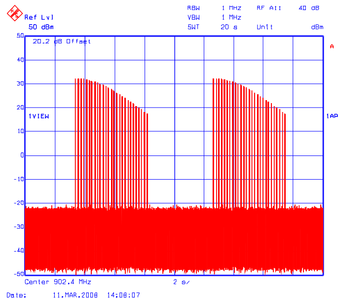
Plot 6.7.5.14(i) Time of Occupancy Test Frequency: 902.4 MHz (at low data rate)
