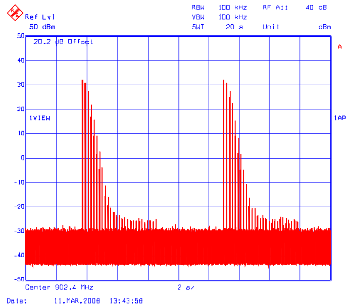
Plot 6.7.5.14(ii) Time of Occupancy (at 100 kHz RBW/VBW to resolve the actual hopping channels) Test Frequency: 902.4 MHz (at low data rate)
