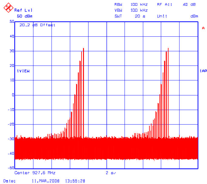
Plot 6.7.5.18(ii) Time of Occupancy (at 100 kHz RBW/VBW to resolve the actual hopping channels) Test Frequency: 927.6 MHz (at low data rate)
