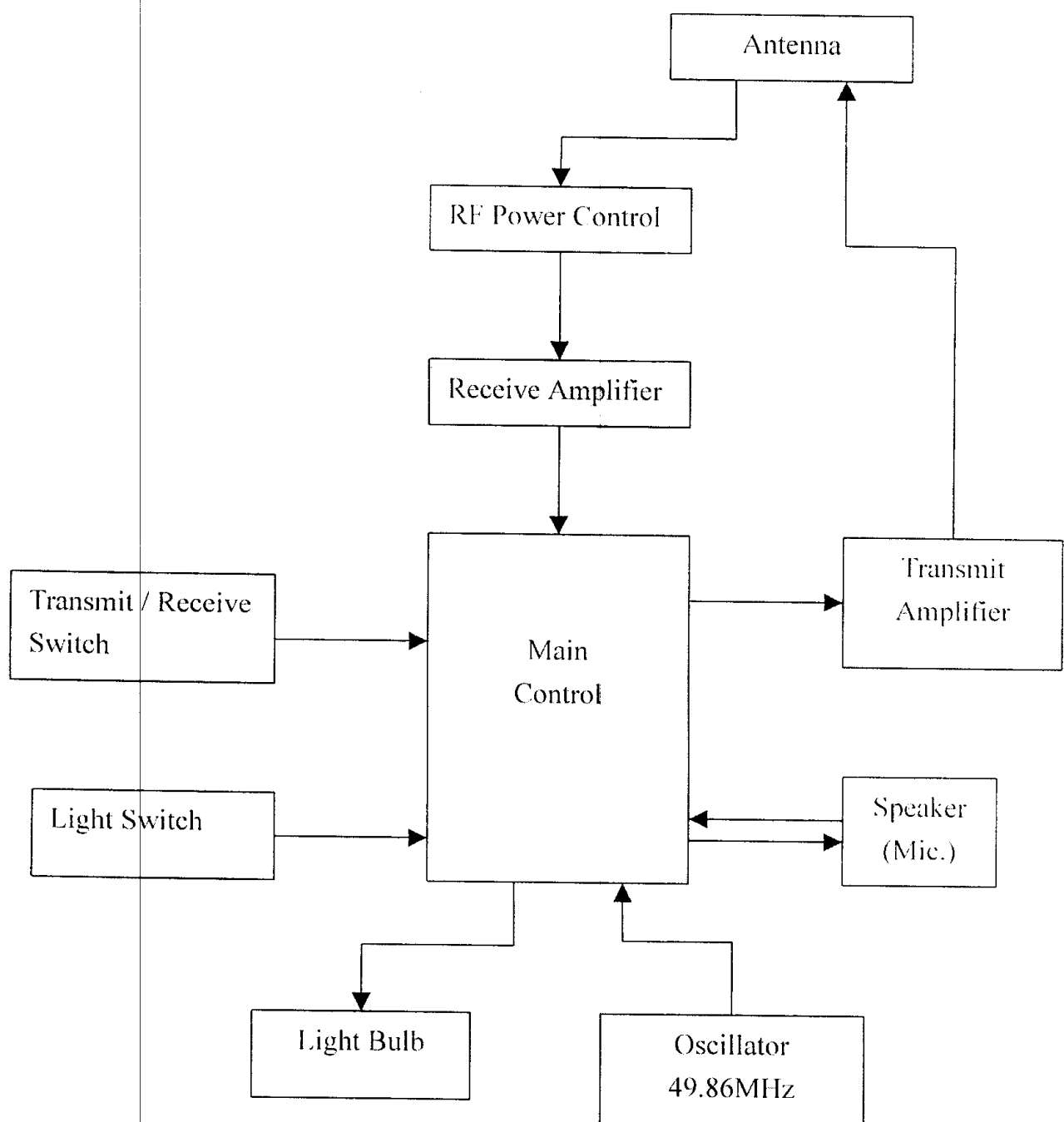
Block Diagram of Rescue Squad Walkie Talkies
