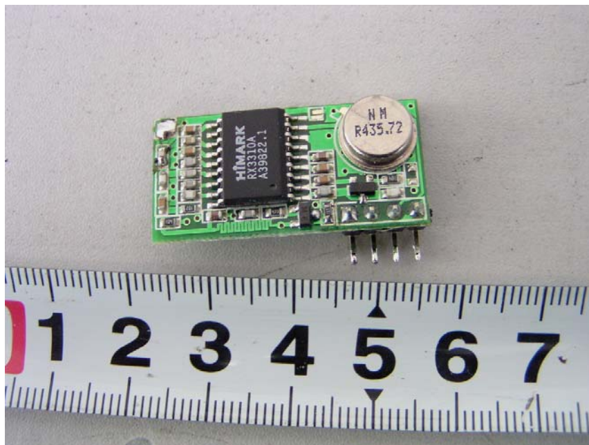
EUT – Radio Module Top View
