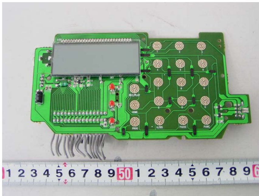
EUT – Keyboard Top View
