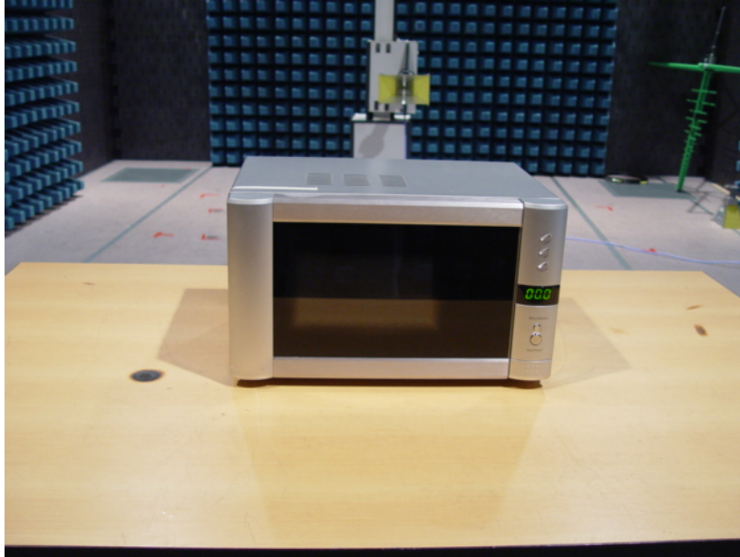
Test Setup Photographs:3 (Above 1GHz)
