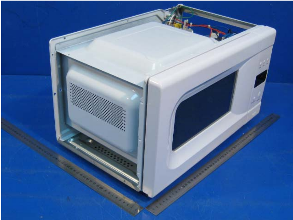
Photo 9 Inside of EUT (WP700D-S20)
