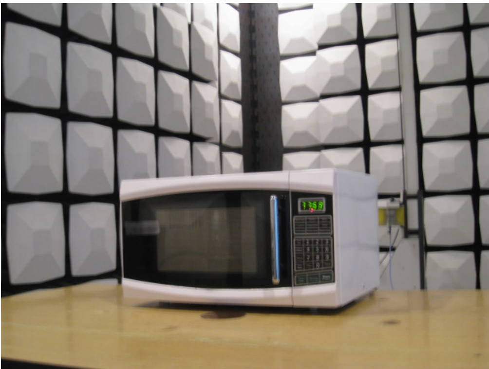
Photo 6 Radiated Disturbance Test (above 1GHz) (MEW621-A1)
